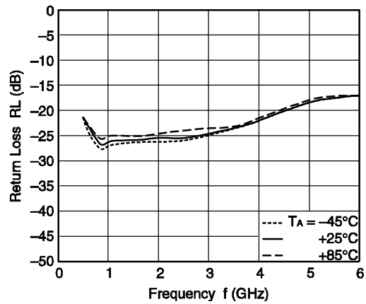
RF1/RF2 RETURN LOSS vs. FREQUENCY
