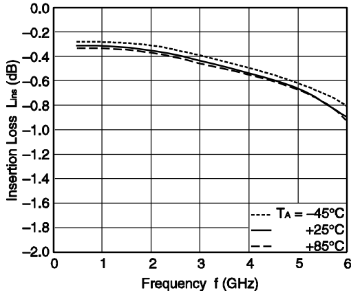
RFC-RF1/RF2 INSERTION LOSS vs. FREQUENCY
