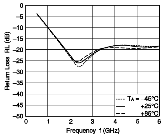
RF1/RF2 RETURN LOSS vs. FREQUENCY
