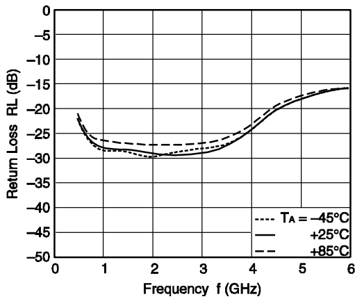
RFC RETURN LOSS vs. FREQUENCY
