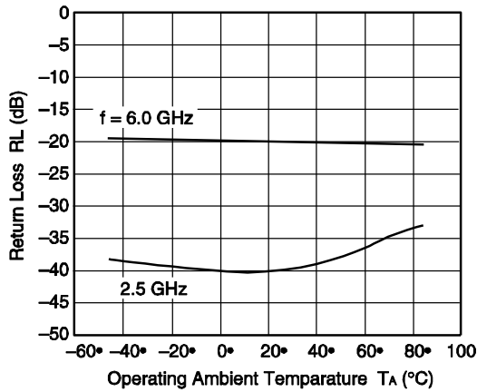
RFC RETURN LOSS vs. OPERATING AMBIENT TEMPERATURE
