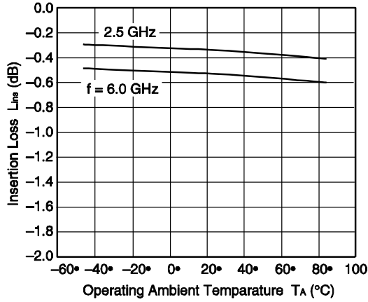
RFC-RF1/RF2 INSERTION LOSS vs. OPERATING AMBIENT TEMPERATURE
