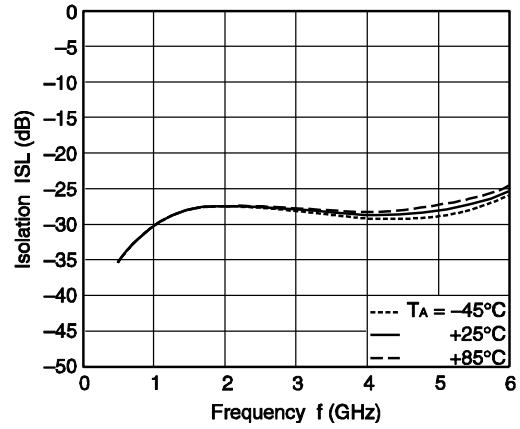
RFC-RF1/RF2 ISOLATION vs. FREQUENCY
