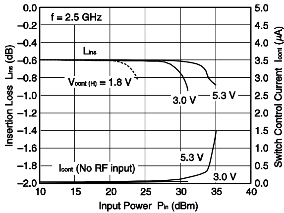
RFC-RF1/RF2 INSERTION LOSS, I_{cont} vs. INPUT POWER
