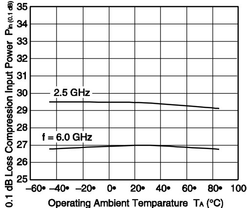
RFC-RF1/RF2 P_{in(0.1\text{ dB})} vs. OPERATING AMBIENT TEMPERATURE
