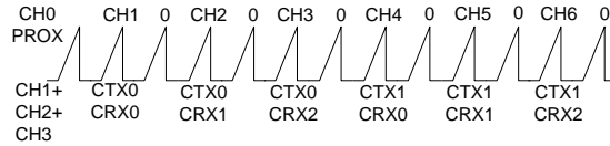
Figure 8.1 IQS156 Charge transfer.
