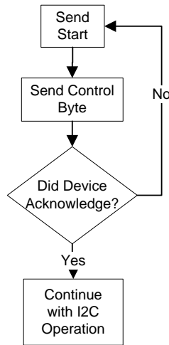
Figure 9.2 ACK Polling.
