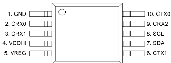
Figure 1.1 IQS156 Pin-outs.
