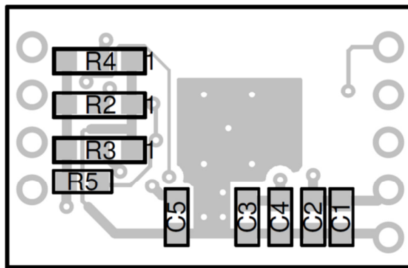
Figure 5.1.2 Bottom layer component placement
