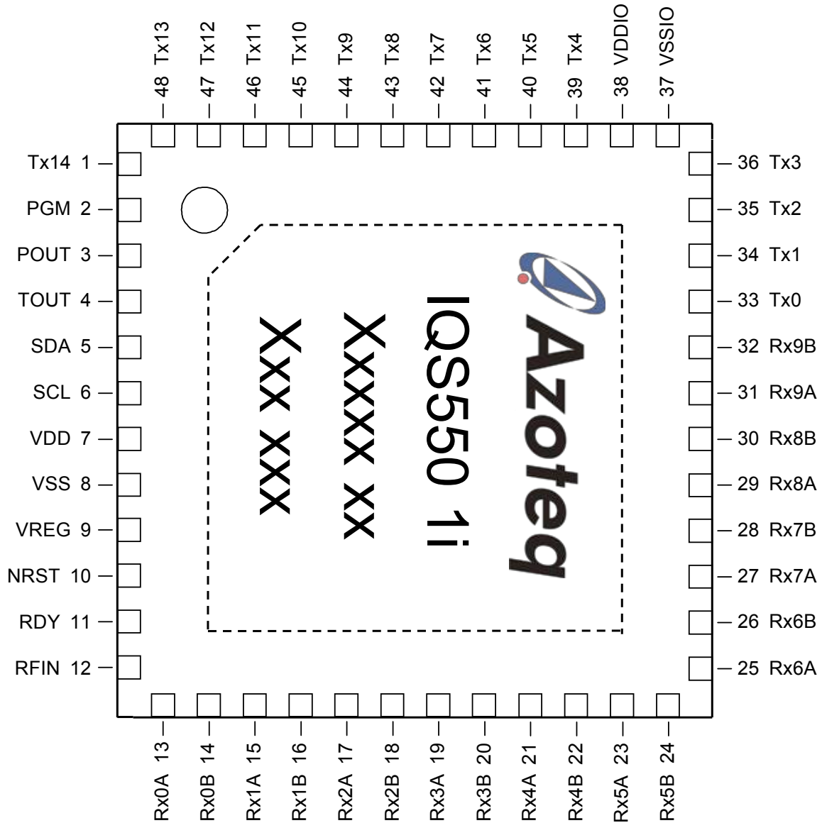
Figure 2.1 QFN Top View
