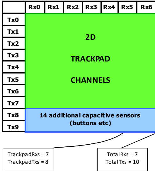
Figure 4.1 Defining trackpad area
