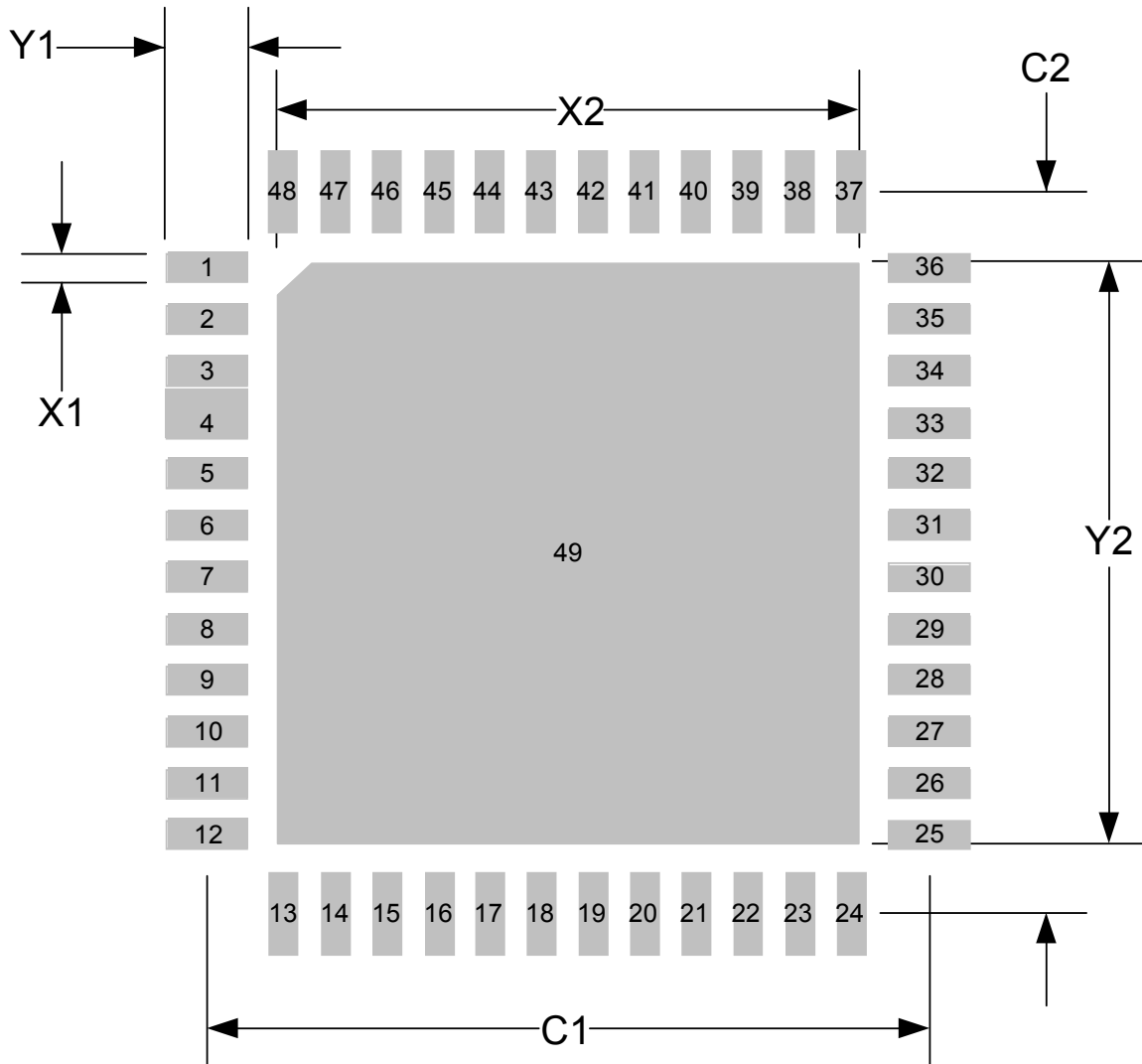
Figure 8.2 QFN(7x7)-48 Footprint
