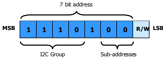
Figure 5.1 I 2 C Control Byte
