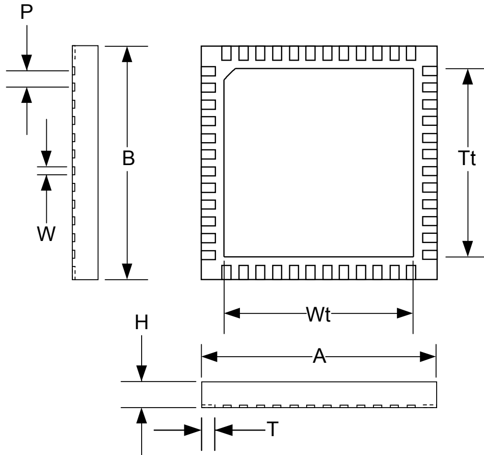
Figure 8.1 QFN(7x7)-48 Package
