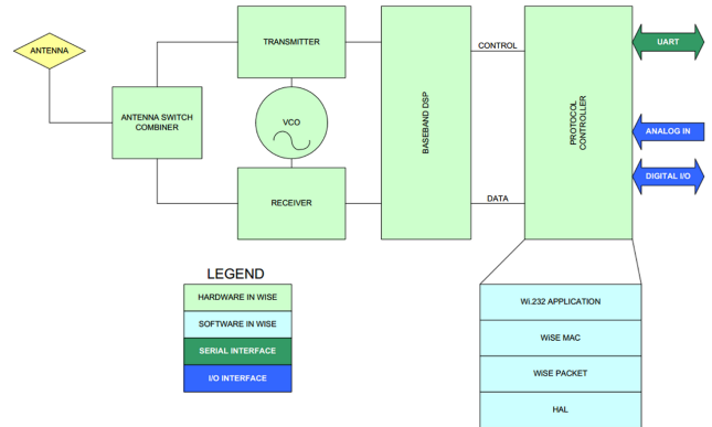
Figure 6: Module Overview
