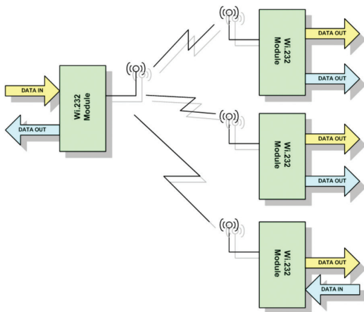
Figure 8: Wi.232DTS Networking Concept
