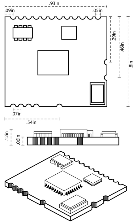
Figure 13: Module Mechanical Drawings
