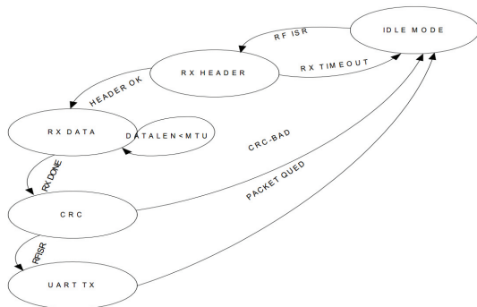
Figure 9: RX State Machine
