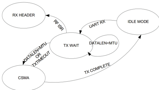
Figure 10: TX State Machine
