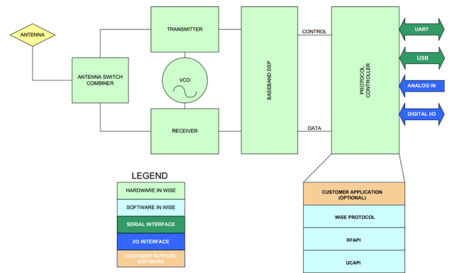
Figure 7: WISE Block Diagram
