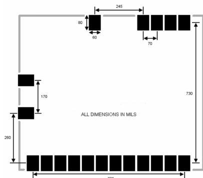
Figure 14: DTS Series Module Suggested Footprint
