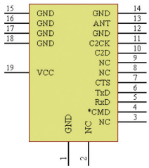
Figure 11: Pinout Diagram
