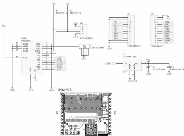
Figure 15: Evaluation Module Circuit
