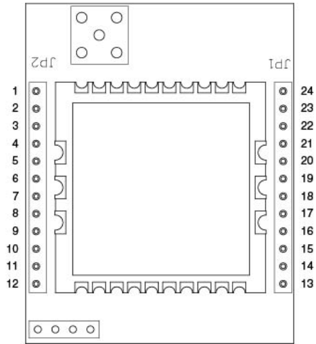
Figure 3: Pin Assignments
