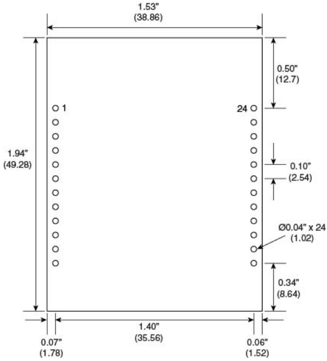
Figure 5: PCB Footprint
