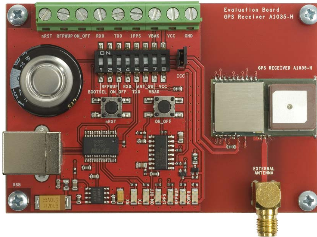
Figure 11: Board overview
