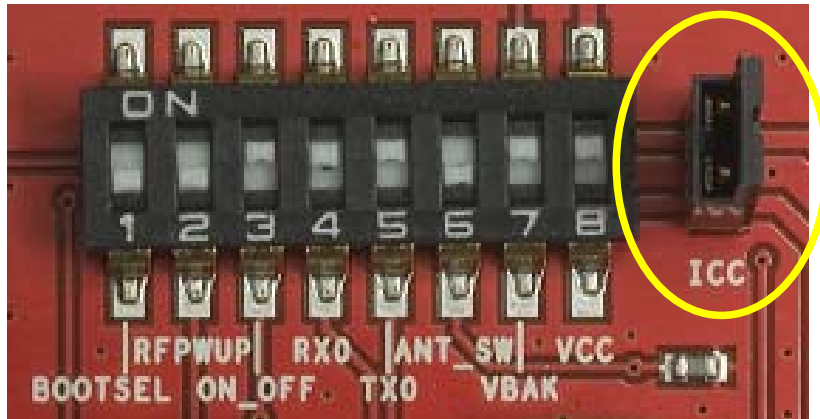
Figure 10: ICC jumper
