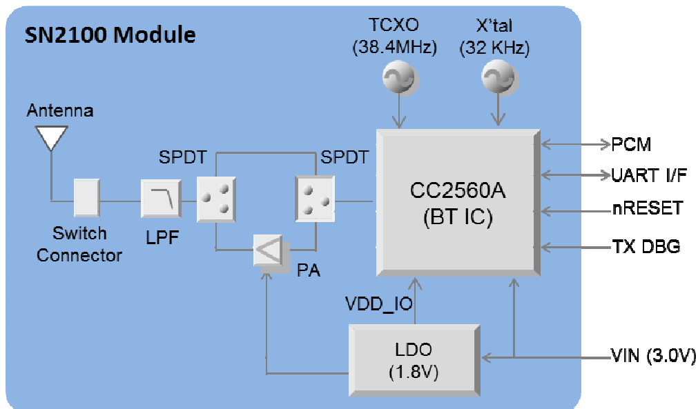
Figure 1 SN2100 Module Block Diagram
