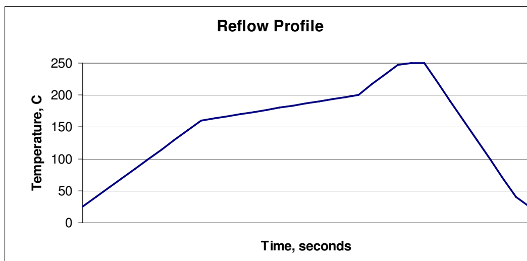
Figure 10 Reflow Profile Pattern
