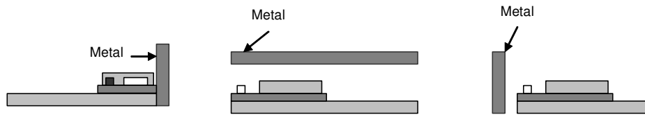
Figure 9 Locations Not Recommended in xy-plane
