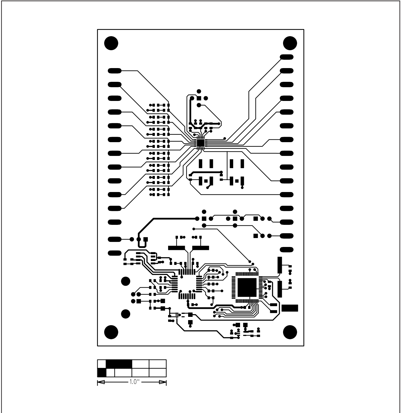
Figure 5. MAX7312 EV Kit PCB Layout—Component Side
