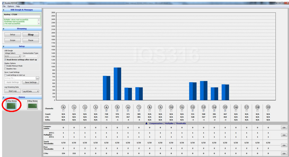
Figure 5.2 Start-up Screen for the IQS316 GUI
