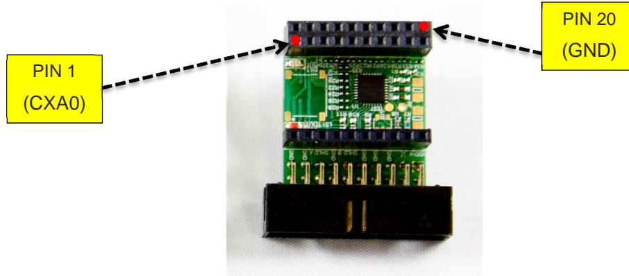
Figure 6.2 IQS316 Controller Module
