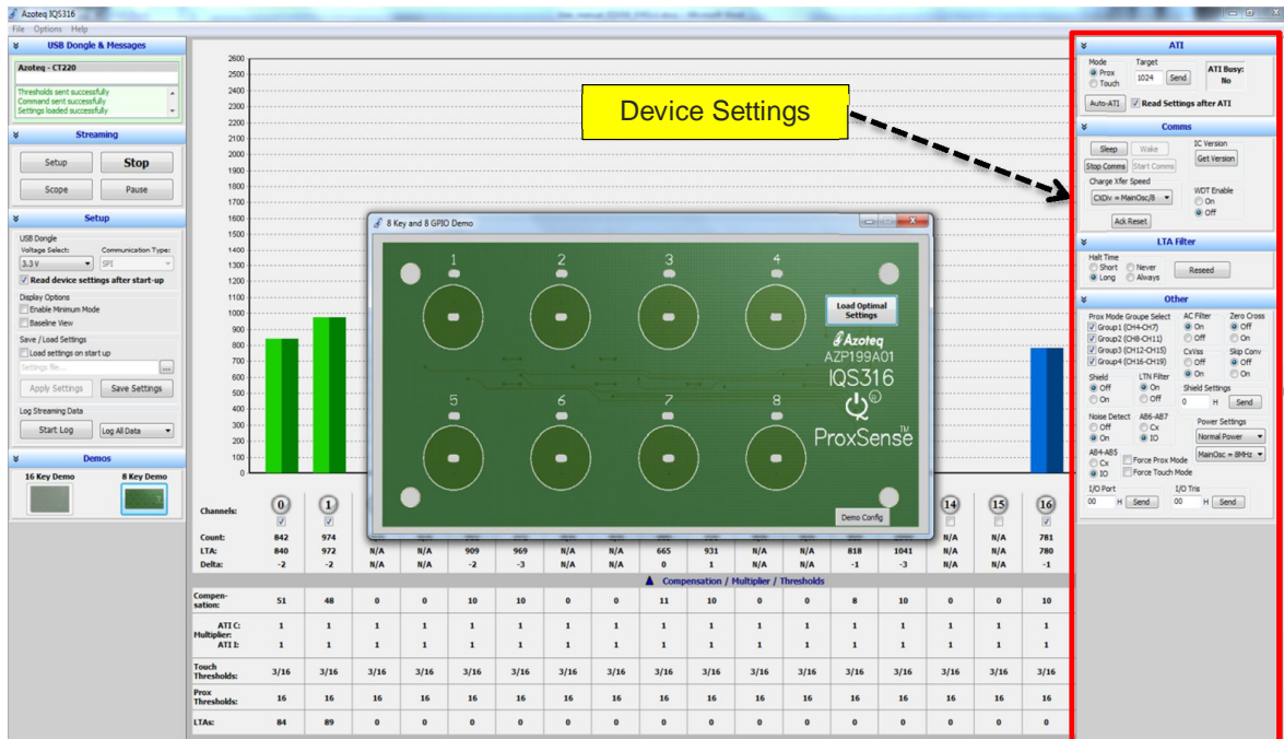
Figure 5.7 Device settings menu
