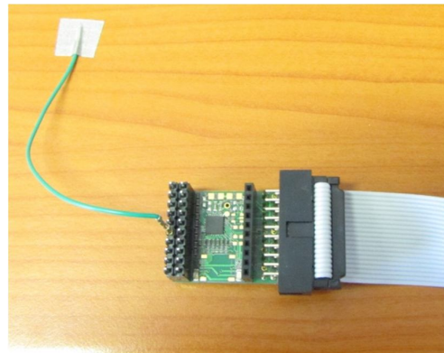
Figure 6.3 Simple touchkey connected to IQS316 Controller
