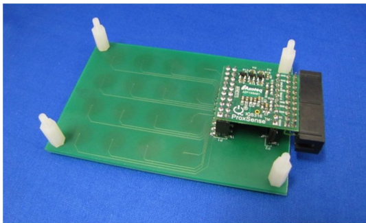
Figure 3.2 16-Key Touchpanel with controller board attached
