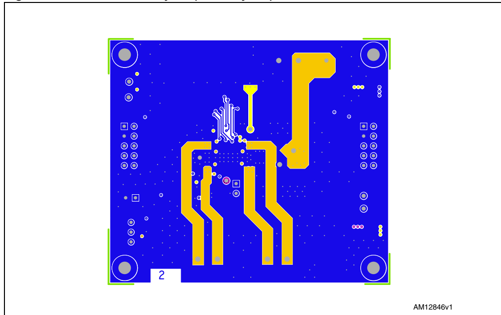
Figure 5. EVAL6470H - layout (inner layer 2)
