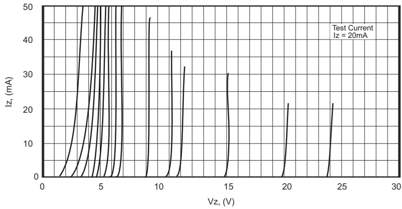
Fig.2 - Breakdown Characteristics
