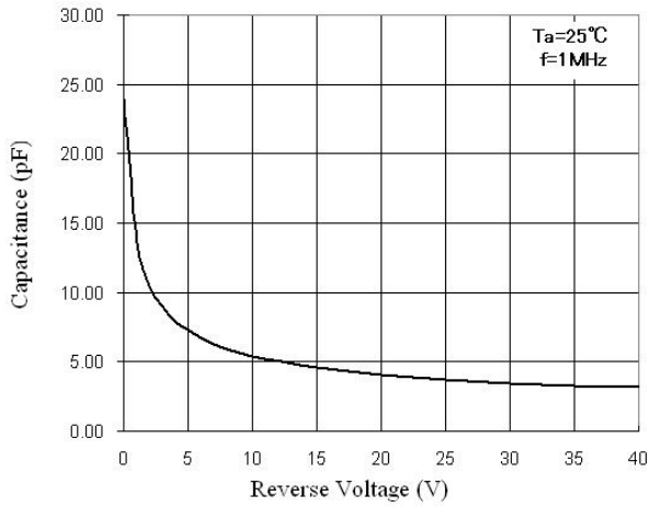
Fig.1 Total Capacitance
