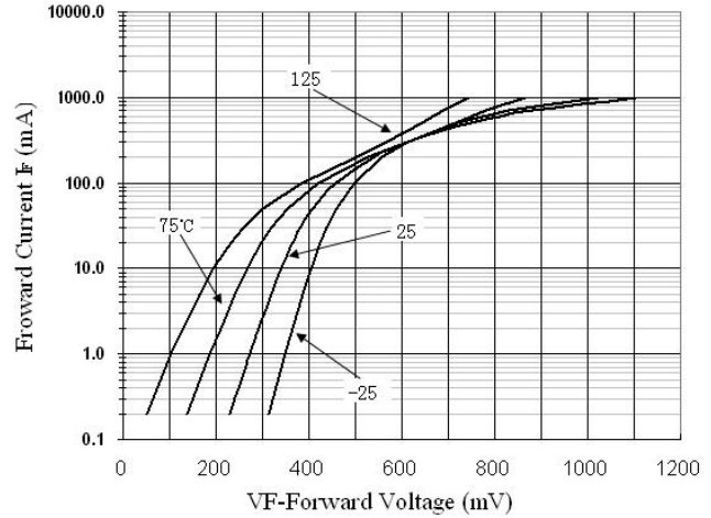
Fig.2 Forward Voltage vs Ambient
