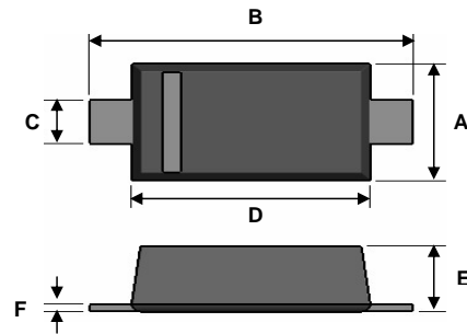
SOD-523F
