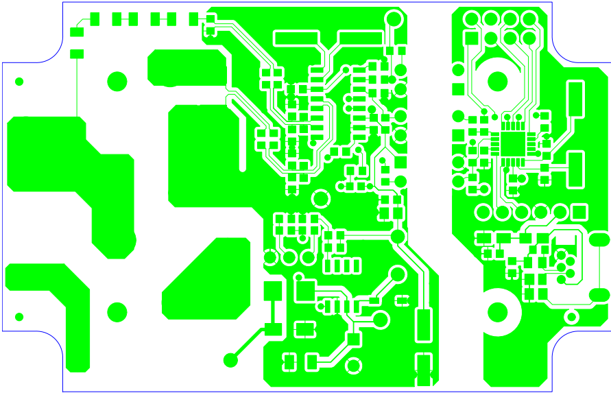
Figure 43. Top Routing
