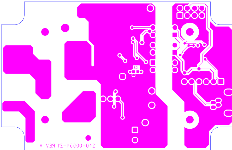
Figure 44. Bottom Routing
