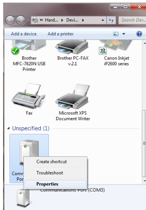
Figure 35. Pop-up Menu
