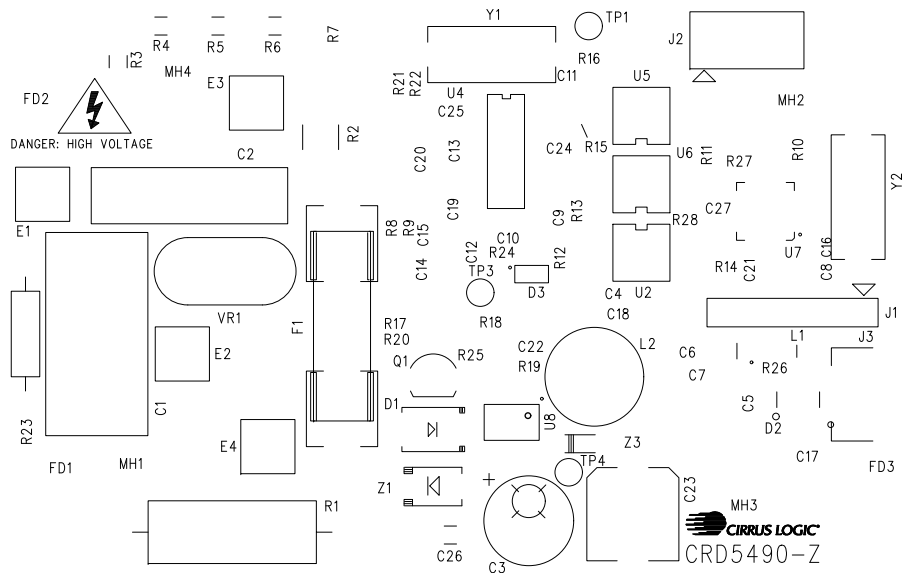
Figure 45. Silkscreen
