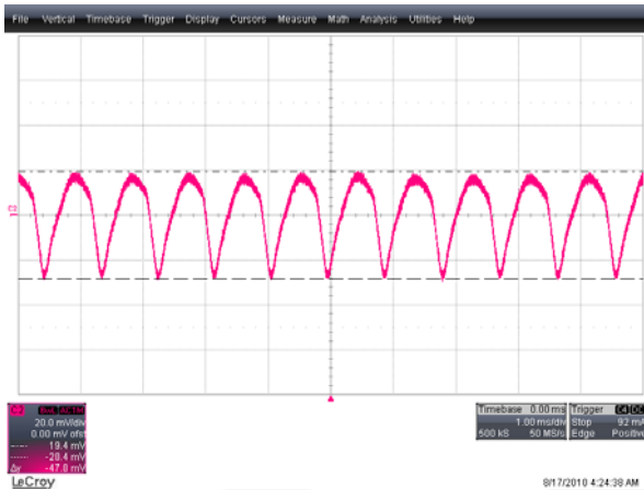
Figure 26. V_{O\_RIPPLE} = 47.8\text{mV} , Maximum Output Ripple at 90\text{V}_{AC} , CH2: V_O (20mV/div), Time: 1ms/div
