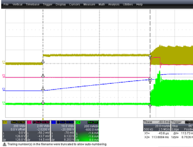
Figure 7. Startup Time (AC Input to V_{CC} UVLO HIGH) = 114ms, 90V AC and Full-Load Condition (CH1: V_{DS} (200V/div), CH2: V_{FB} (2V/div), CH3: V_{CC} (10V/div), CH4: I_{DS} (200mA/div), Time: 20ms/div
