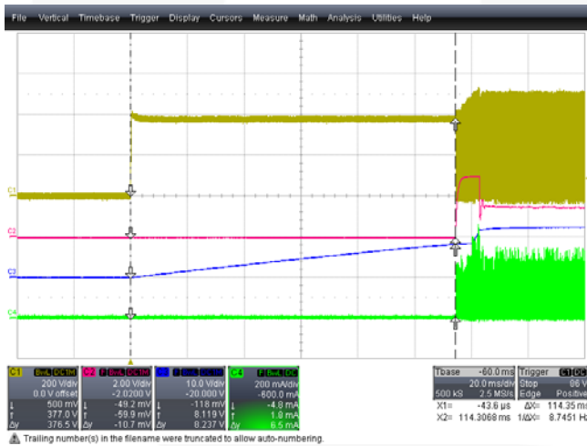
Figure 9. Startup Time (AC Input to V_{CC} UVLO HIGH) = 114ms, 265V AC and Full-Load Condition, (CH1: V_{DS} (200V/div), CH2: V_{FB} (2V/div), CH3: V_{CC} (10V/div), CH4: I_{DS} (200mA/div), Time: 20ms/div
