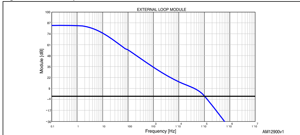
Figure 9. Module plot
