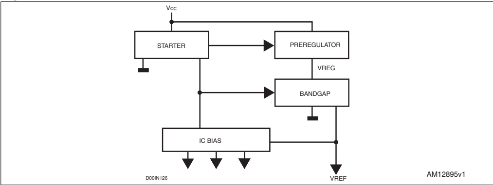
Figure 4. Internal circuit
