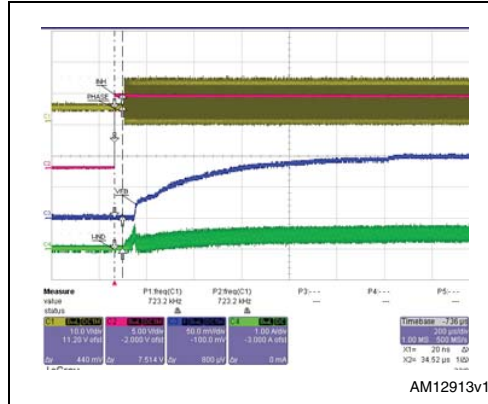
Figure 26. Dimming operation
