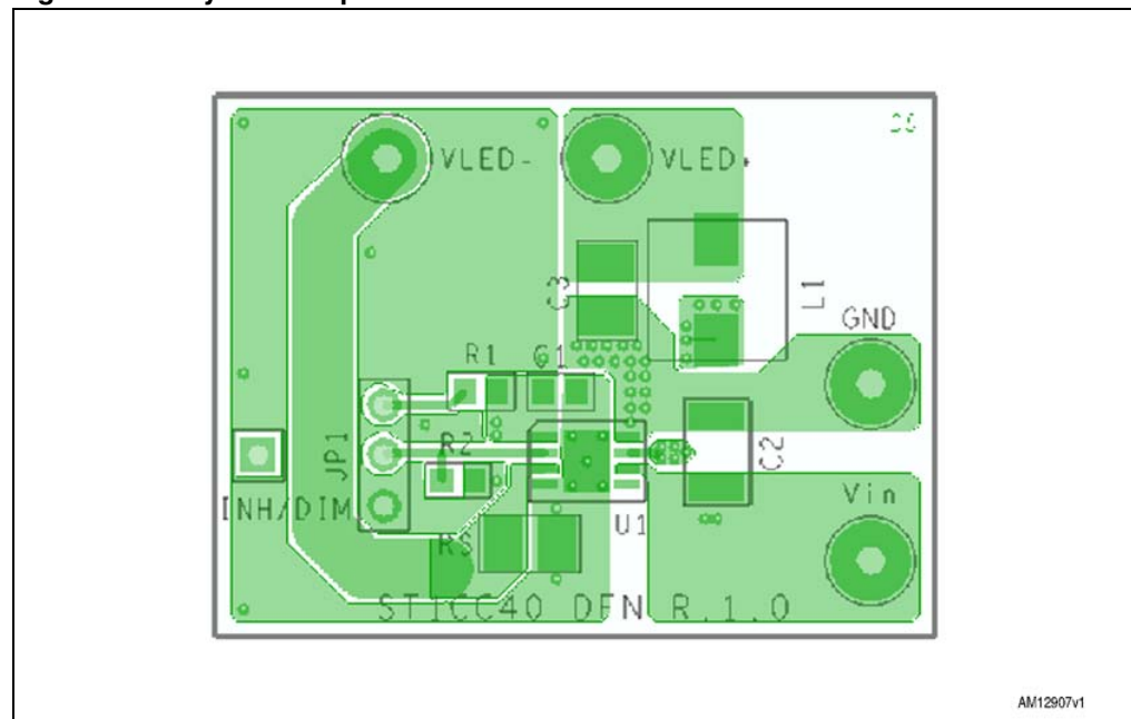
Figure 16. Layout example
