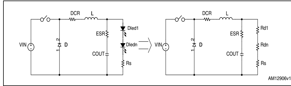
Figure 15. Equivalent circuit
