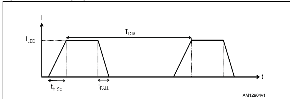
Figure 13. Dimming signal
