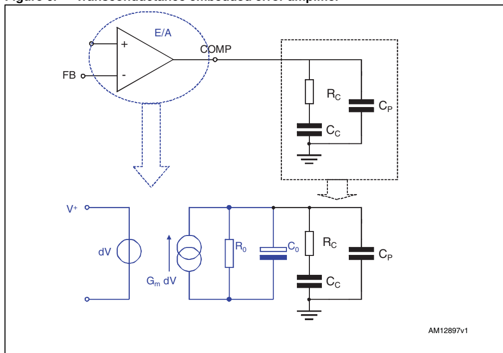
Figure 6. Transconductance embedded error amplifier
