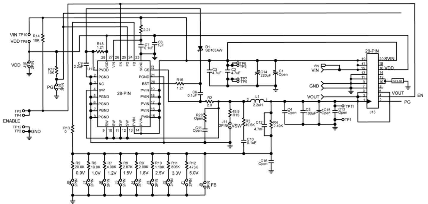
Schematic of MIC26601 Evaluation Board (J11, R13, R15 are for testing purposes)
