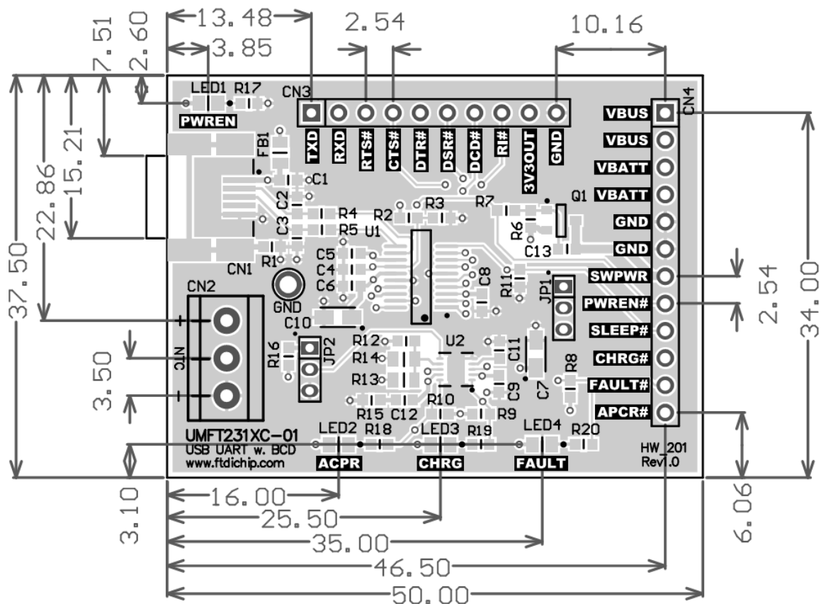
Figure 7.1 – UMFT231XC Module Dimensions
