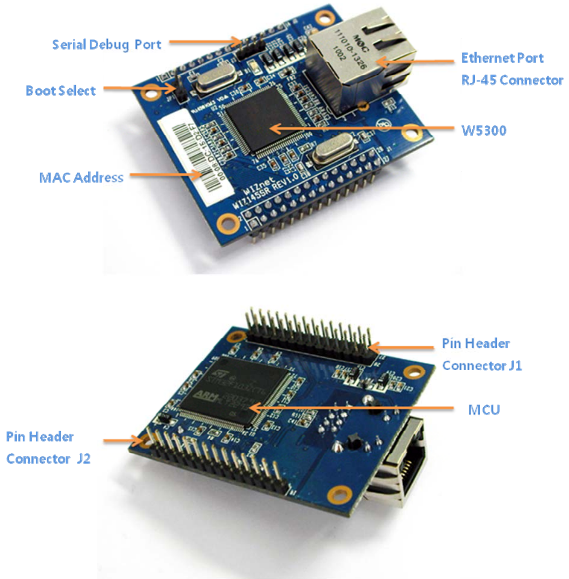
Figure 2. WIZ145SR Module Interface
