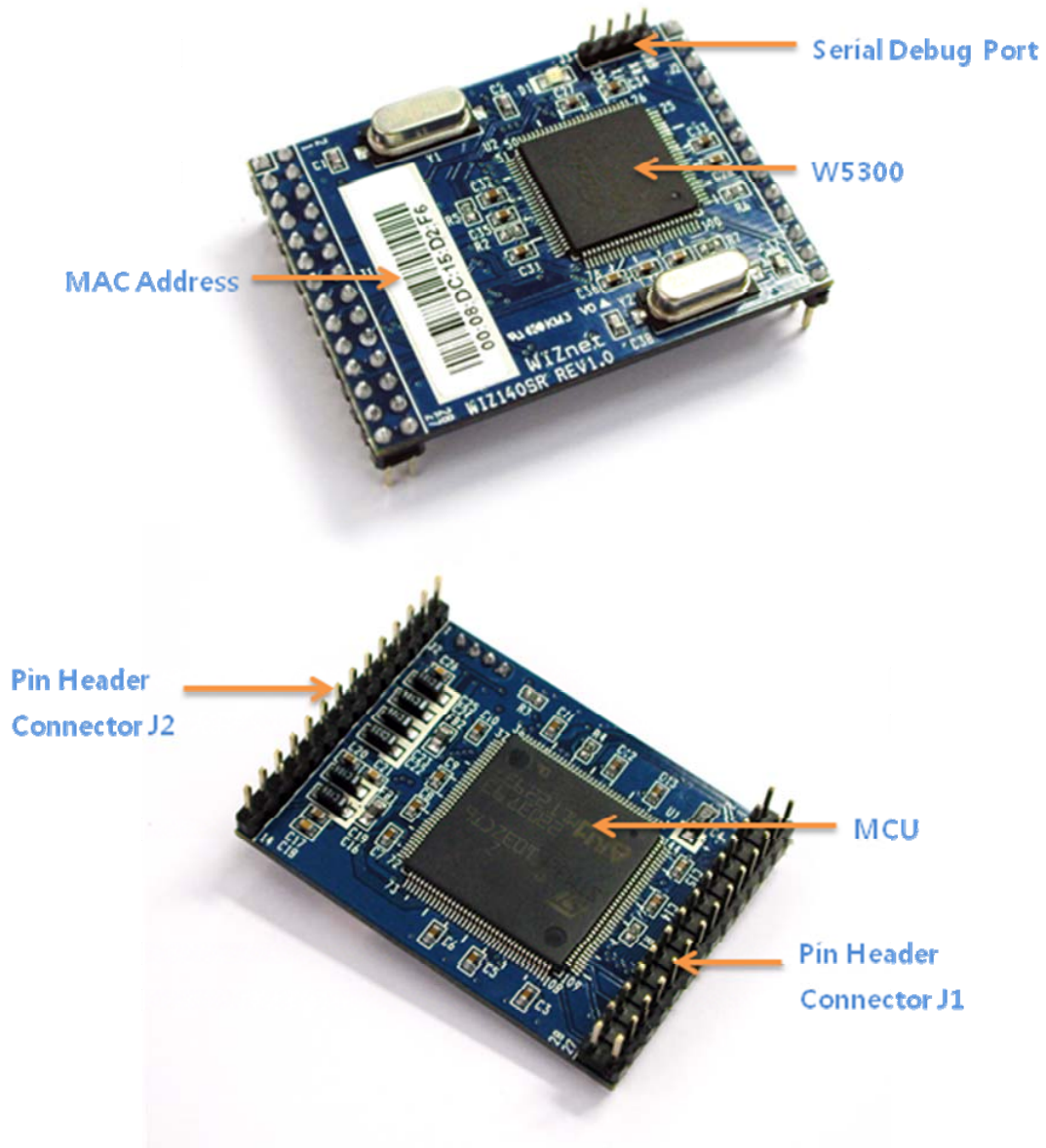
Figure 1. WIZ140SR Module Interface
