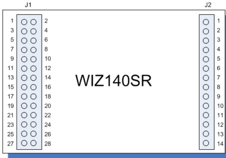
Figure 6. WIZ140SR Module Pin Assign
