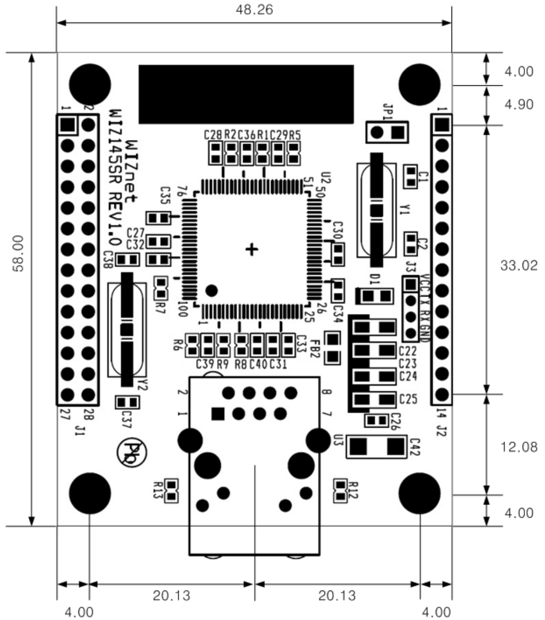
Figure 5. WIZ145SR Module Dimension (mm)
