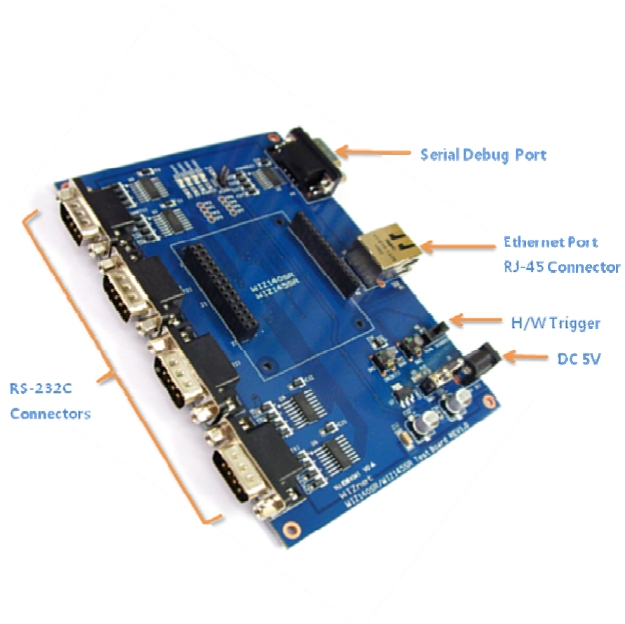
Figure 3. WIZ140SR/WIZ145SR Test Board Interface
