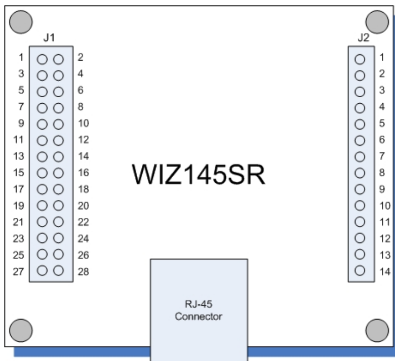
Figure 7. WIZ145SR Module Pin Assign
