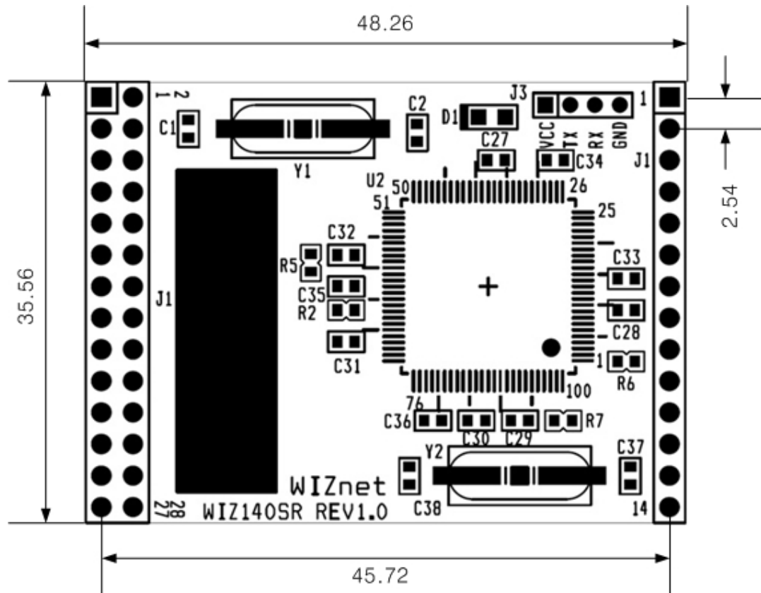
Figure 4. WIZ140SR Module Dimensions (mm)
