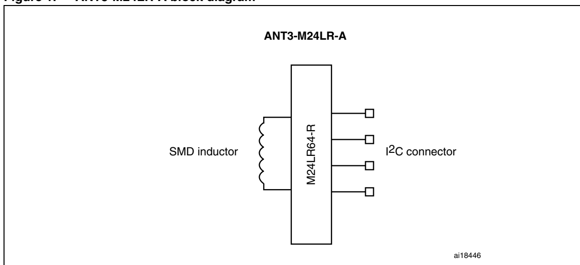
Figure 1. ANT3-M24LR-A block diagram
