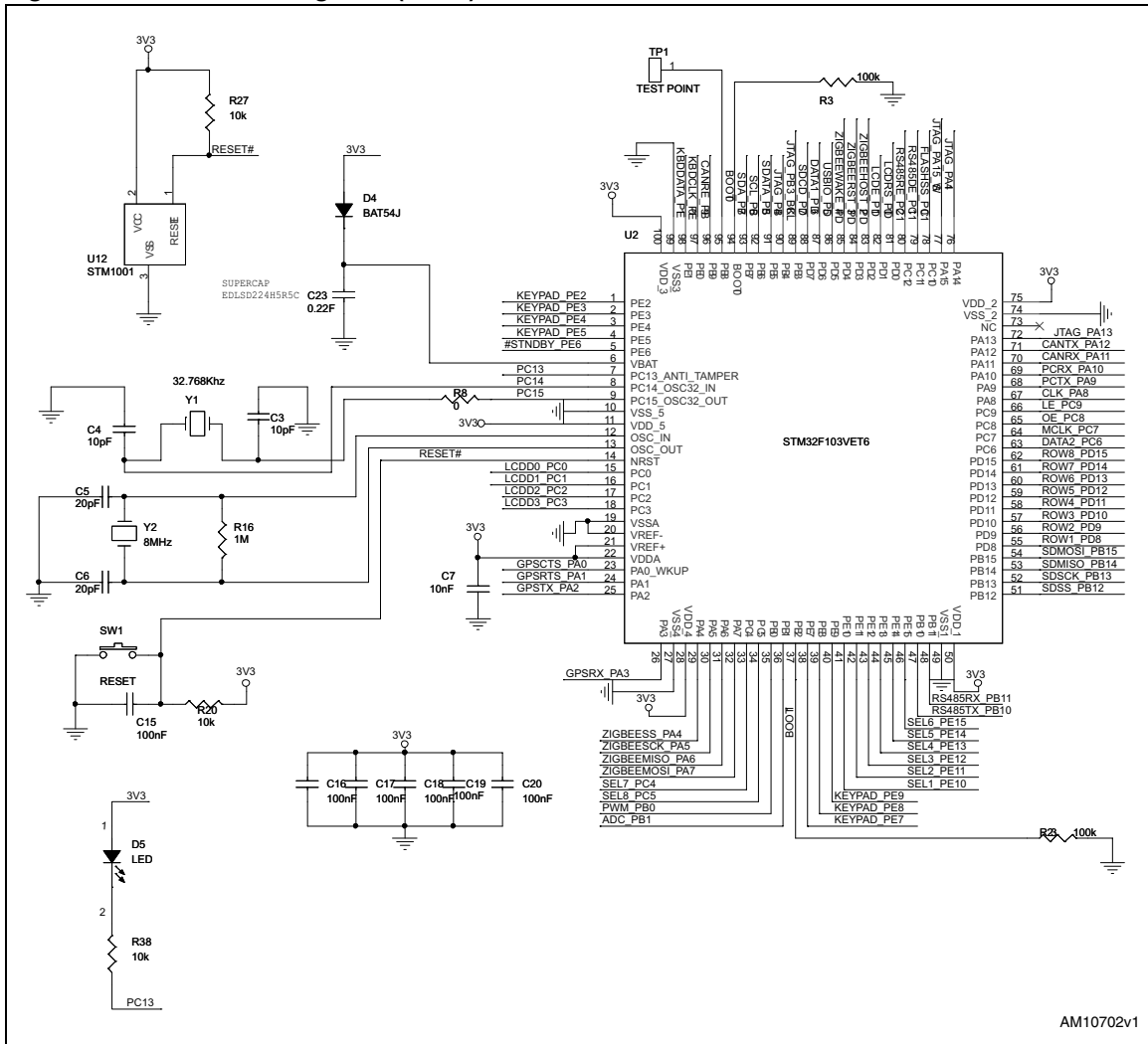
Figure 3. Schematic diagrams (3 of 3)
