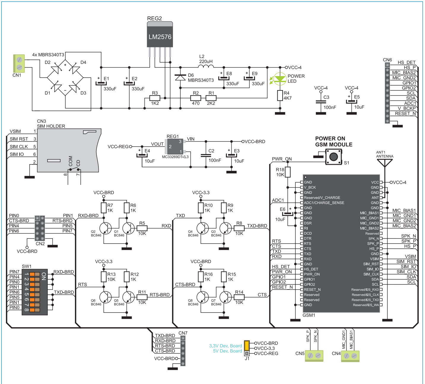
Figure 4: SmartG100 connection schematics
