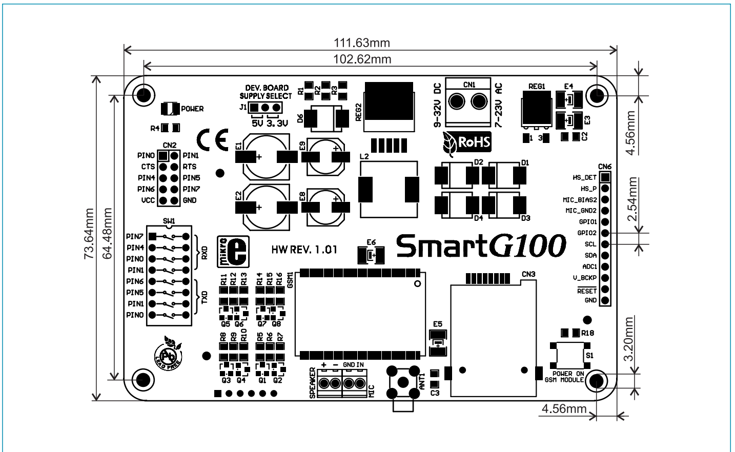
Figure 3: SmartG100 dimensions
