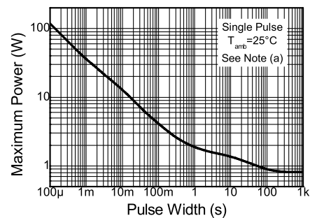
Pulse Power Dissipation
