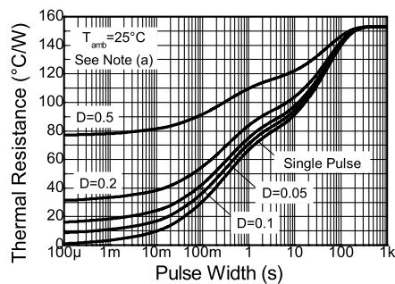
Transient Thermal Impedance
