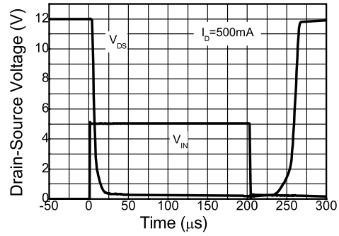
Switching Speed
