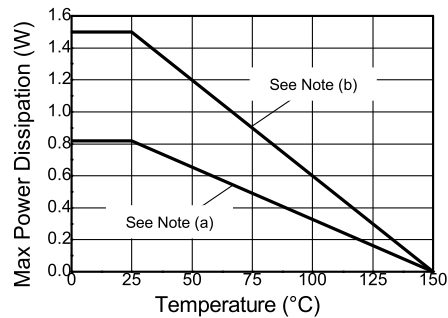
Derating Curve
