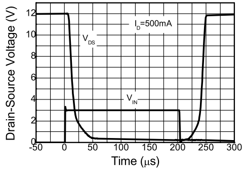
Switching Speed
