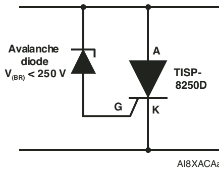
Figure 2. Overvoltage Protection Circuit
