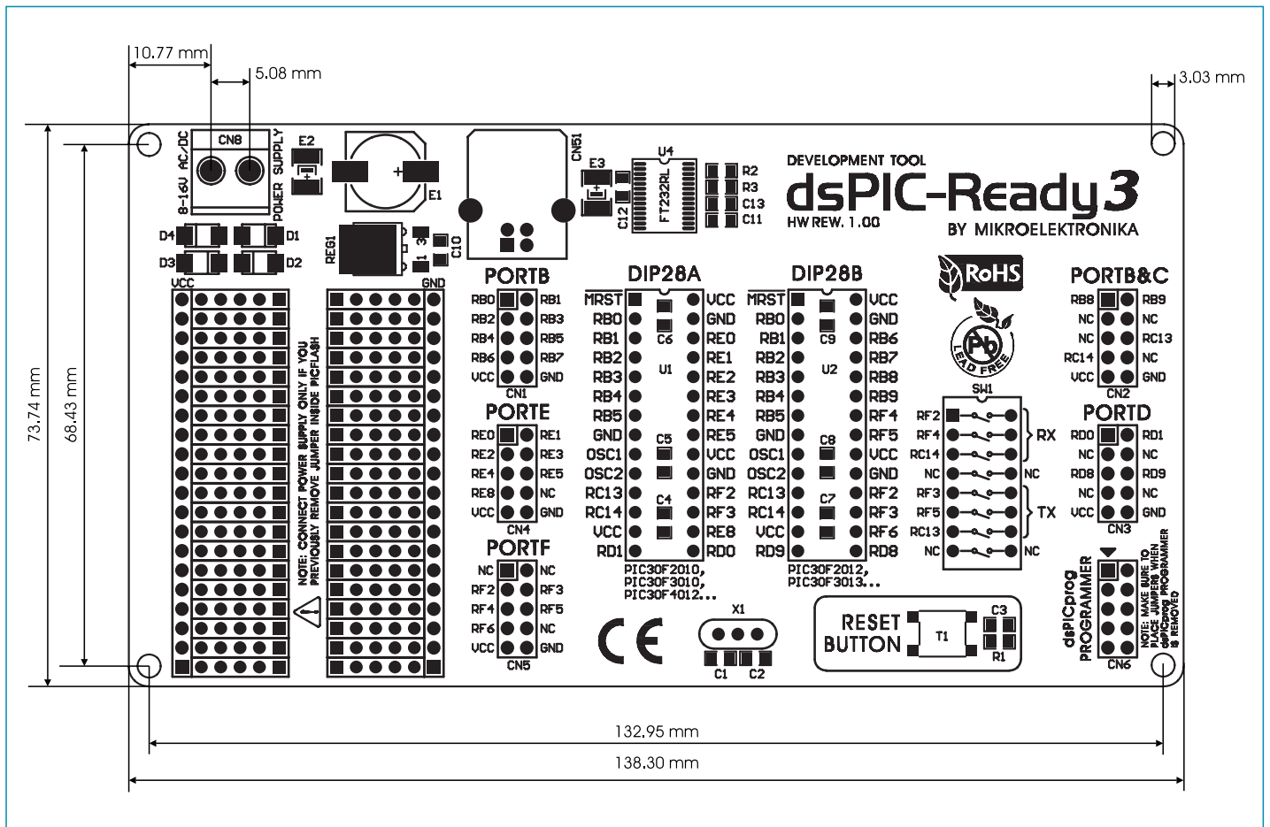
Figure 4: Dimensions of the dsPIC Ready3 additional board
