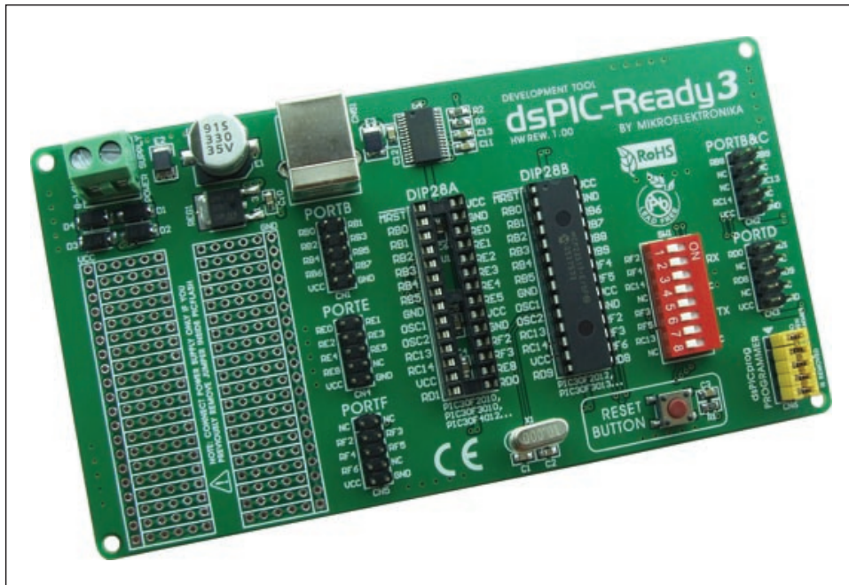
Figure 1: dsPIC Ready3 additional board
