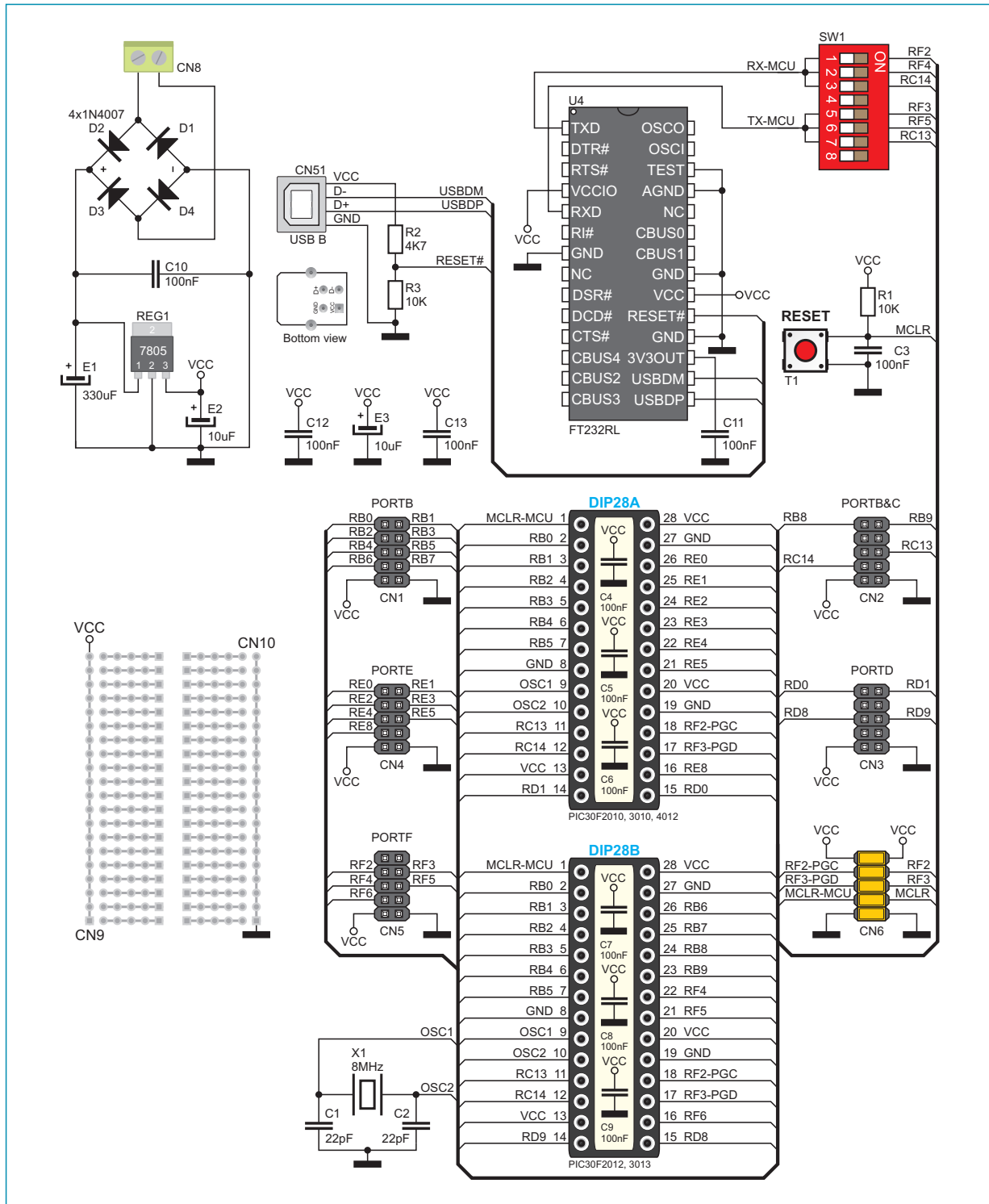
Figure 3: The dsPIC Ready3 board connection schematic
