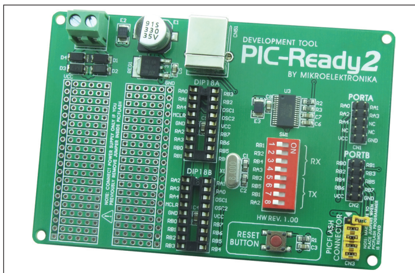
Figure 1: PIC-Ready2 additional board
