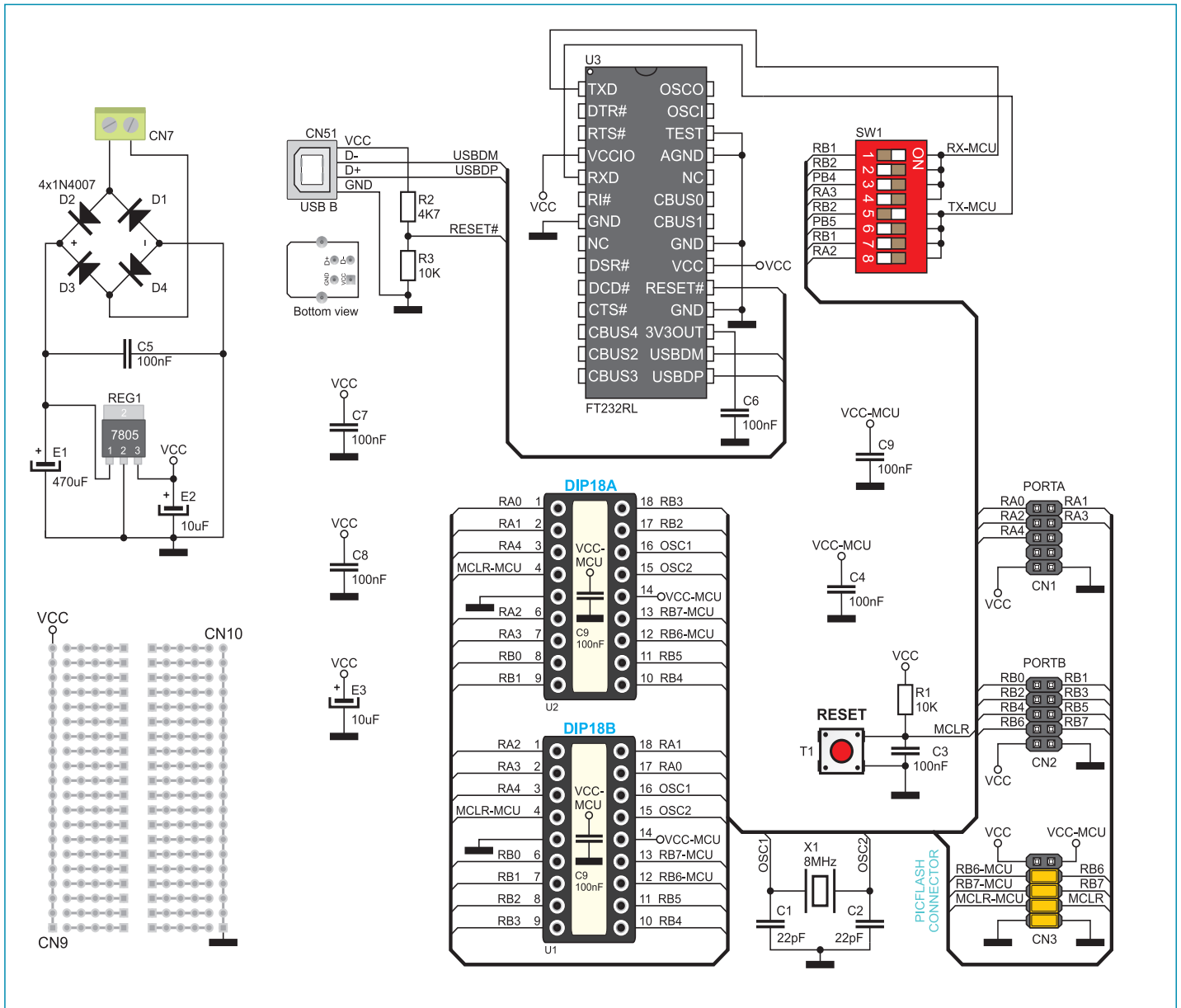
Figure 4: Additional board connection schematic
