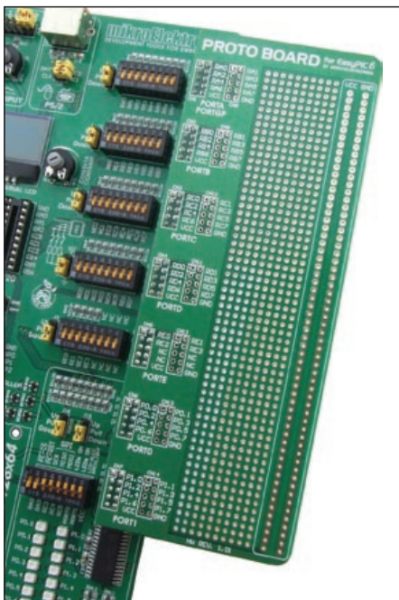
Figure 1-2: Proto board connected to EasyPIC6
