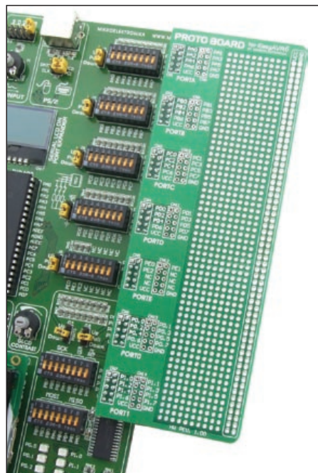
Figure 1-3: Proto board connected to EasyAVR6
