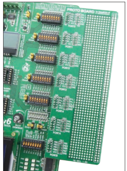
Figure 1-4: Proto board connected to Easy8051 v6
