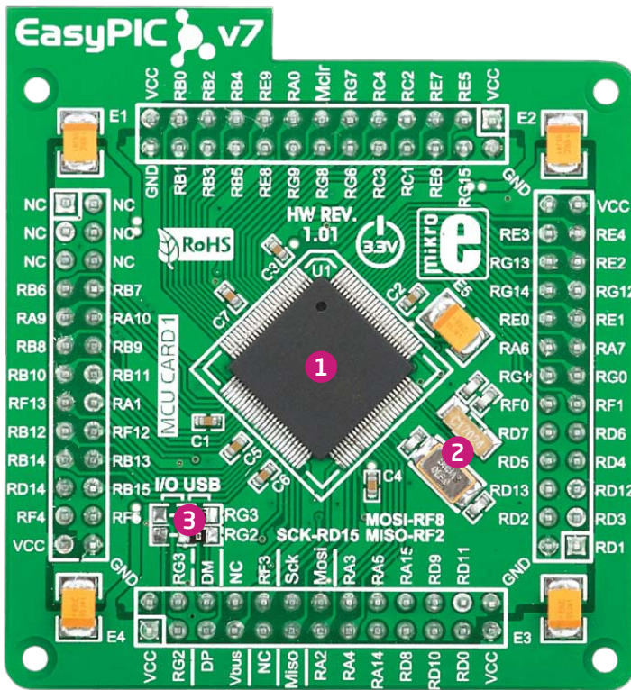
Figure 1: MCU card with PIC24EP512GU810
