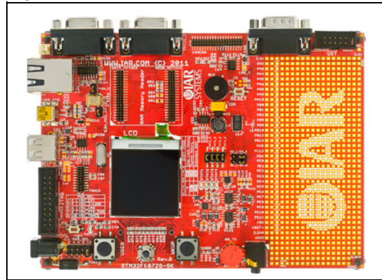
Figure 1. Evaluation board
