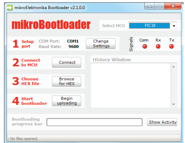
Figure 2-1: mikroBootloader window
