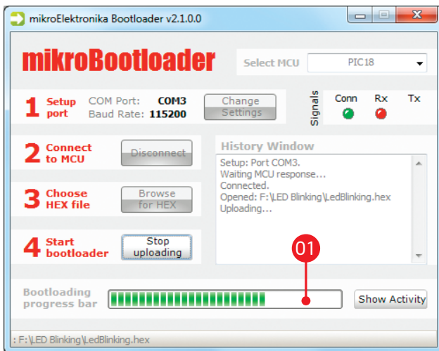
Figure 2-8: Progress bar
