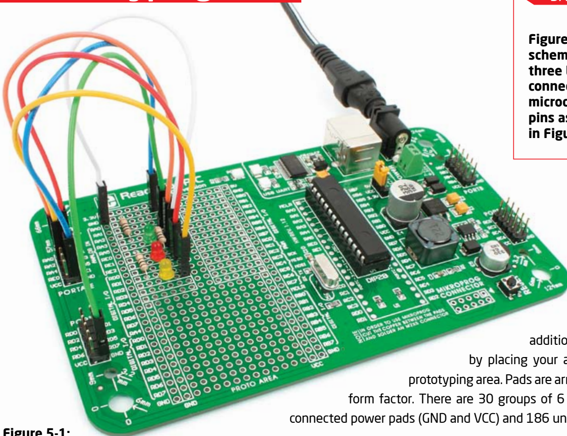
Figure 5-1: Proto area usage
