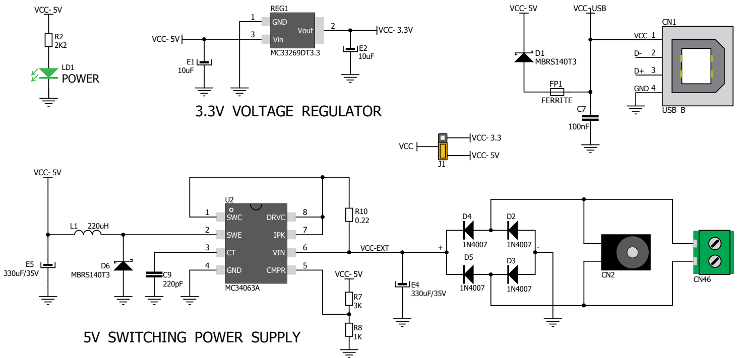
Figure 1-4: Power supply schematic
