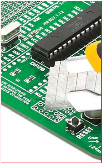
Figure 3-2: cutting copper between pads
