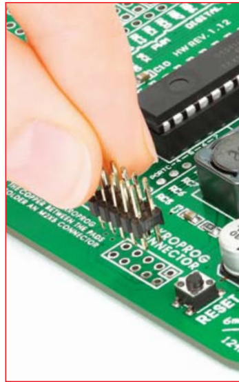
Figure 3-3: placing 2x5 male header
