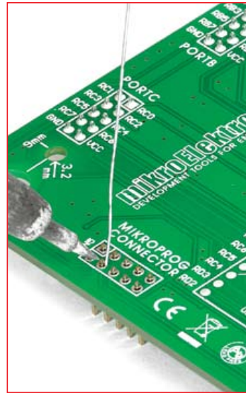
Figure 3-4: soldering 2x5 male header on the pads
