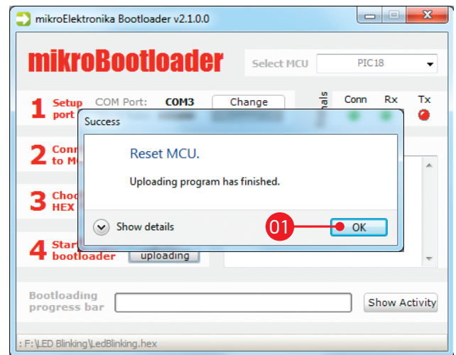
Figure 2-9: Restarting MCU
