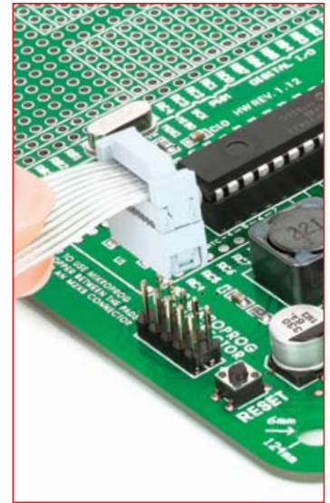
Figure 3-5: Connecting mikroProg™ programmer
