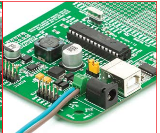
Figure 1-3: screw terminals power supply
