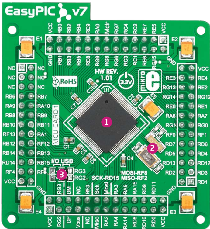
Figure 1: MCU card with dsPIC33EP512MU810
