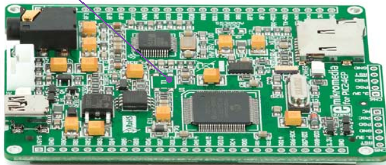
Figure 4-1: Location of additional reset button
