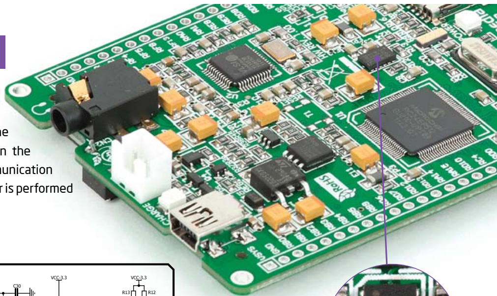
Figure 10-1: Accelerometer module
