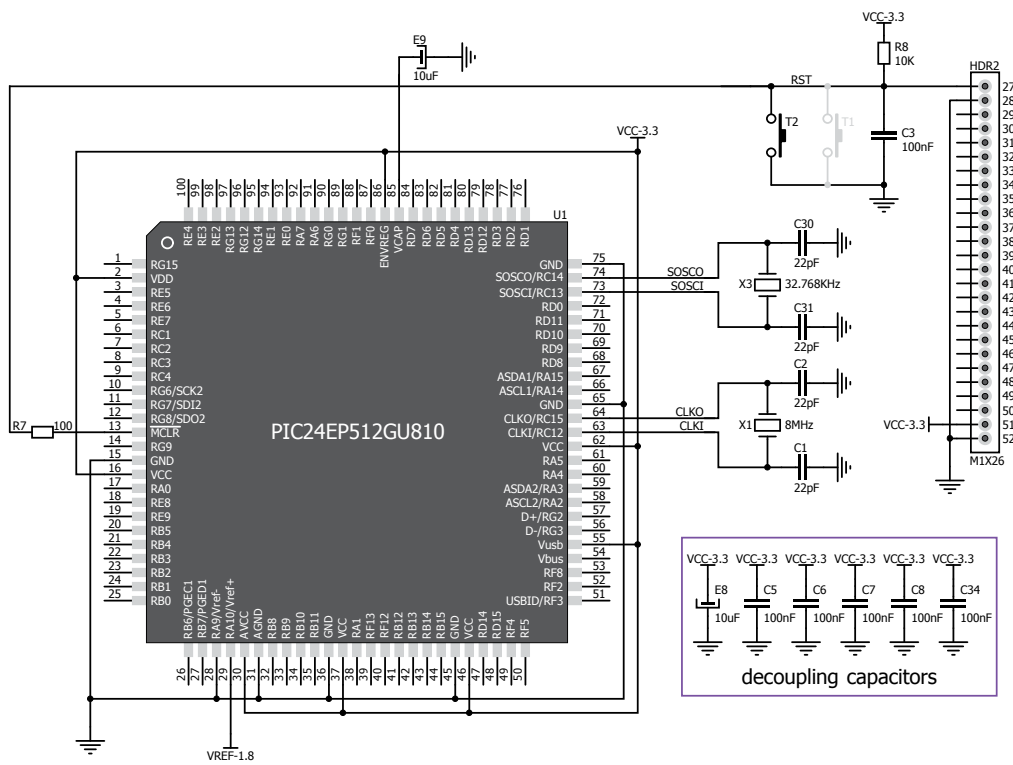
Figure 4-3: Reset circuit schematic
