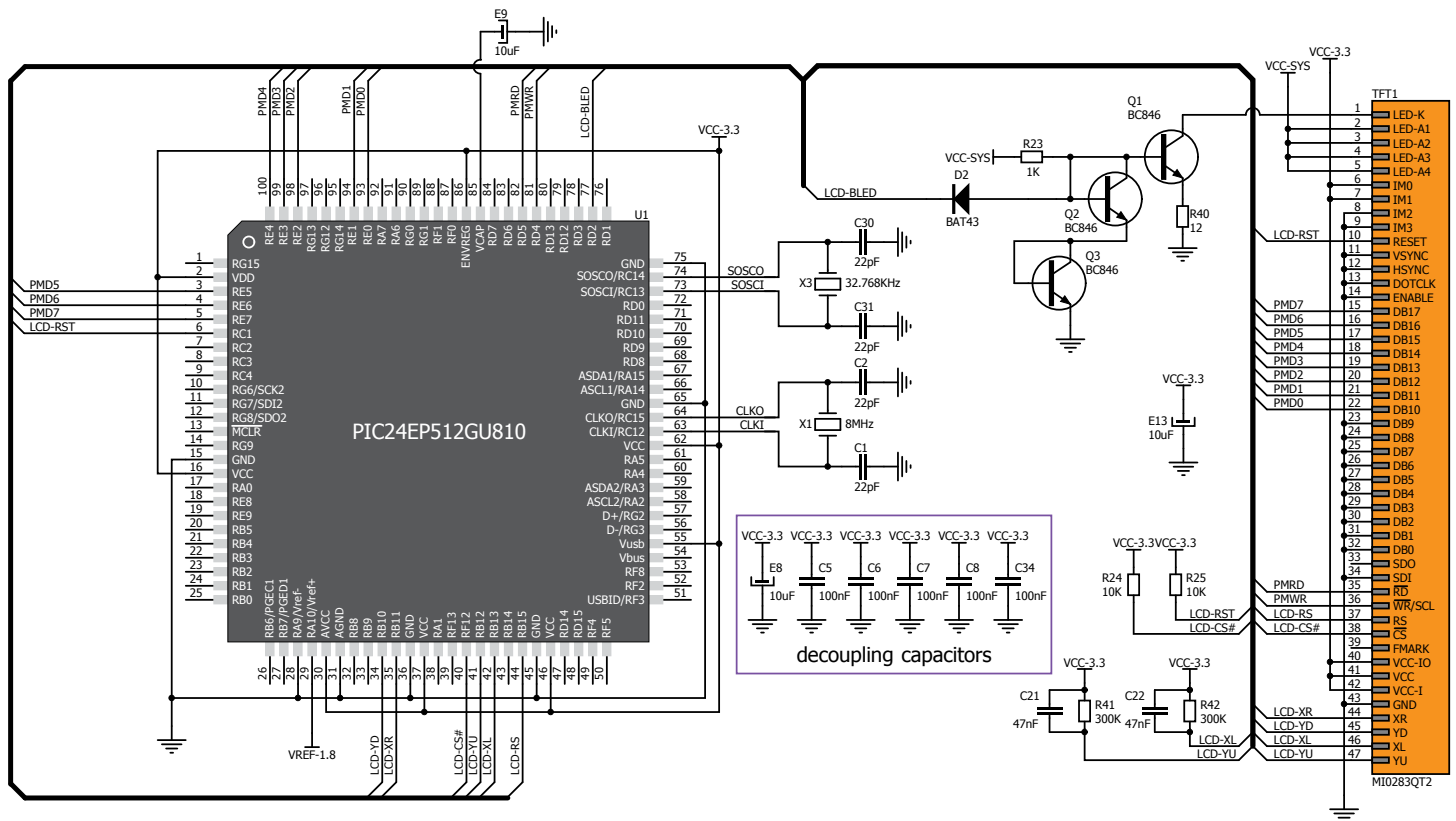
Figure 7-2: Touch Screen connection schematic
