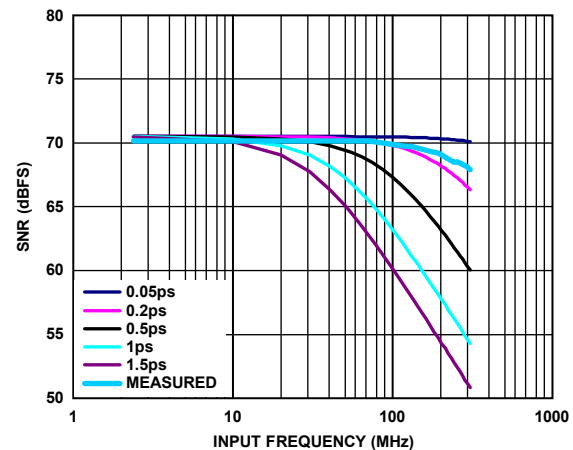
Figure 56. AD9634-250 SNR vs. Input Frequency and Jitter
