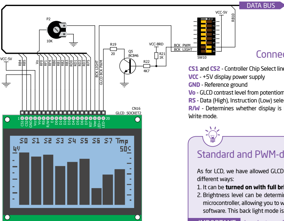
Figure 12-1: GLCD 128x64 connection schematics
