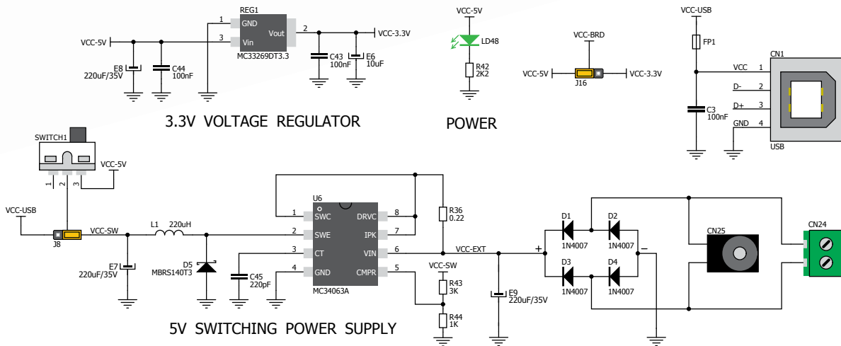
Figure 3-2: Dual power supply unit schematics
