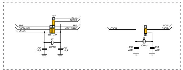
Figure 4-2: crystal oscillators
