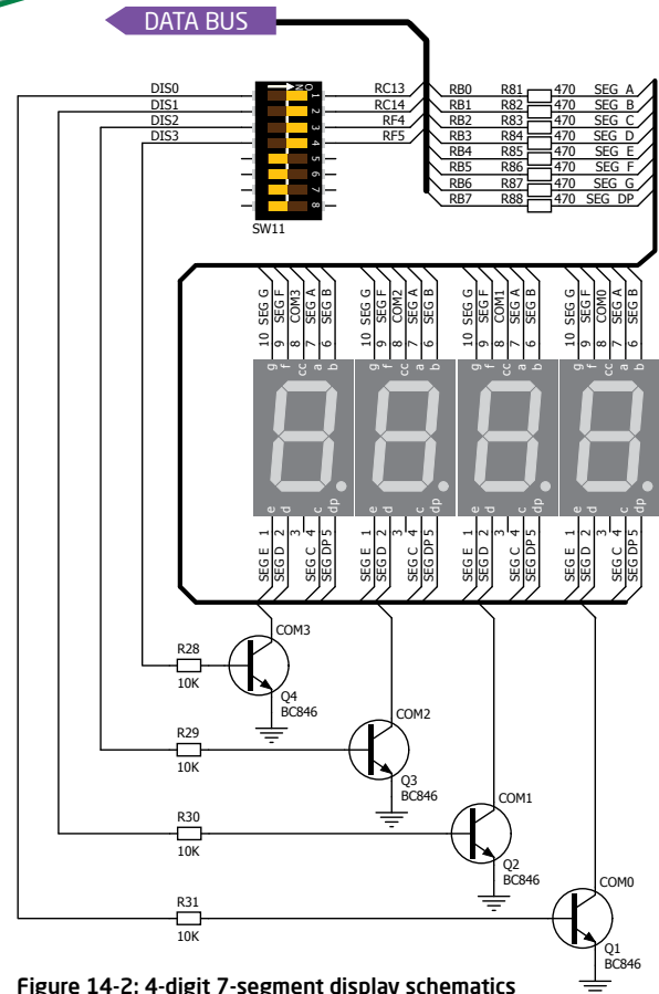
Figure 14-2: 4-digit 7-segment display schematics
