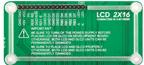
Figure 11-1: On-board LCD 2x16 display connector
