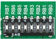
Figure 10-2: Tri-state DIP switch on PORTB
