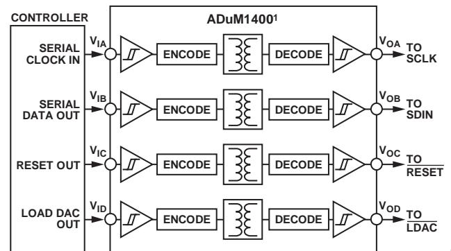
Figure 53. Isolated Interface
