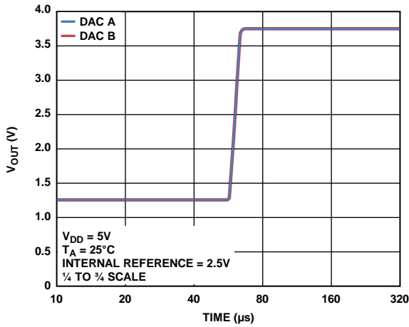
Figure 30. Settling Time
