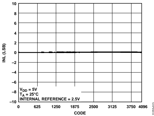
Figure 12. Integral Nonlinearity (INL) vs. Code
