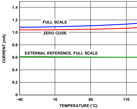
Figure 29. Supply Current vs. Temperature
