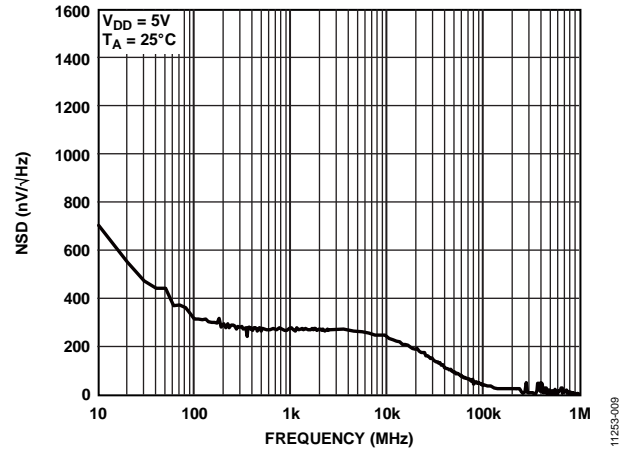
Figure 8. Internal Reference Noise Spectral Density vs. Frequency
