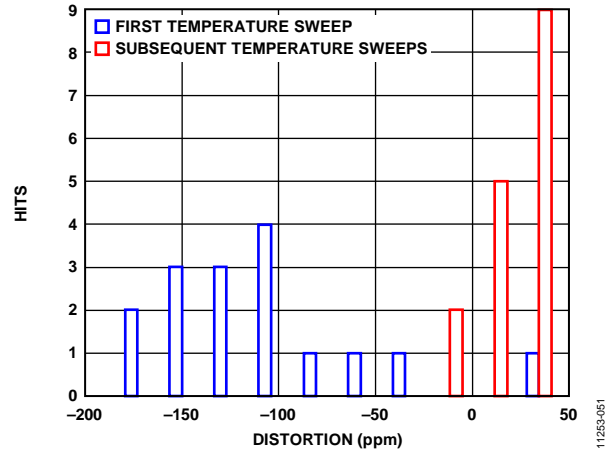
Figure 50. Thermal Hysteresis
