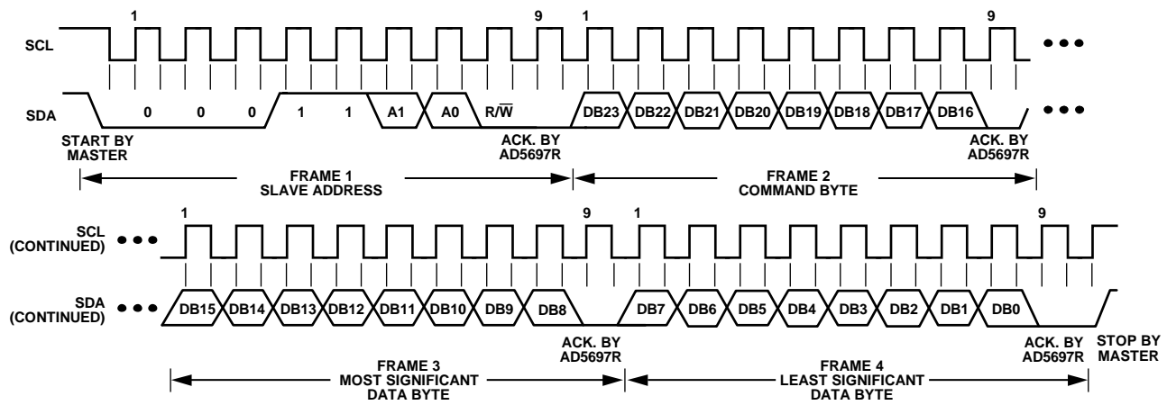
Figure 44. I 2 C Write Operation
