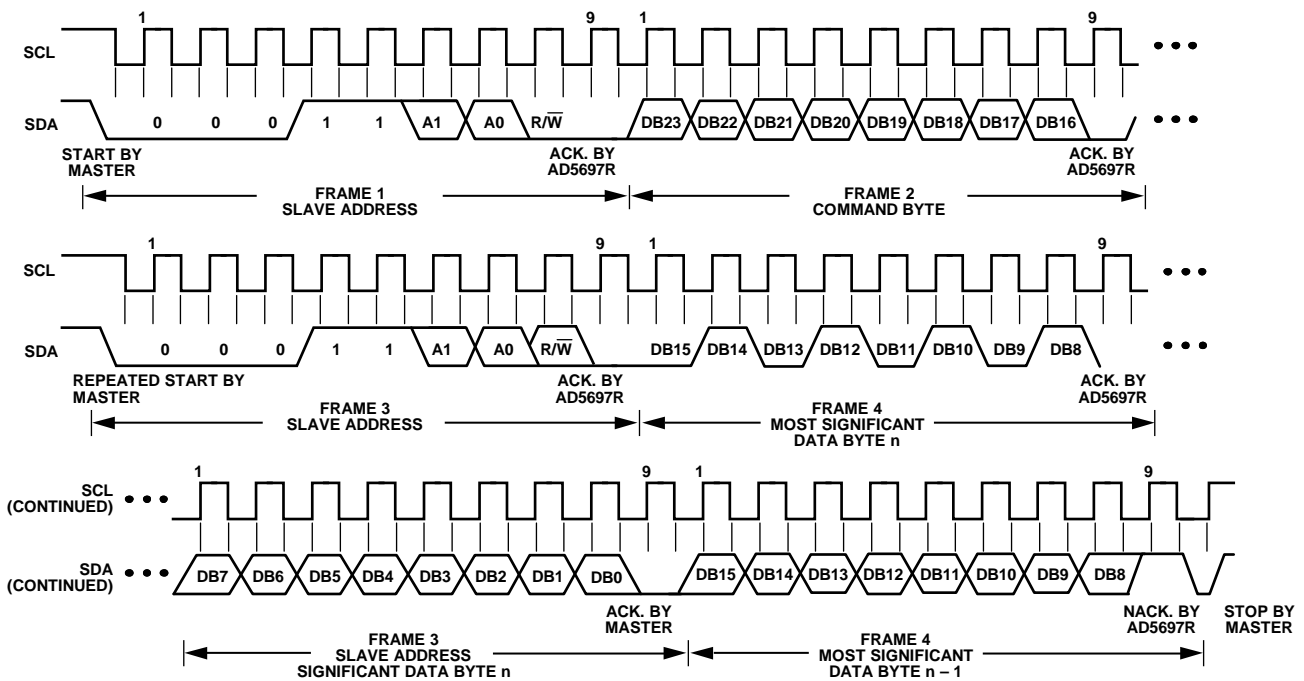
Figure 45. I 2 C Read Operation
