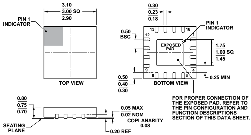
Figure 54. 16-Lead Lead Frame Chip Scale Package [LFCSP_WQ] 3 mm x 3 mm Body, Very Very Thin Quad (CP-16-22)
