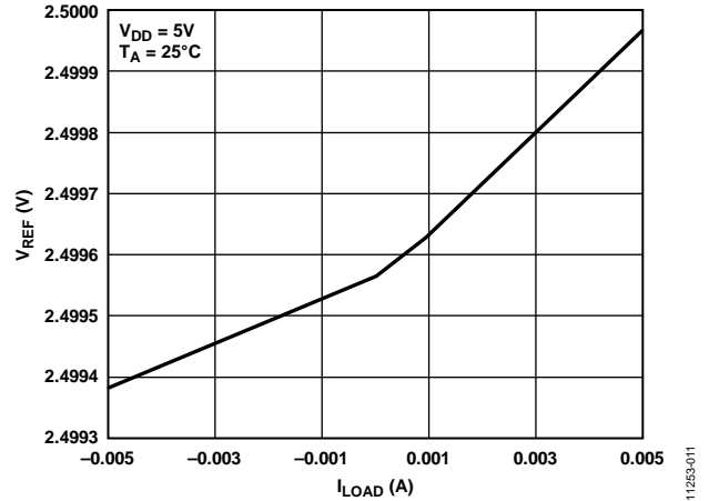
Figure 10. Internal Reference Voltage vs. Load Current
