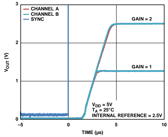
Figure 32. Exiting Power-Down to Midscale
