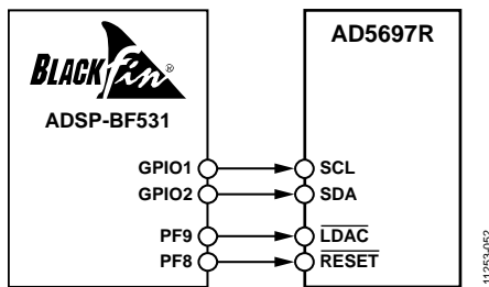
Figure 51. ADSP-BF531 Interface to the AD5697R
