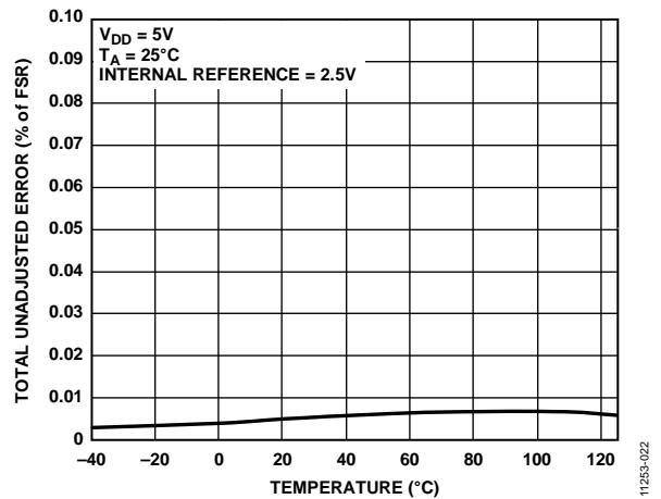
Figure 21. Total Unadjusted Error vs. Temperature
