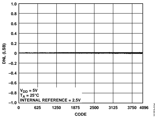
Figure 13. Differential Nonlinearity (DNL) vs. Code
