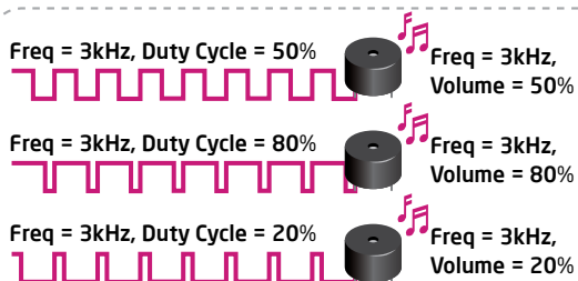
Figure 19-1: Piezo buzzer connected to RD3 microcontroller pin
