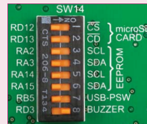
Figure 19-2: push SW14.8 to ON position to connect Piezo buzzer to RD3
