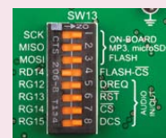
Figure 14-2: Enabling audio codec communication lines
