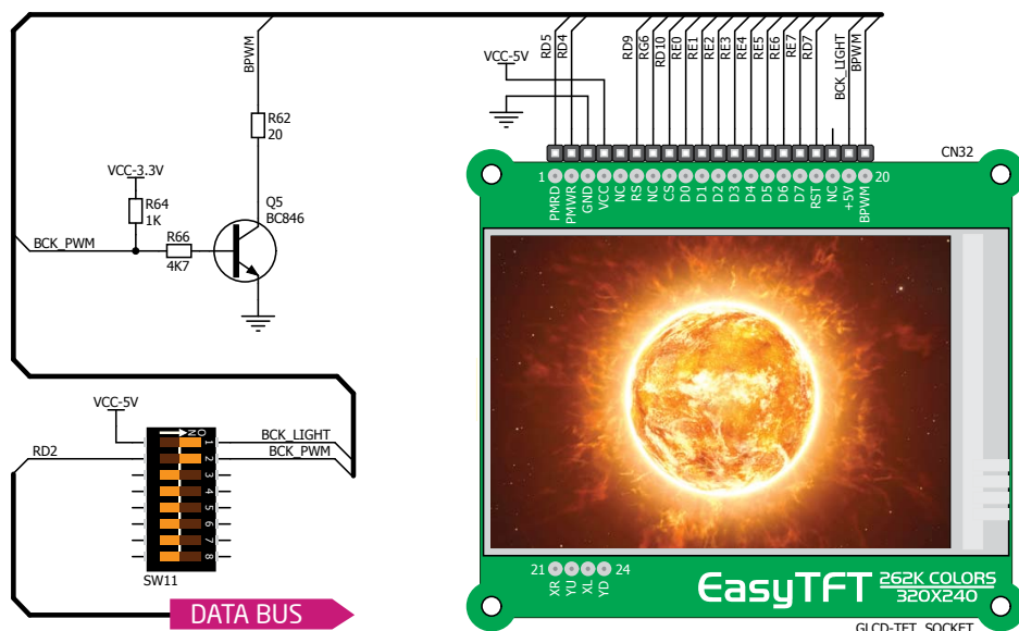
Figure 16-1: TFT display connection schematic
