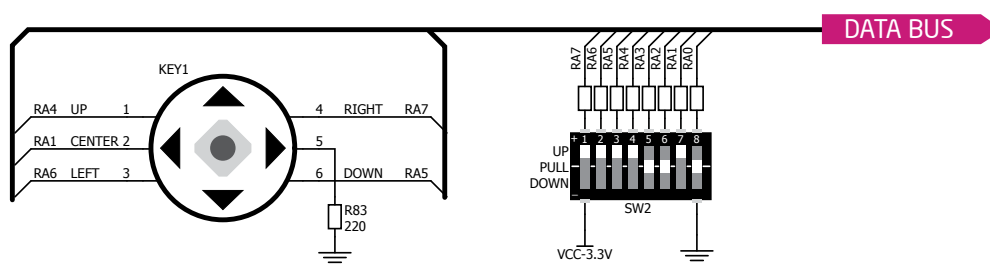
Figure 18-1: Navigation switch connection schematic. Pull-up resistors should be enabled during operation
