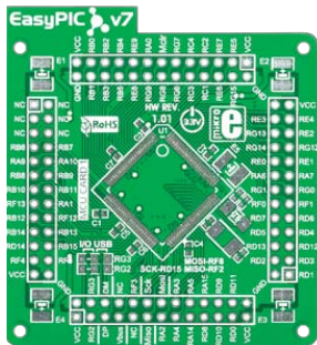
Empty 100-pin TQFP PF MCU CARD 1
