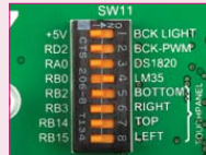
Figure 21-3: Enabled SW11.4 DIP switch
