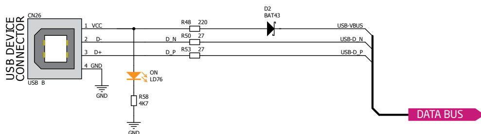
Figure 11-1: USB device connection schematic
