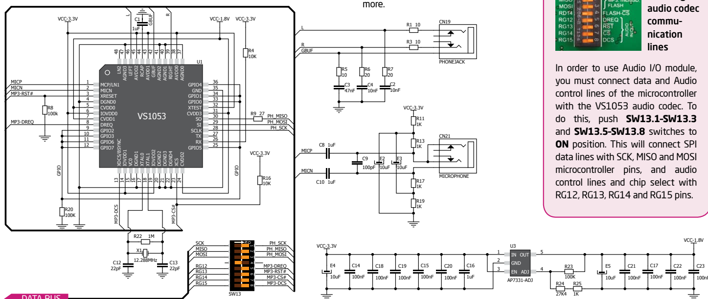
Figure 14-1: Audio IN/OUT connection schematic
