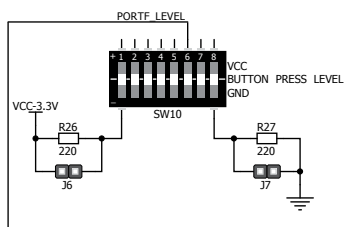
Figure 6-2: Tri-state DIP switch on PORTF
