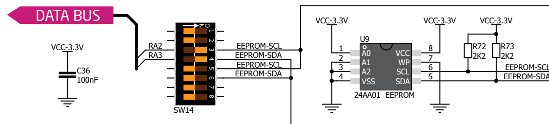
Figure 23-1: Schematic of I 2 C EEPROM module
