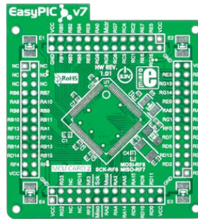
Empty 100-pin TQFP PF MCU CARD 2
