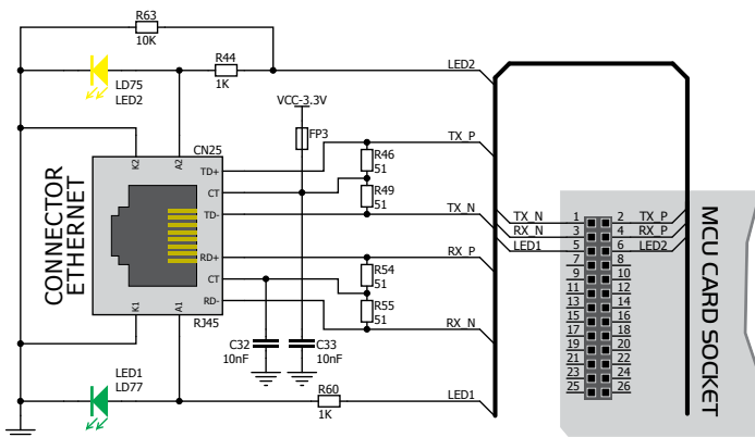
Figure 12-1: Ethernet connection schematic
