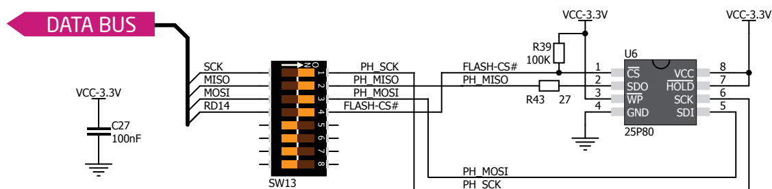
Figure 22-1: Schematic of Serial Flash Memory module
