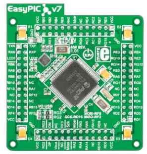
100-pin TQFP PT ETHERNET CARD with PIC32MX795F512L
