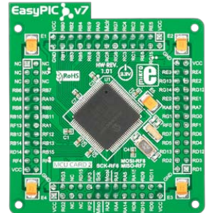
100-pin TQFP PF MCU CARD 2 with dsPIC33FJ256GP710A
