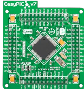
100-pin TQFP PT MCU CARD 1 with dsPIC33EP512MU810
