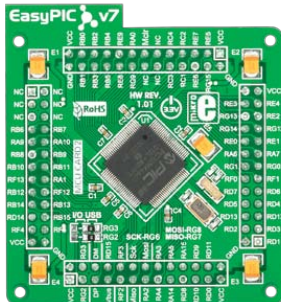
100-pin TQFP PT MCU CARD 2 with PIC32MX460F512L
