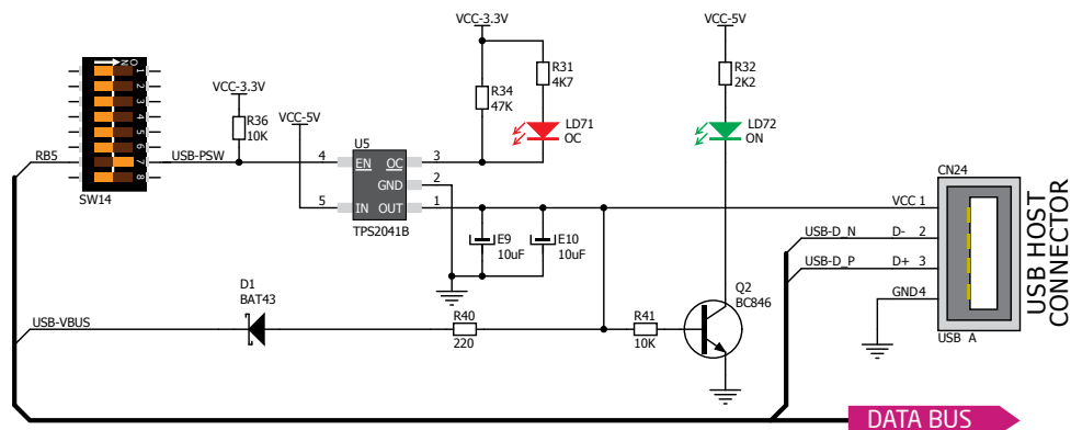
Figure 10-1: USB host connection schematic
