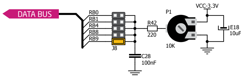
Figure 24-1: Schematic of ADC input
