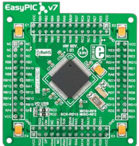
100-pin TQFP PT MCU CARD 1 with PIC24EP512GU810
