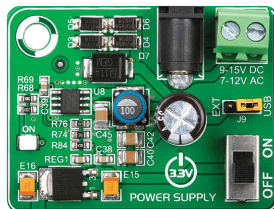
Figure 3-1: Power supply unit of EasyPIC Fusion™ v7
