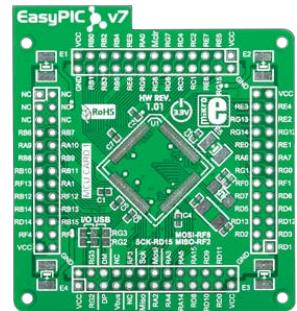
Empty 100-pin TQFP PT MCU CARD 1
