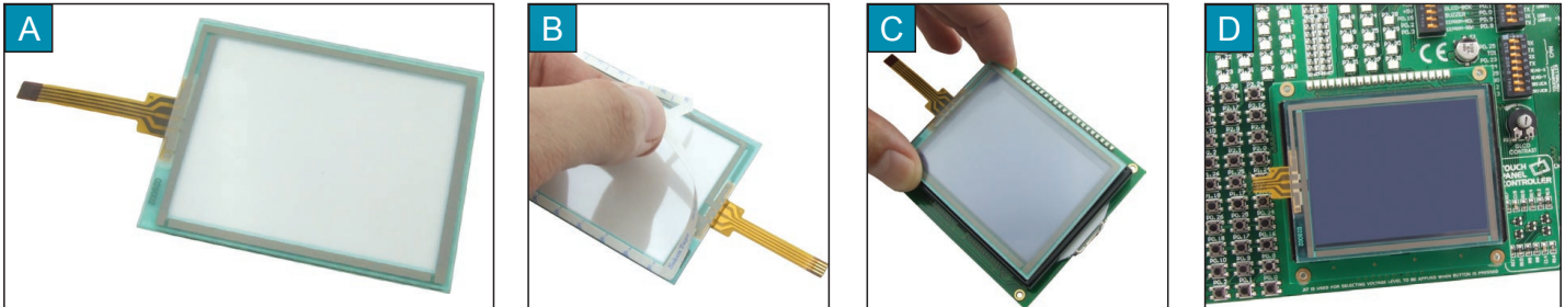
Figure 16-1: Placing touch panel over a GLCD
