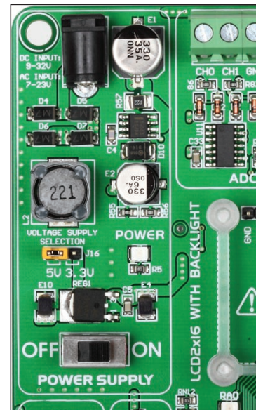
Figure 1-2: Power supply module
