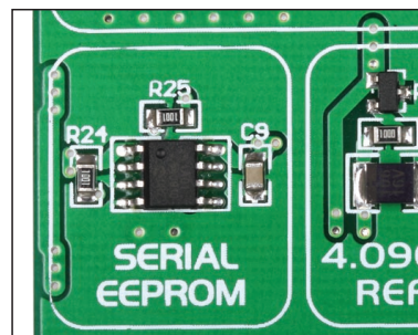
Figure 8-1: EEPROM module
