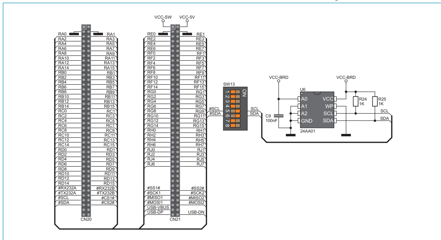
Figure 8-2: EEPROM module connection schematic
