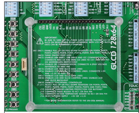
Figure 15-2: GLCD connector
