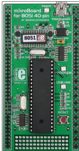
Figure 2-2: mikroBoard for 8051 40-pin
