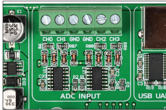
Figure 6-1: ADC module
