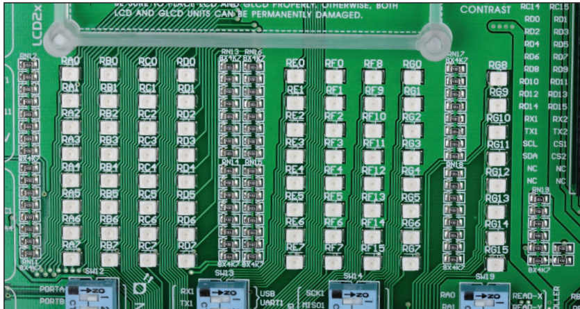
Figure 12-1: LEDs
