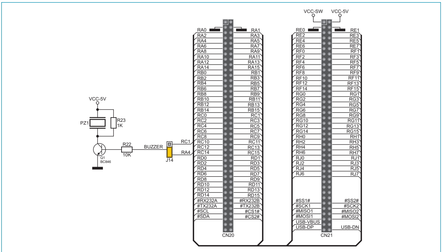
Figure 9-4: Piezo buzzer connection schematic
