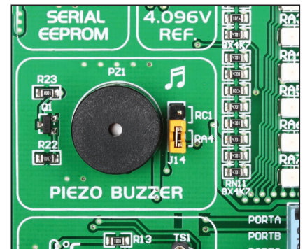
Figure 9-3: Signal generation via RA4
