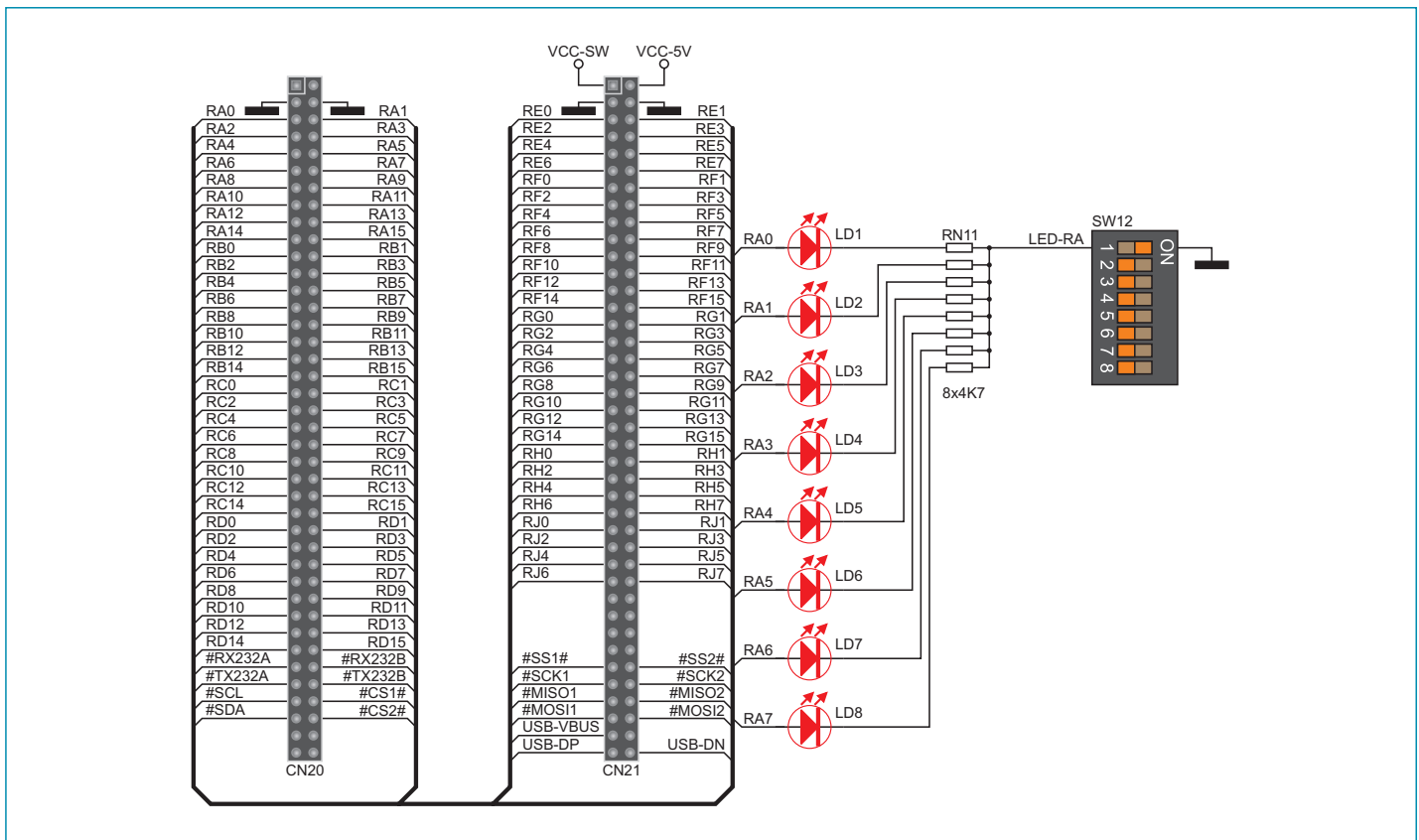
Figure 12-2: LED and port PORT0 connection schematic
