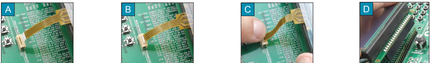
Figure 16-3: Connecting touch panel
