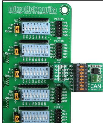
Figure 17-2: Additional board connected to I/O port
