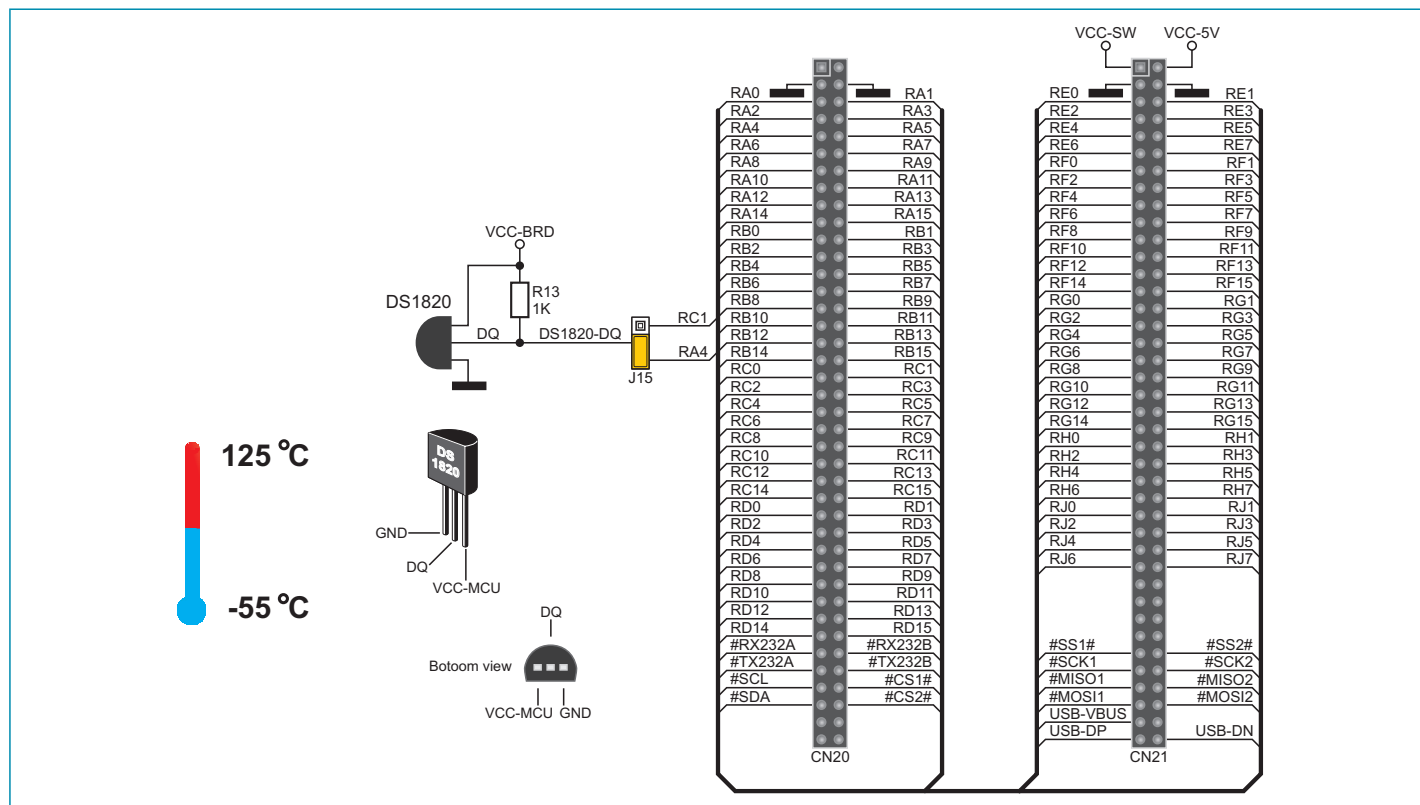
Figure 10-4: DS1820 and microcontroller connection schematic
