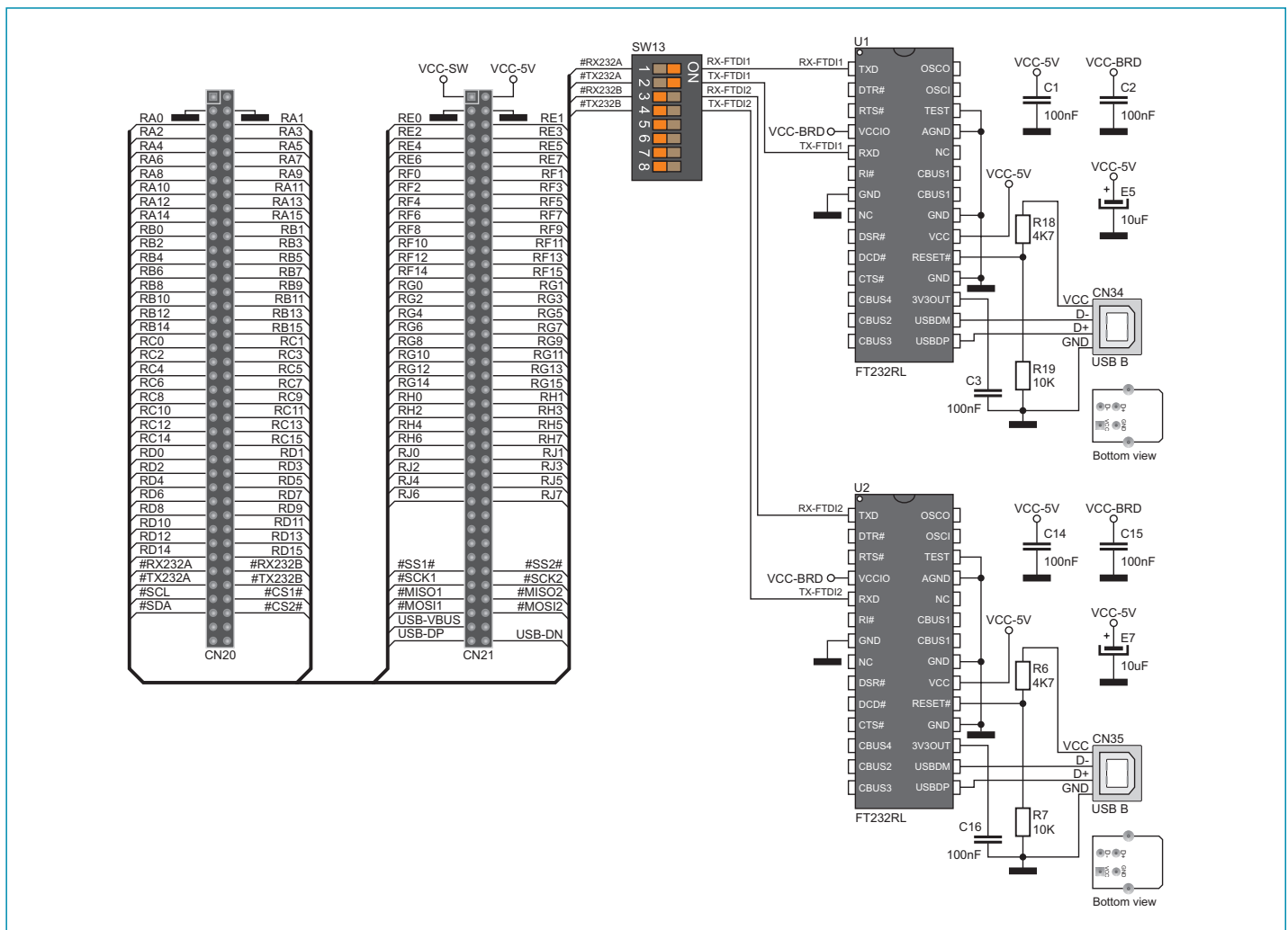
Figure 5-2: USB UART modules connection schematic
