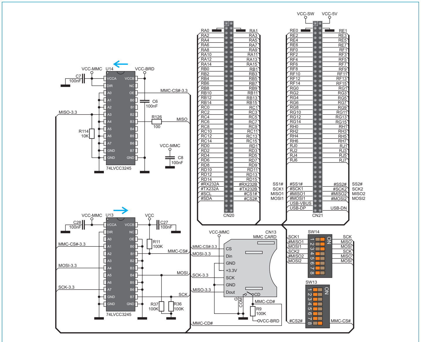
Figure 11-2: MMC/SD connector and microcontroller connection schematic
