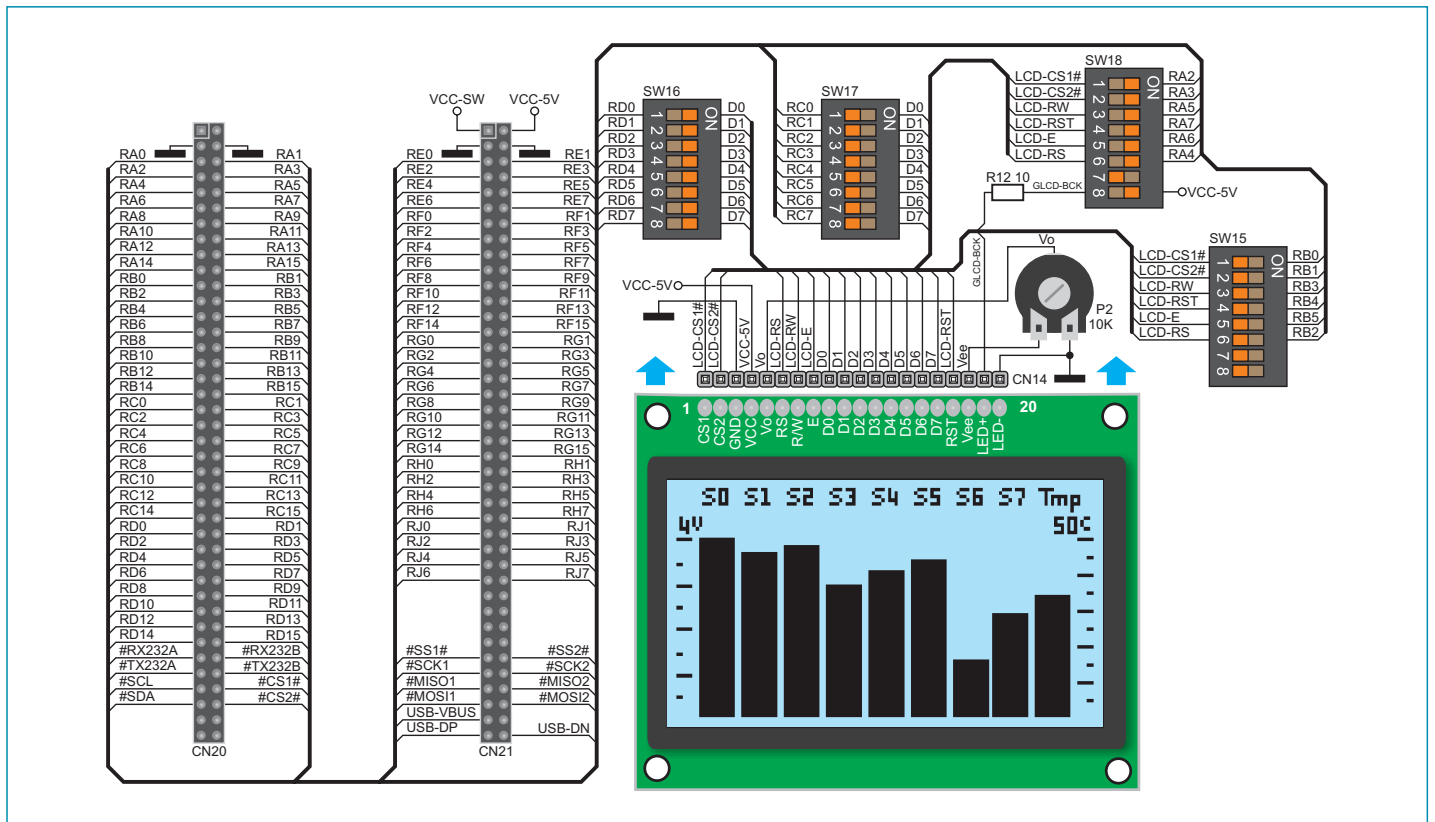
Figure 15-3: GLCD display connection schematic
