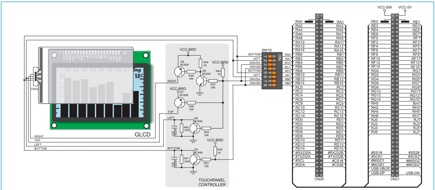
Figure 16-2: Touch panel connection schematic
