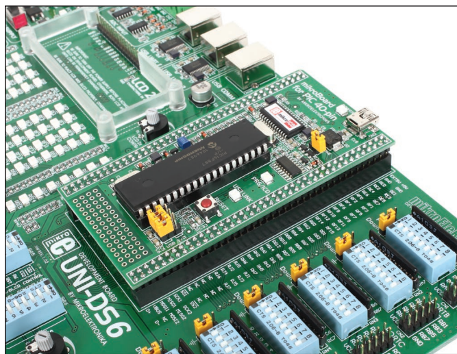
Figure 3-1: mikroBoard placed in socket
