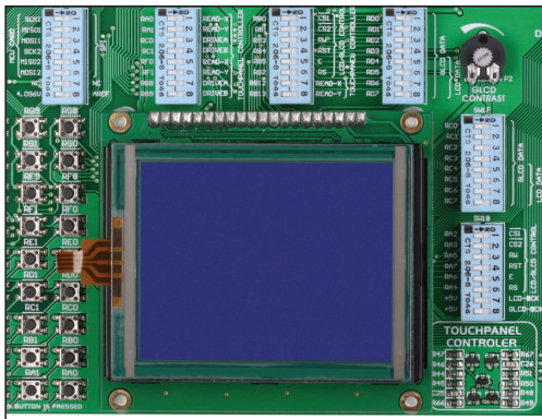
Figure 15-1: GLCD display
