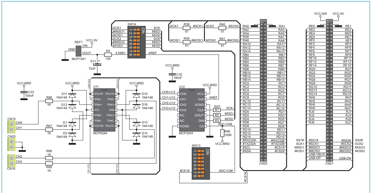
Figure 6-2: ADC module connection schematic
