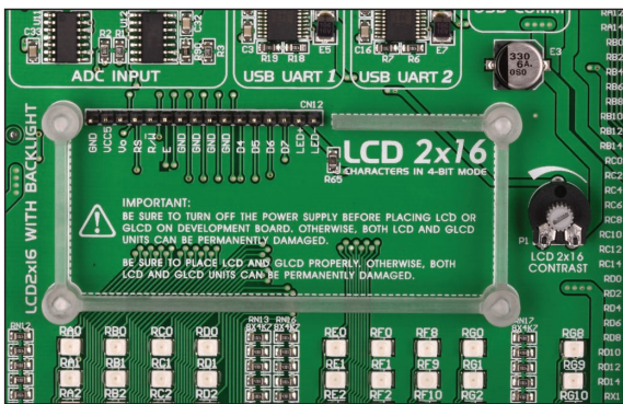
Figure 14-1: Connector for alphanumeric LCD display
