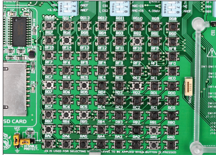
Figure 13-1: Push buttons
