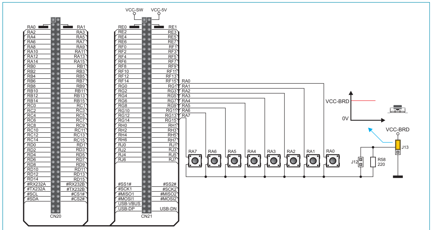
Figure 13-2: Push buttons and port PORT0 connection schematic
