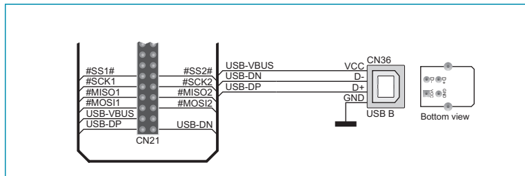
Figure 7-2: USB connector connection schematic
