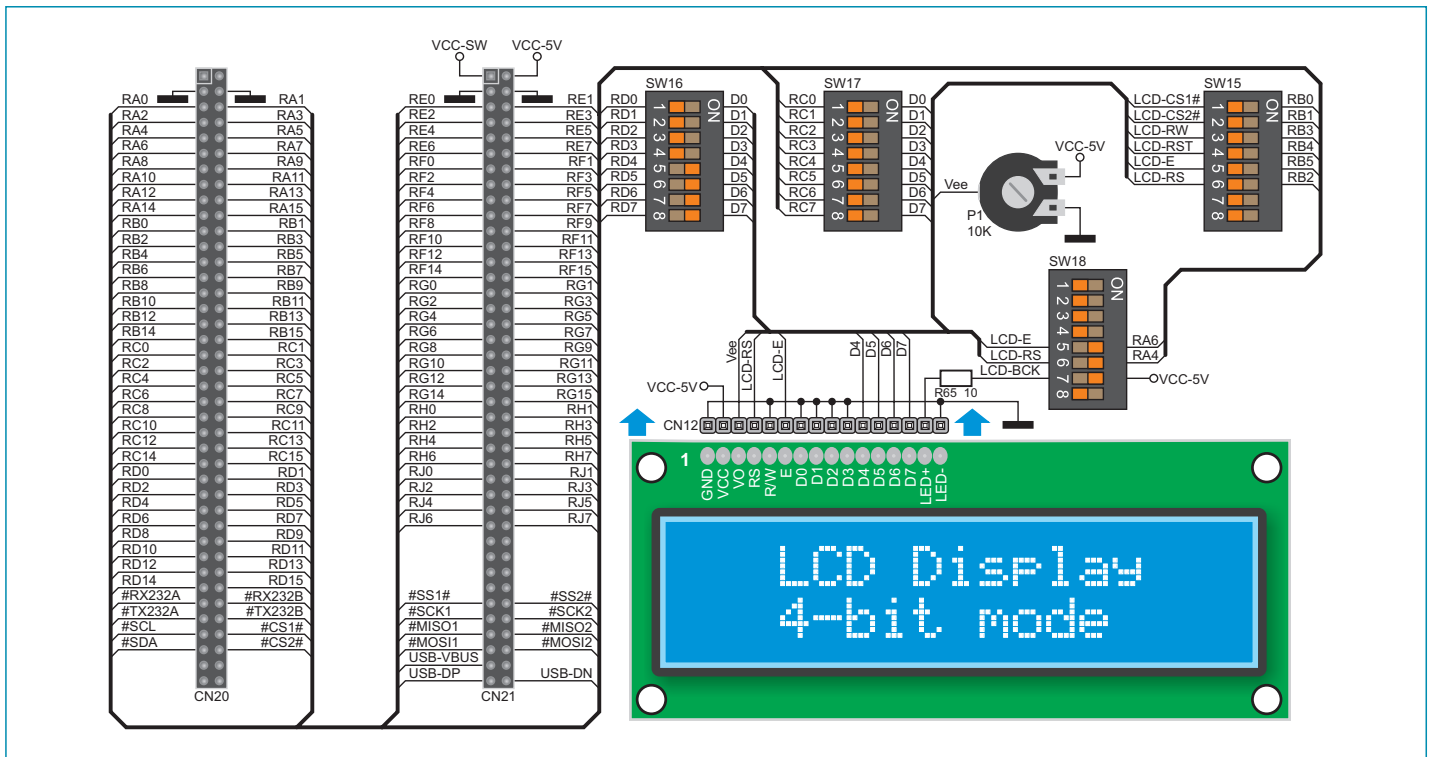
Figure 14-3: 2x16 LCD display connection schematic
