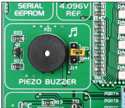
Figure 9-1: Piezo buzzer
