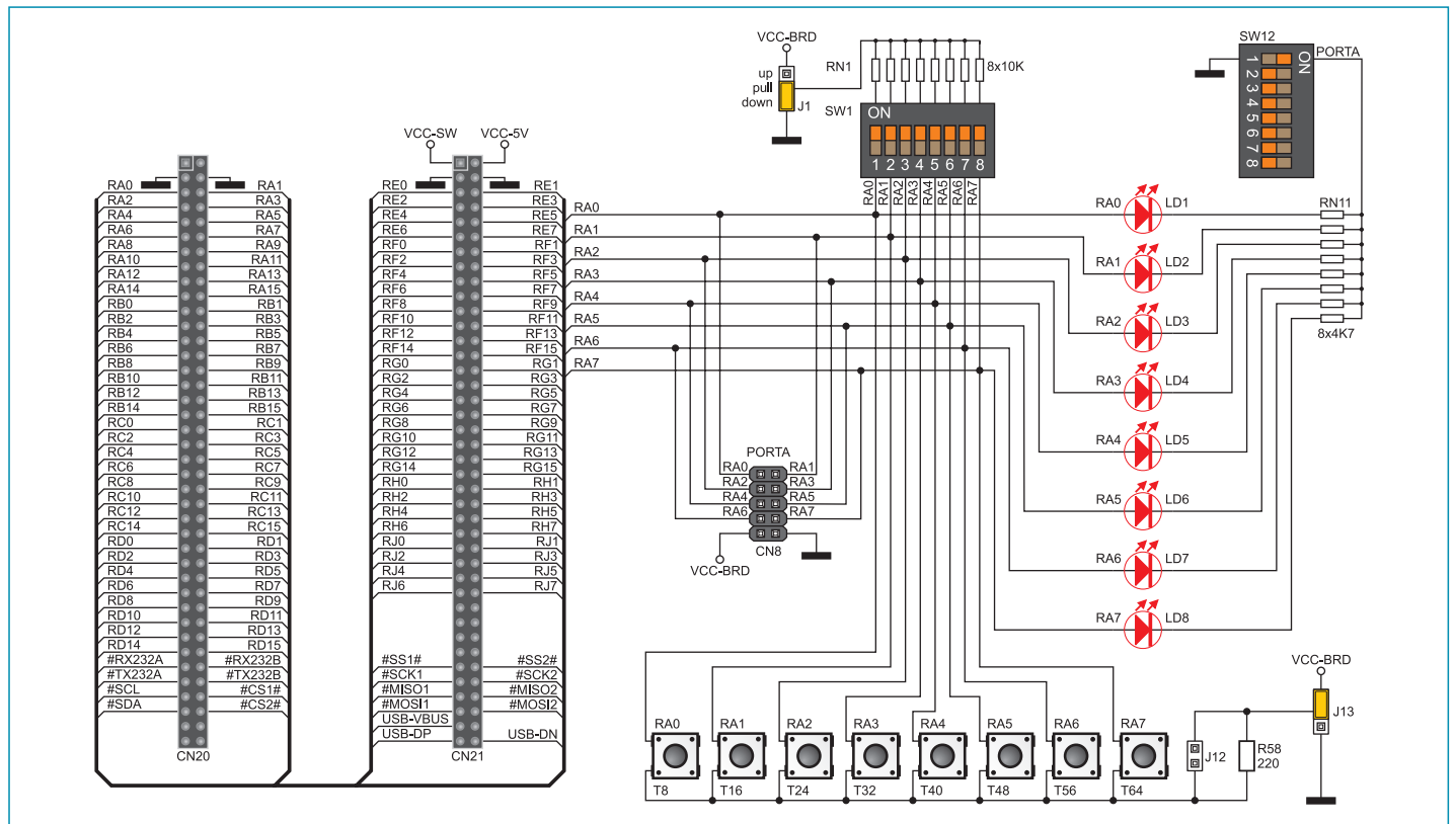
Figure 17-5: Port PORTA connection schematic
