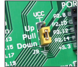
Figure 17-3: J9 in pull-down position
