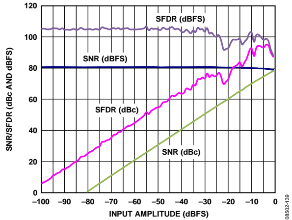
Figure 39. AD9265-125 Single-Tone SNR/SFDR vs. Input Amplitude ( A_{IN} ) with f_{IN} = 2.4 \text{ MHz}
