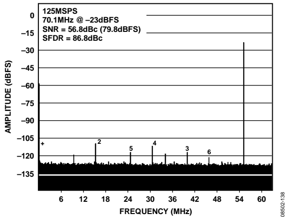
Figure 38. AD9265-125 Single-Tone FFT with f_{IN} = 70.1 \text{ MHz} @ -23 \text{ dBFS} with Dither Enabled, 1M Sample
