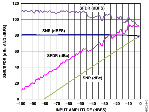
Figure 40. AD9265-125 Single-Tone SNR/SFDR vs. Input Amplitude ( A_{IN} ) with f_{IN} = 98.12 \text{ MHz}
