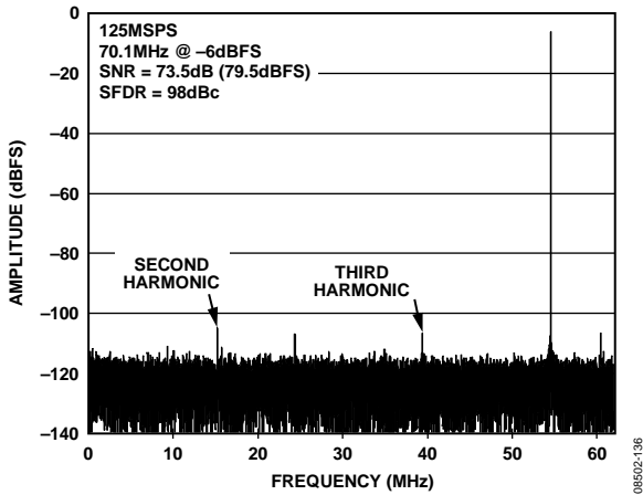
Figure 36. AD9265-125 Single-Tone FFT with f_{IN} = 70.1 \text{ MHz} @ -6 \text{ dBFS} with Dither Enabled
