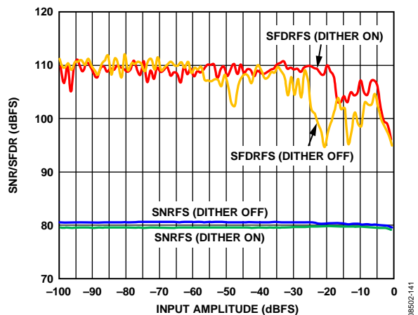
Figure 41. AD9265-125 Single-Tone SNR/SFDR vs. Input Amplitude ( A_{IN} ) with f_{IN} = 30 \text{ MHz} With and Without Dither Enabled
