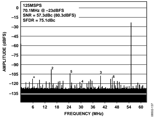
Figure 37. AD9265-125 Single-Tone FFT with f_{IN} = 70.1 \text{ MHz} @ -23 \text{ dBFS} with Dither Disabled, 1M Sample
