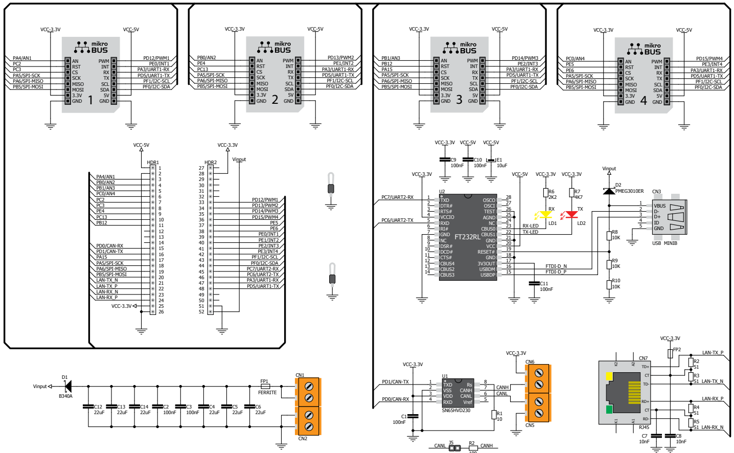
Figure 1-2: mikromedia+ shield schematic
