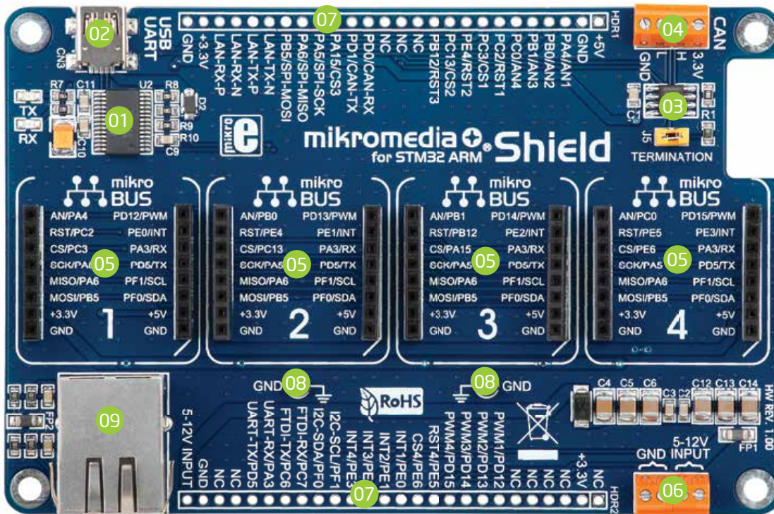
Figure 1-1: mikromedia+ shield
