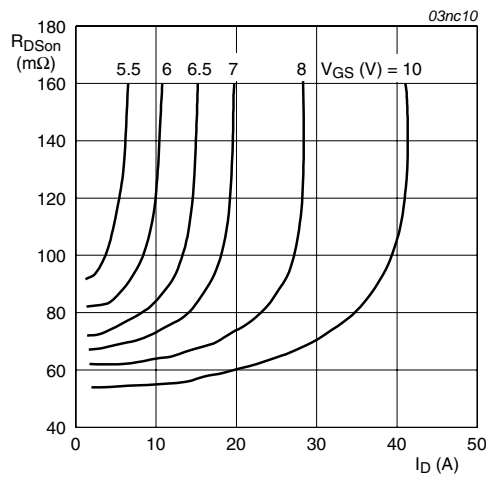
T_j = 25^\circ\text{C}
