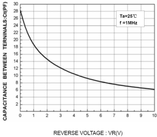
REVERSE VOLTAGE : V_R (V) Figure3.Total Capacitance
