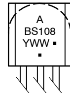
TO-92 CASE 29-11 STYLE 30
