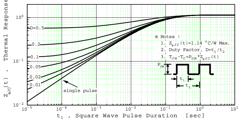
Fig 11. Thermal Response
