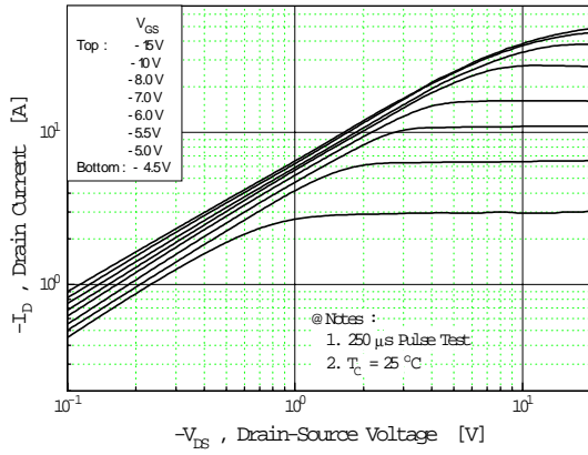
Fig 1. Output Characteristics
