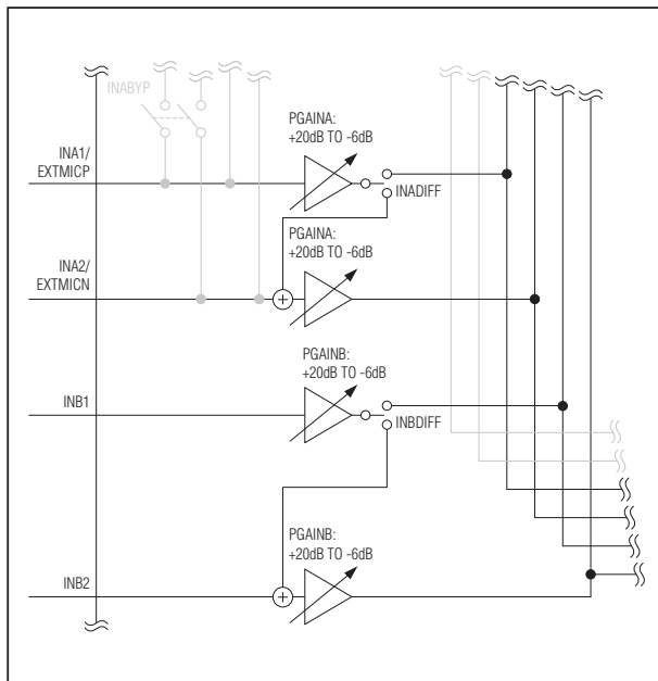
Figure 7. Line Input Block Diagram
