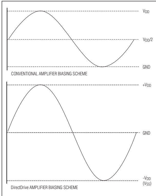
Figure 28. Traditional Amplifier Output vs. DirectDrive Output
