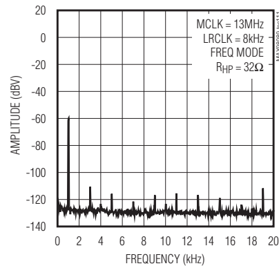
FFT, -60dBFS (DAC TO HEADPHONE)
