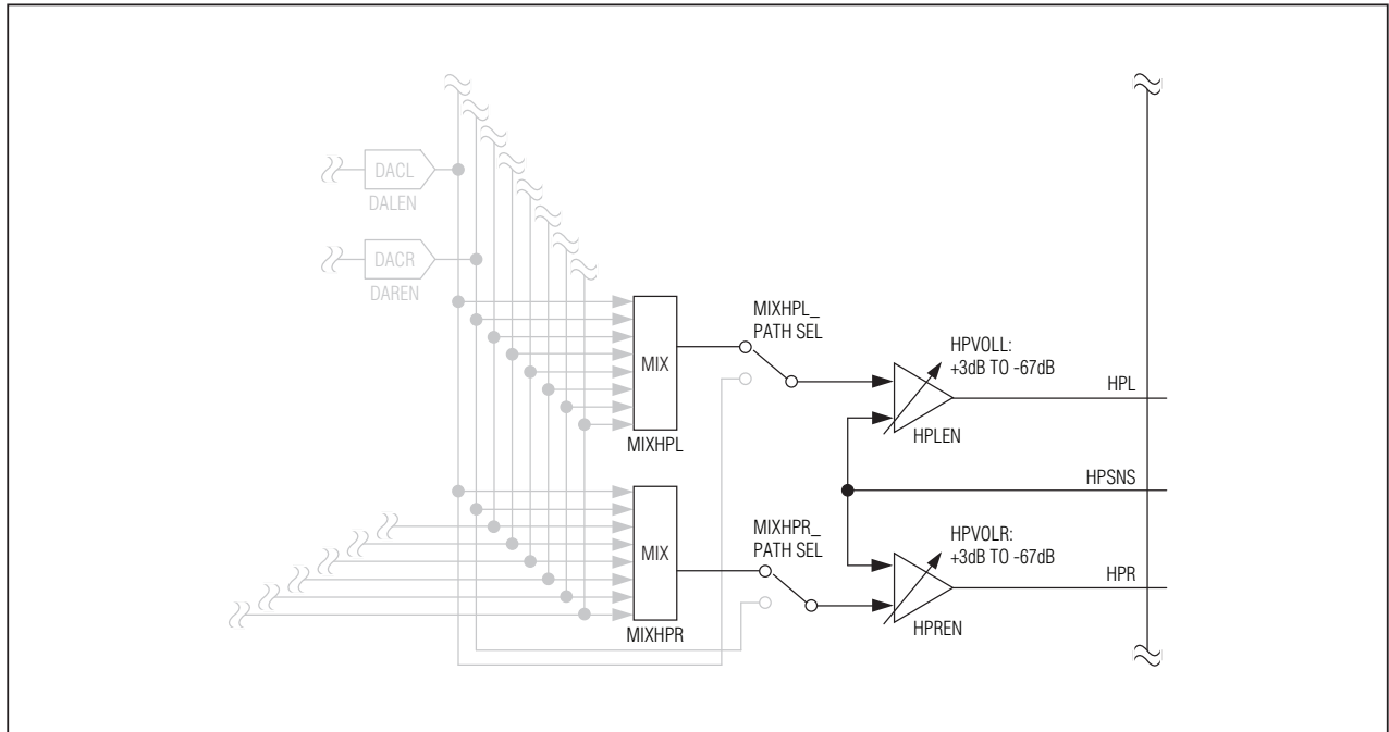
Figure 31. Headphone Amplifier Block Diagram
