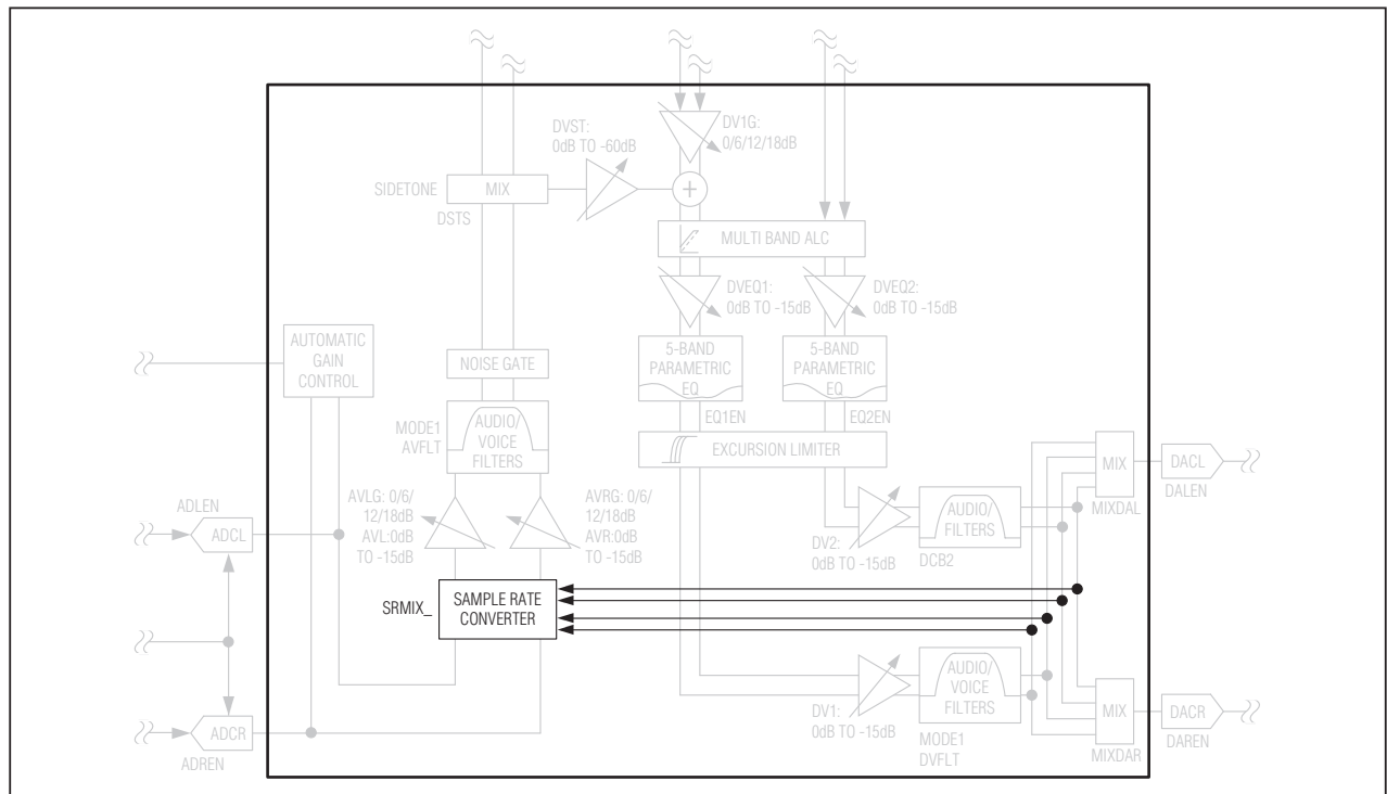
Figure 18. Sample Rate Converter
