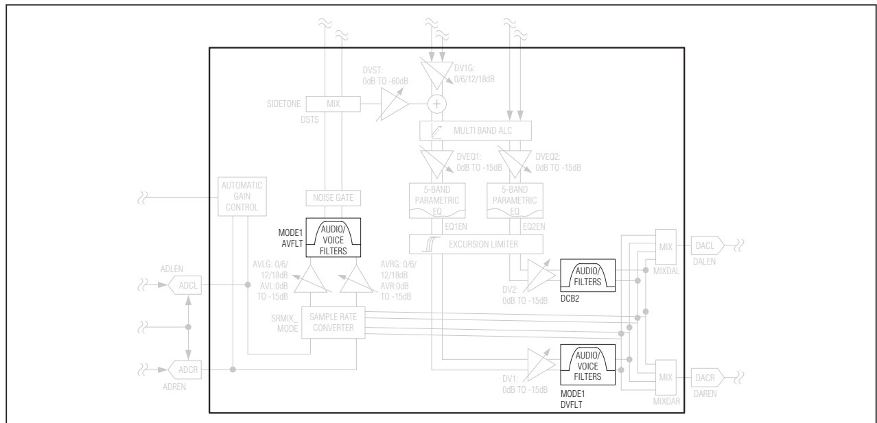
Figure 19. Digital Passband Filtering Block Diagram
