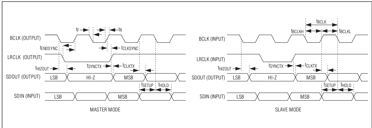
Figure 3. TDM Audio Interface Timing Diagram ( TDM_ = 1, FSW_ = 1 )
