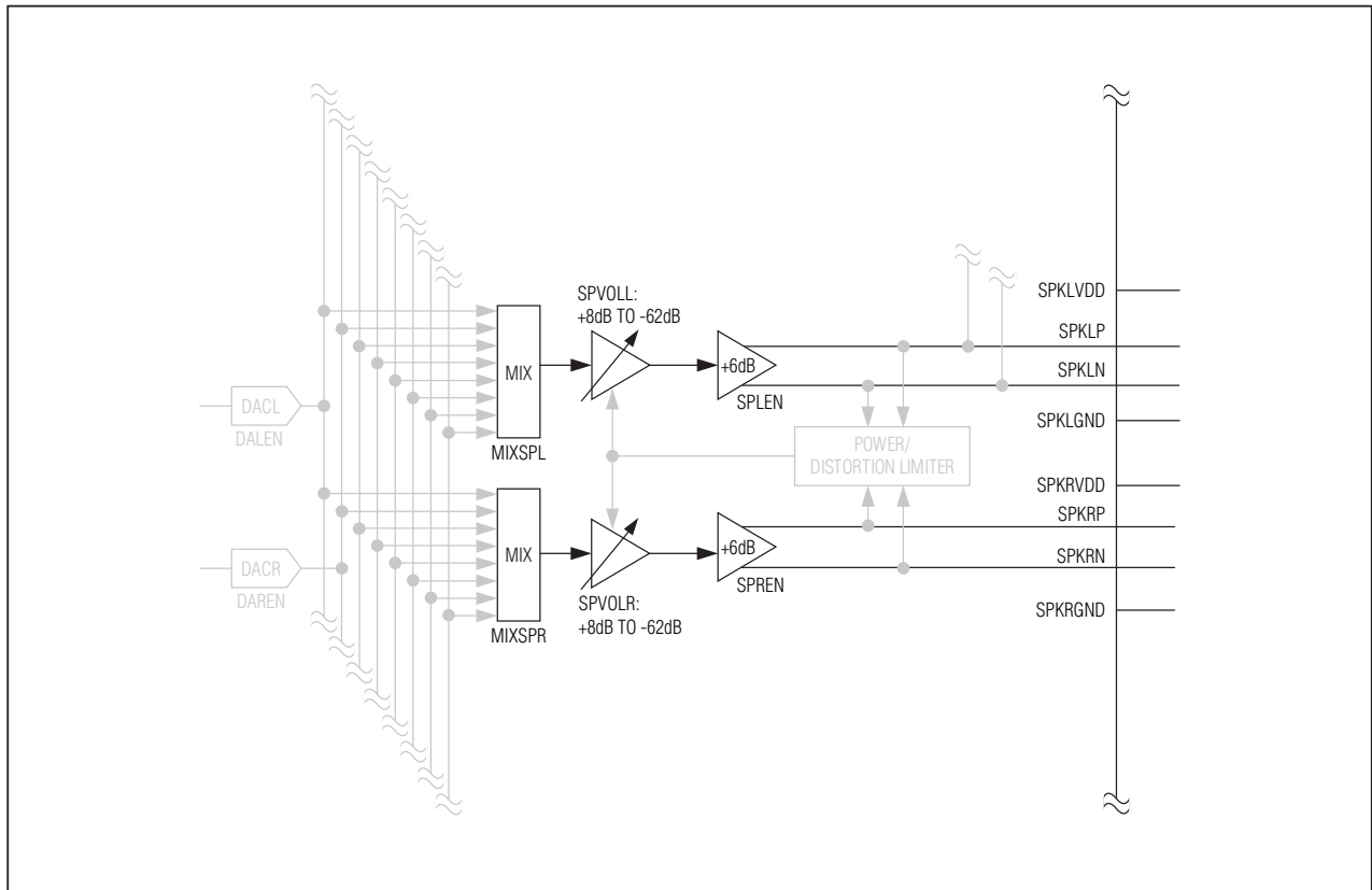
Figure 26. Speaker Amplifier Path Block Diagram
