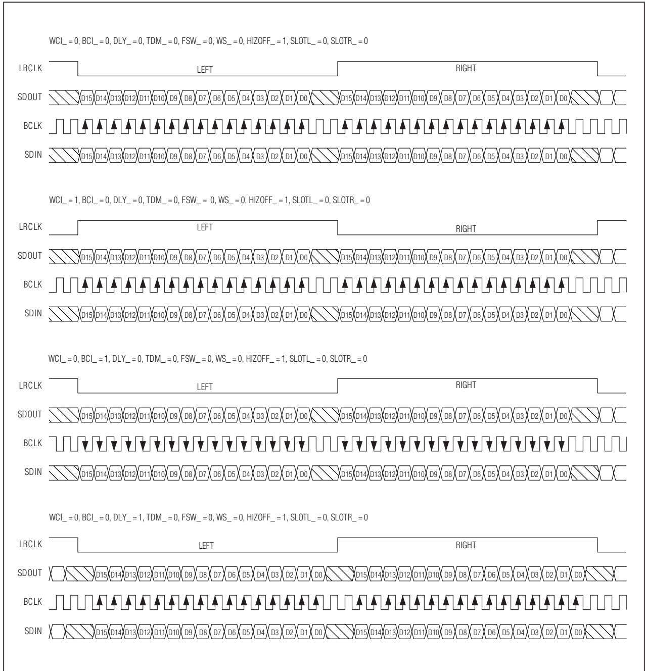
Figure 16. Non-TDM Data Format Examples
