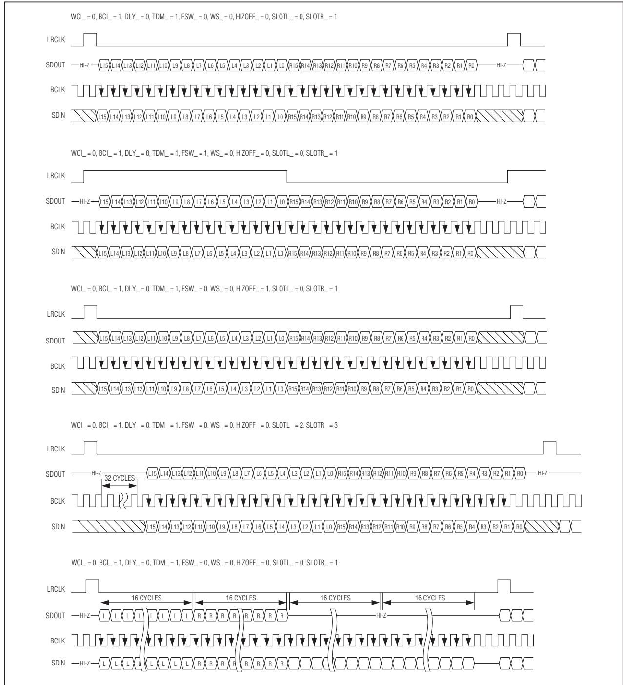
Figure 17. TDM Mode Data Format Examples
