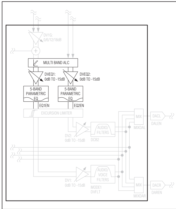
Figure 20. Playback Path Signal Processing Block Diagram
