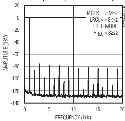
FFT, 0dBFS (DAC TO RECEIVER)
