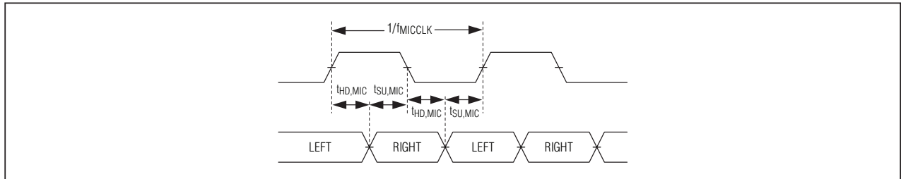
Figure 4. Digital Microphone Timing Diagram
