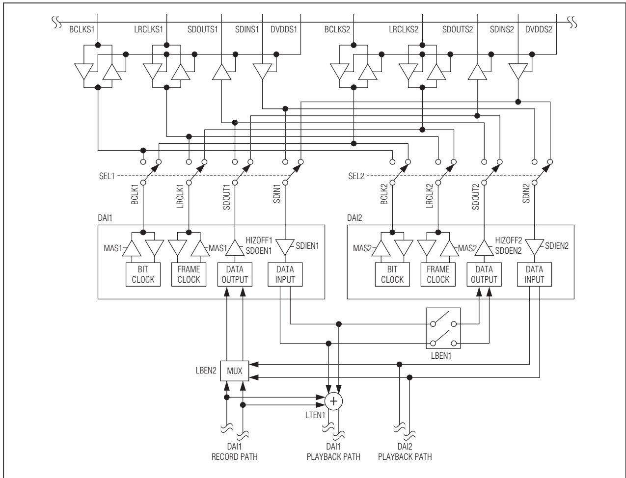
Figure 15. Digital Audio Signal Routing
