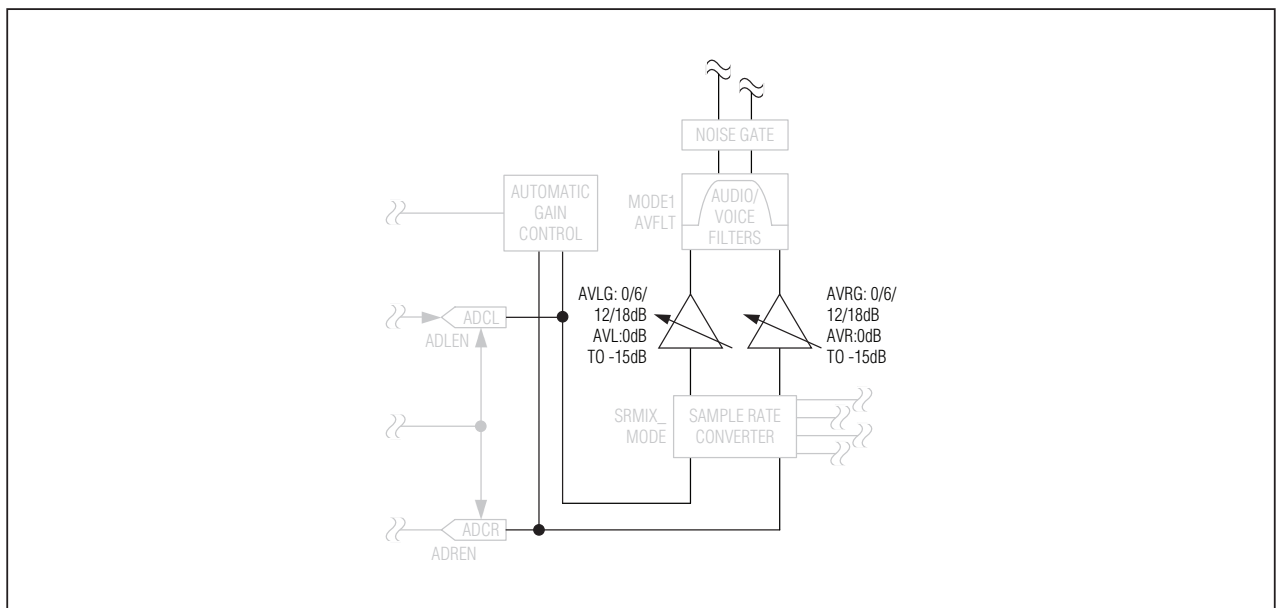
Figure 13. ADC Record Level Control Block Diagram
