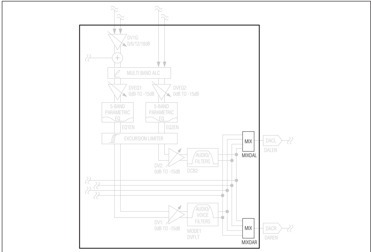
Figure 24. DAC Input Mixer Block Diagram
