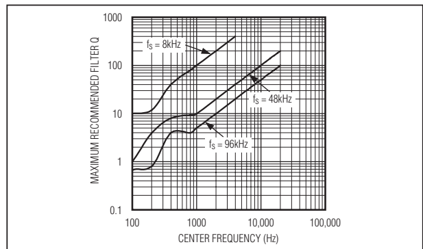
Figure 22. Maximum Recommended Filter Q vs. Frequency
