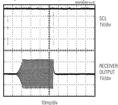
SOFTWARE TURN-ON/OFF RESPONSE (DAC TO RECEIVER, V_{SEN} = 1 )
