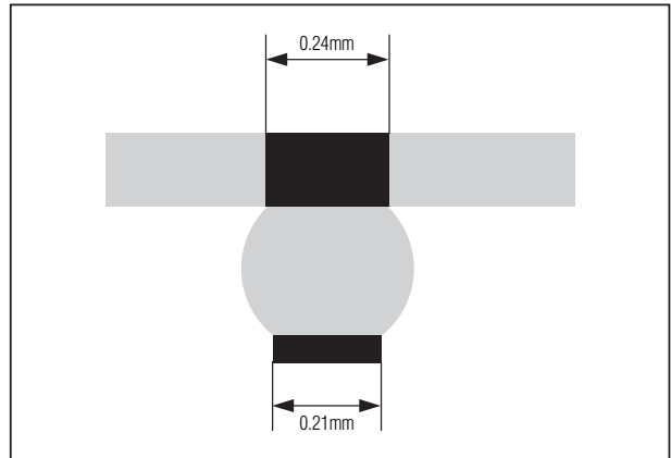
Figure 44. MAX98089EWY WLP Ball Dimensions
