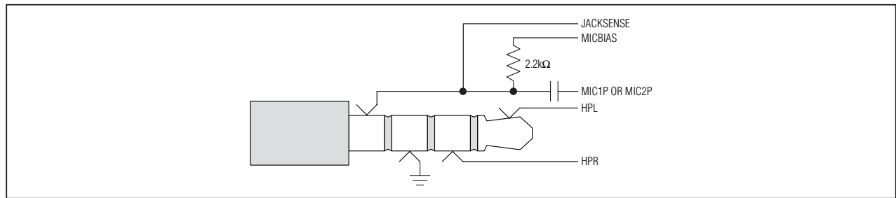
Figure 33. Typical Configuration for Jack Detection
