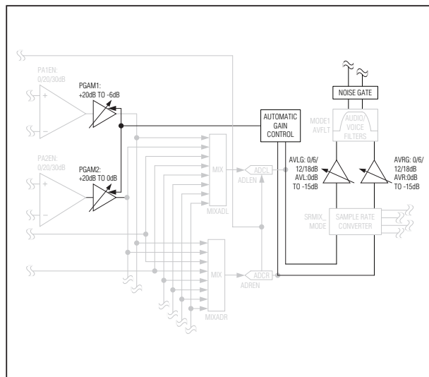
Figure 10. Record Path Signal Processing Block Diagram
