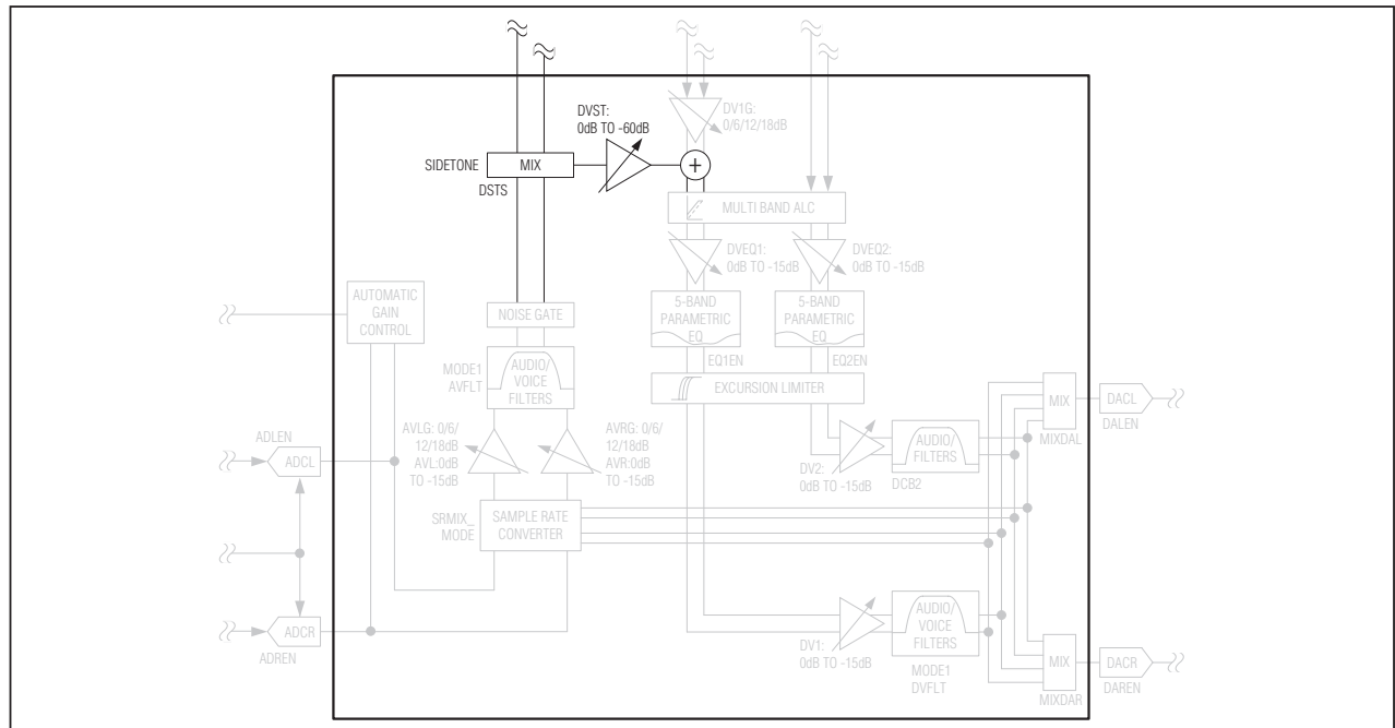
Figure 14. Sidetone Block Diagram
