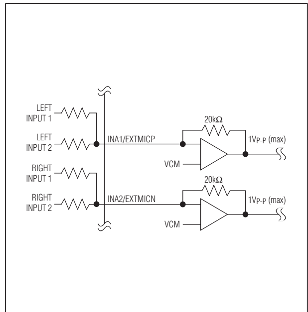
Figure 8. Summing Multiple Input Signals into INA/INB
