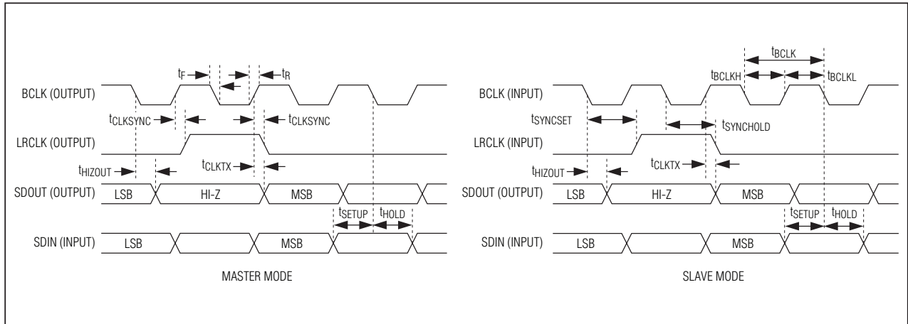
Figure 2. TDM Audio Interface Timing Diagram ( TDM_ = 1, FSW_ = 0 )
