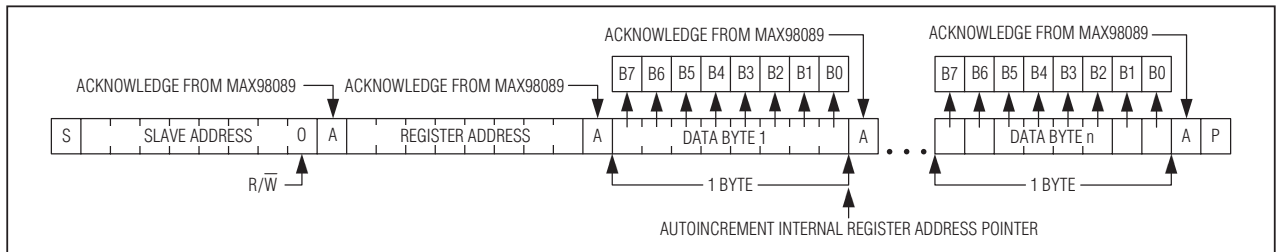
Figure 37. Writing n-Bytes of Data to the ICs
