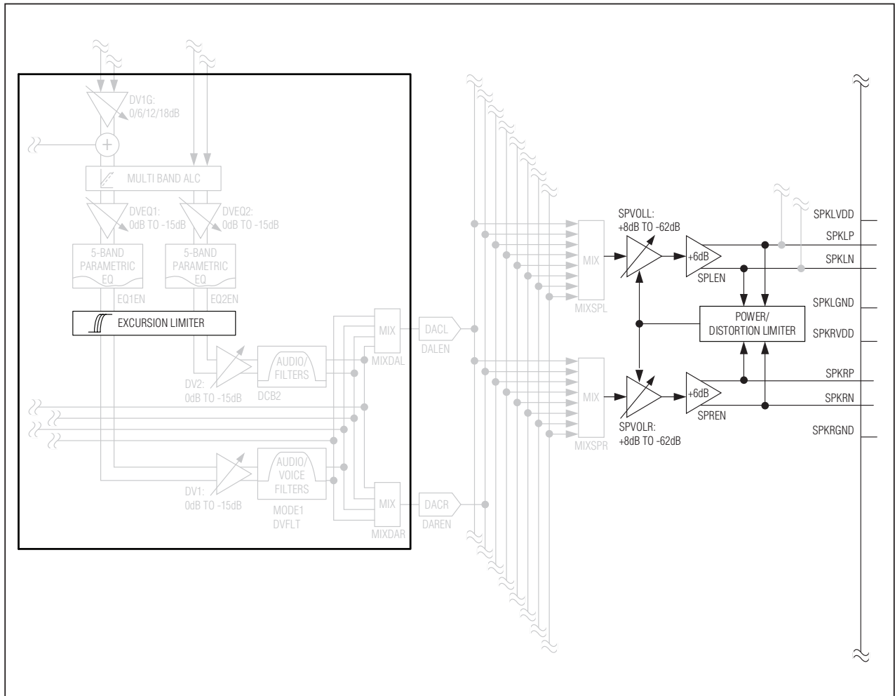
Figure 27. Speaker Amplifier Signal Processing Block Diagram
