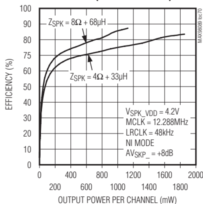
EFFICIENCY vs. OUTPUT POWER (DAC TO SPEAKER)
