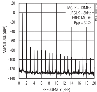
FFT, 0dBFS (DAC TO HEADPHONE)
