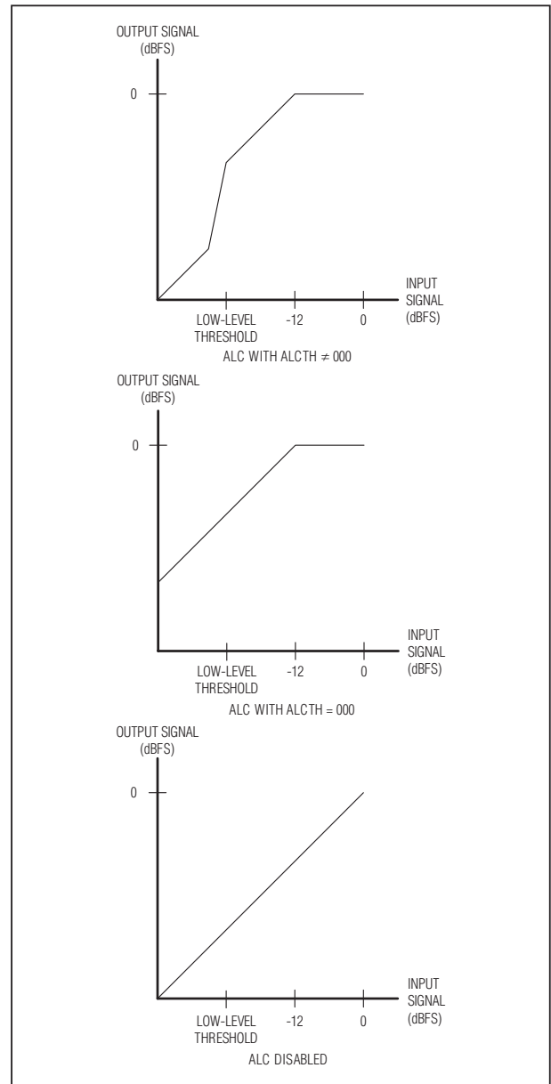
Figure 21. ALC Input vs. Output Examples
