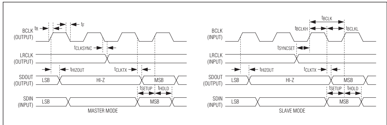
Figure 1. Non-TDM Audio Interface Timing Diagrams (TDM 0 = 0)
