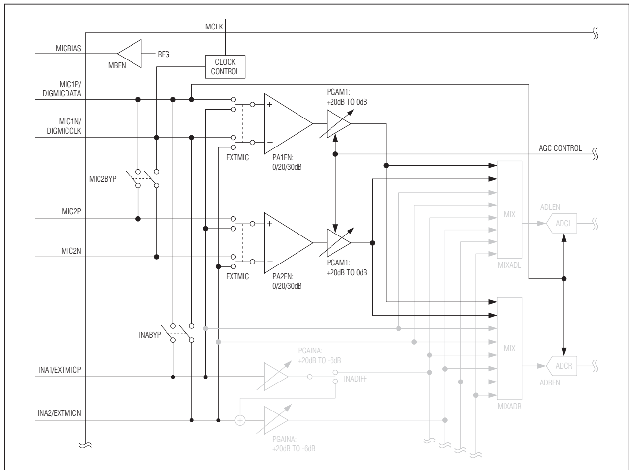
Figure 6. Microphone Input Block Diagram
