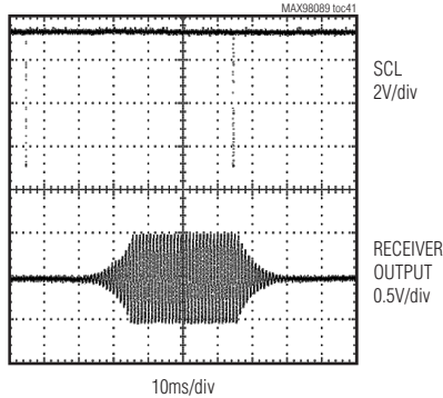
SOFTWARE TURN-ON/OFF RESPONSE (DAC TO RECEIVER, V_{SEN} = 0 )
