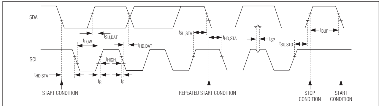
Figure 5. I 2 C Interface Timing Diagram
