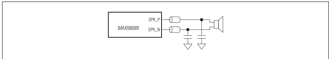
Figure 42. Optional Class D Ferrite Bead Filter
