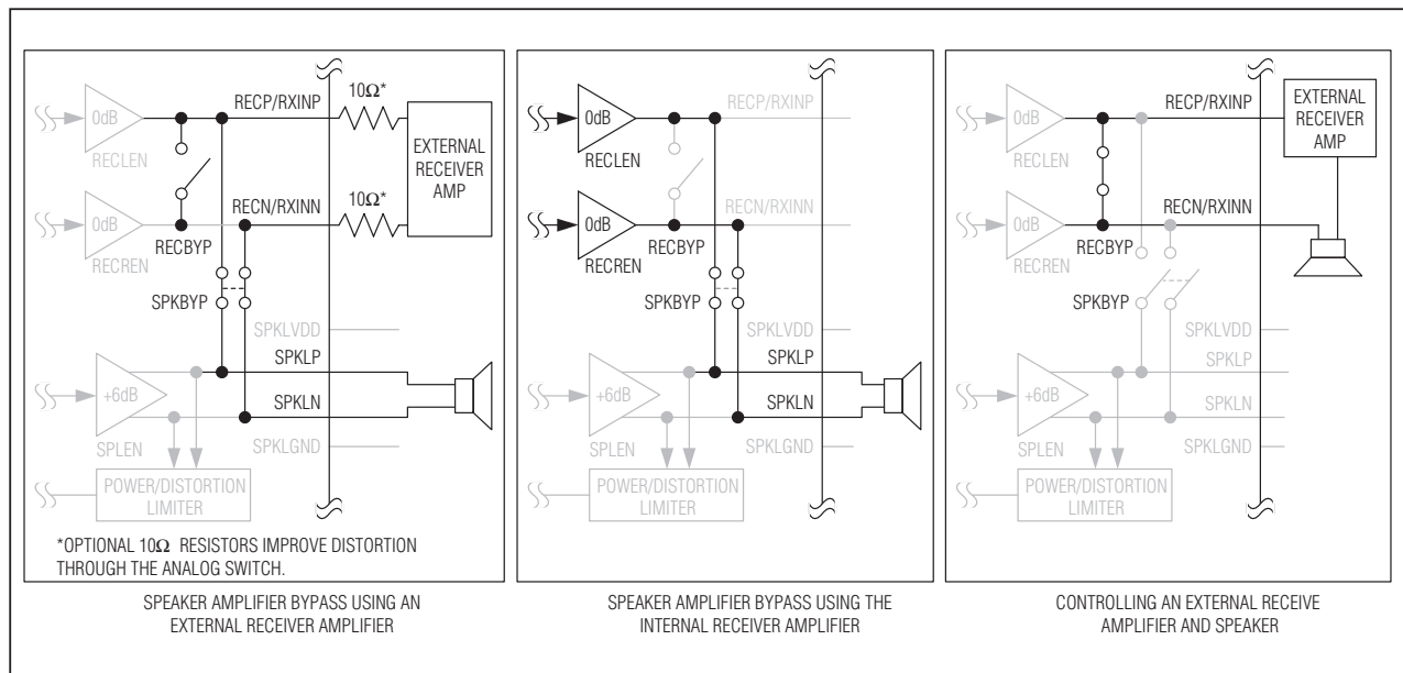
Figure 32. Output Bypass Switch Block Diagrams
