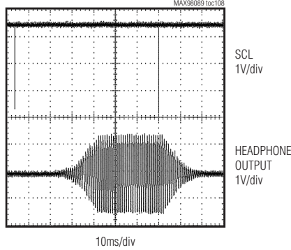
SOFTWARE TURN-ON/OFF RESPONSE (DAC TO HEADPHONE, V_{SEN} = 0 )
