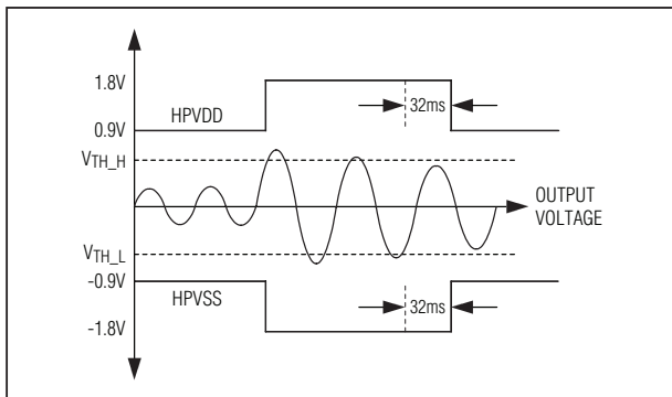
Figure 29. Class H Operation
