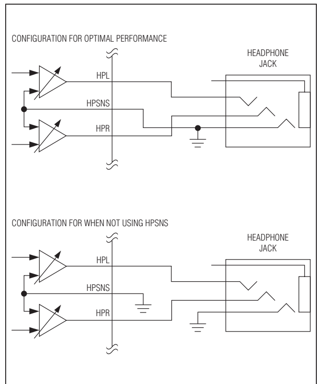
Figure 30. HPSNS configurations
