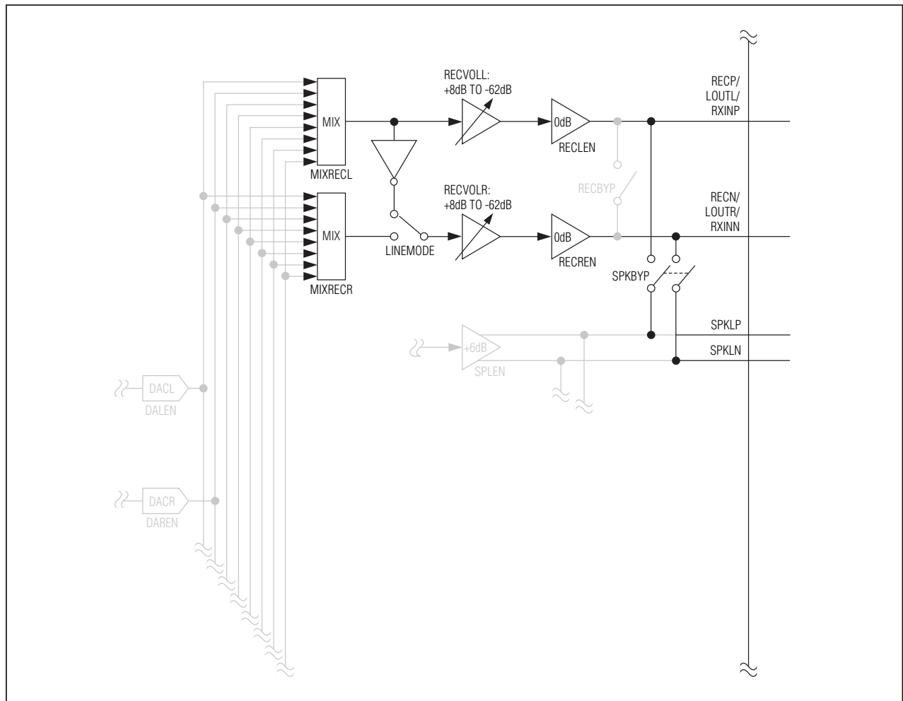
Figure 25. Receiver Amplifier Block Diagram
