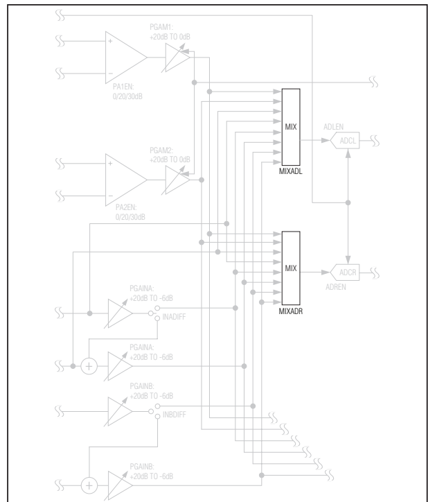
Figure 9. ADC Input Mixer Block Diagram
