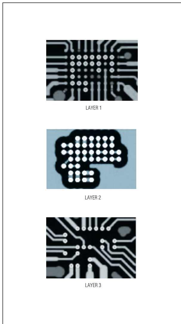
Figure 43. Suggested Routing for the MAX98089EWY
