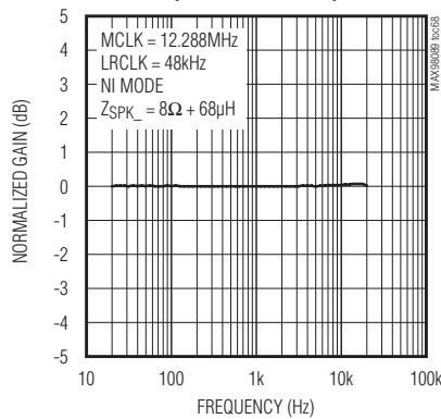
GAIN vs. FREQUENCY (DAC TO SPEAKER)
