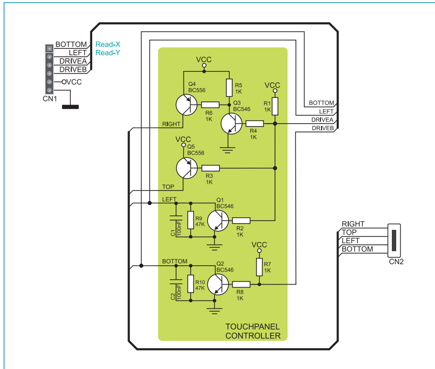
Figure 2: TouchPanel Controller PROTO additional board connection schematic
