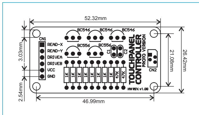
Figure 3: Dimensions of the TouchPanel Controller PROTO board
