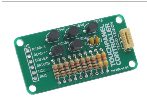
Figure 1: TouchPanel Controller PROTO additional board
