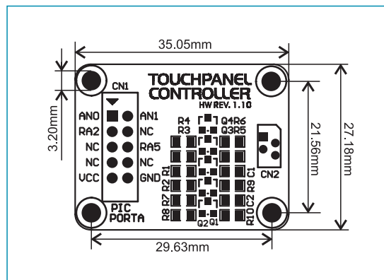
Figure 3: Dimensions of the additional board
