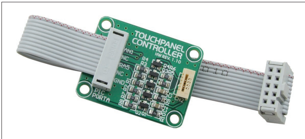
Figure 1: TouchPanel Controller additional board
