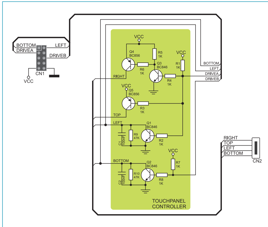
Figure 2: TouchPanel Controller board connection schematic
