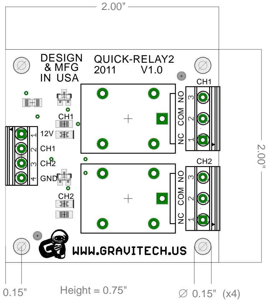
QUICK-RELAY2 MECHANICAL DIMENSIONS
