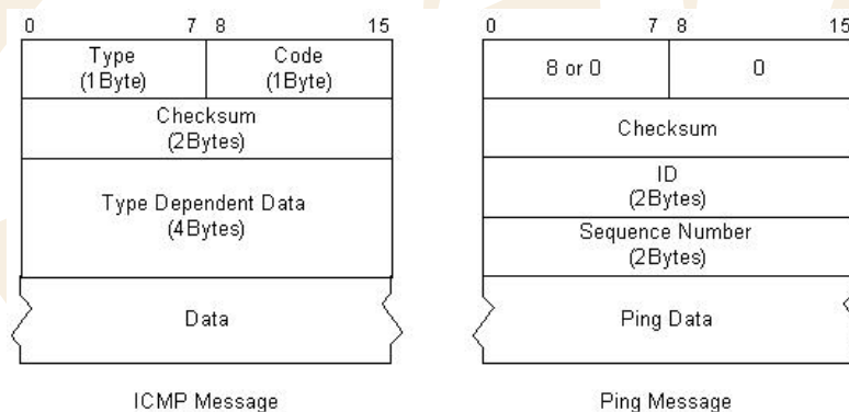
<Fig 3.10: ICMP Message VS Ping Message>
