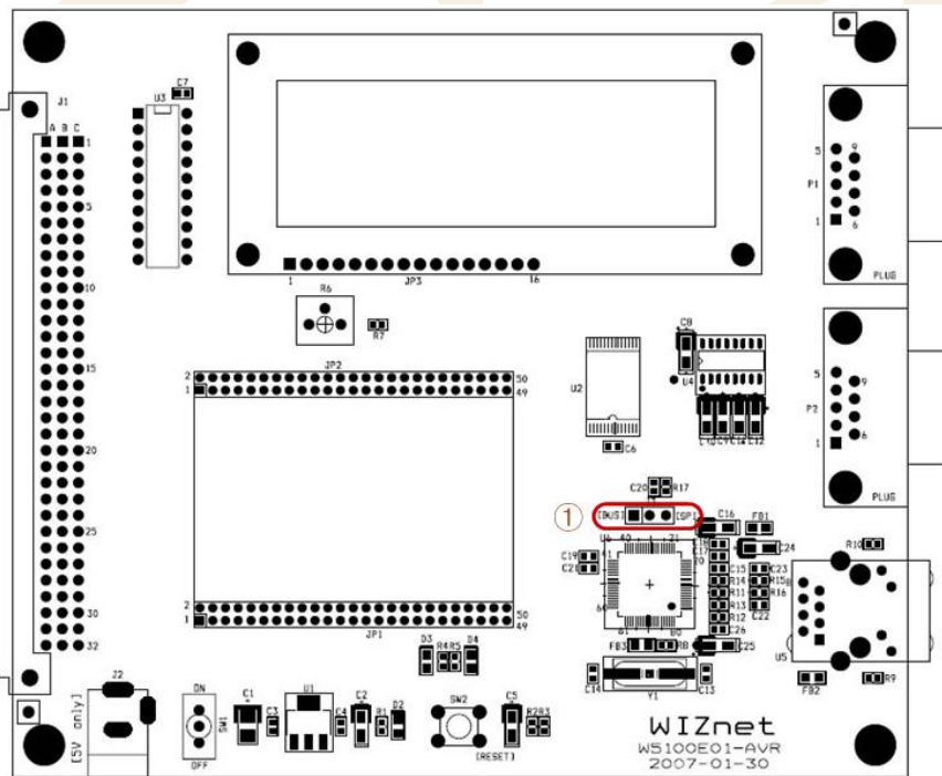
<Fig 2.1 : EVB B/D Jumper Setting>
