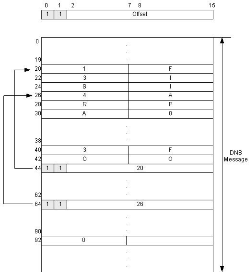
<Fig 3.45: DNS Message Compression Scheme>
