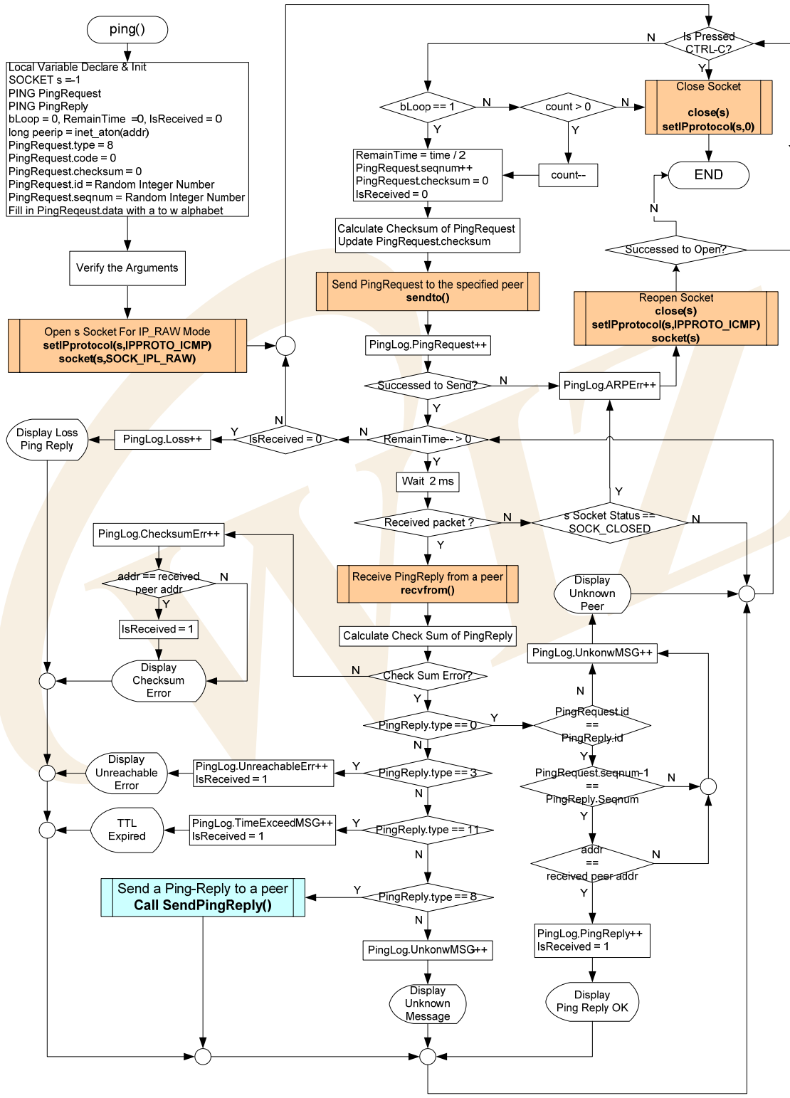
<Fig 3.11: ping(>
