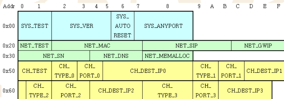
<Fig 3.2: AVR Internal EEPROM Map>
