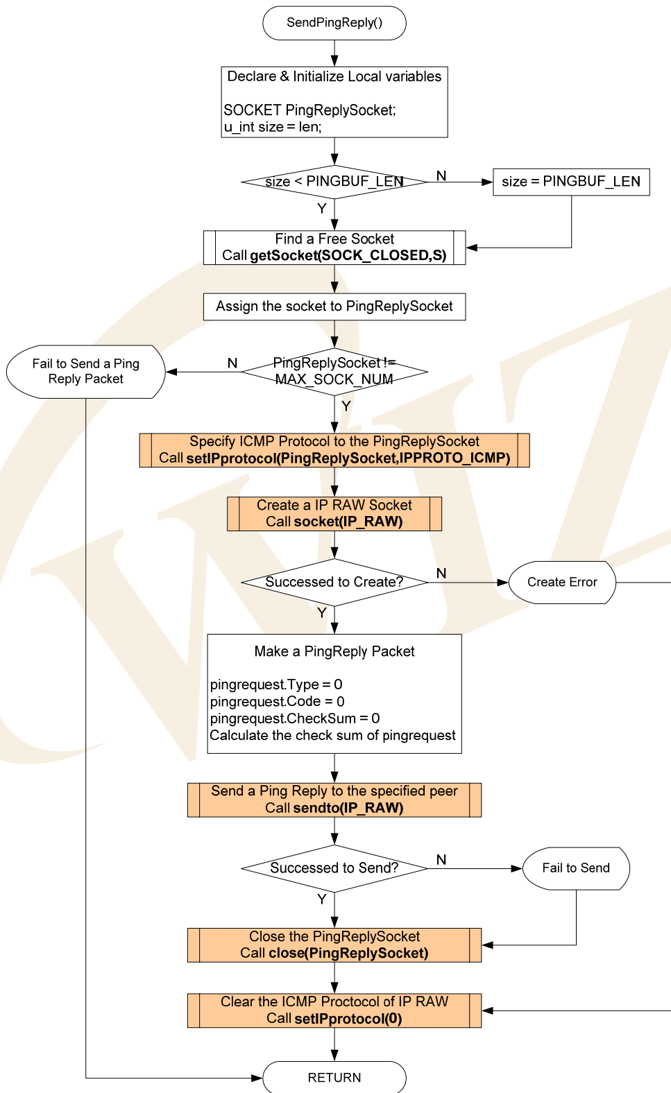
<Fig 3.13: SendPingReply()>
