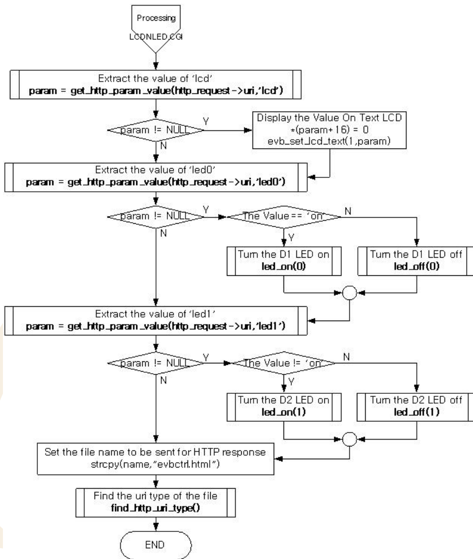
<Fig 3.24: LCDNLED.CGI Processing>
