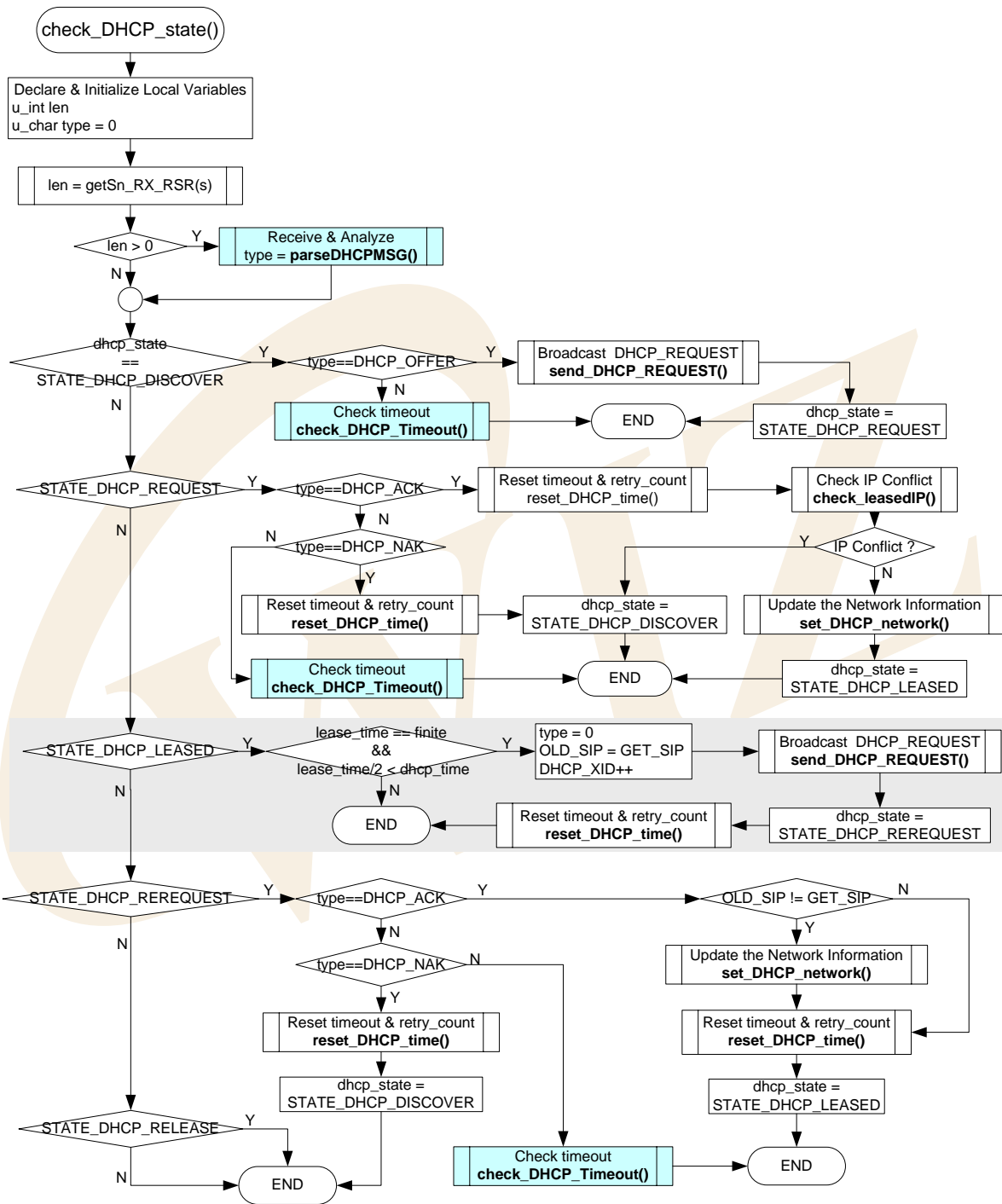
<Fig 3.31: check_DHCP_state(>
