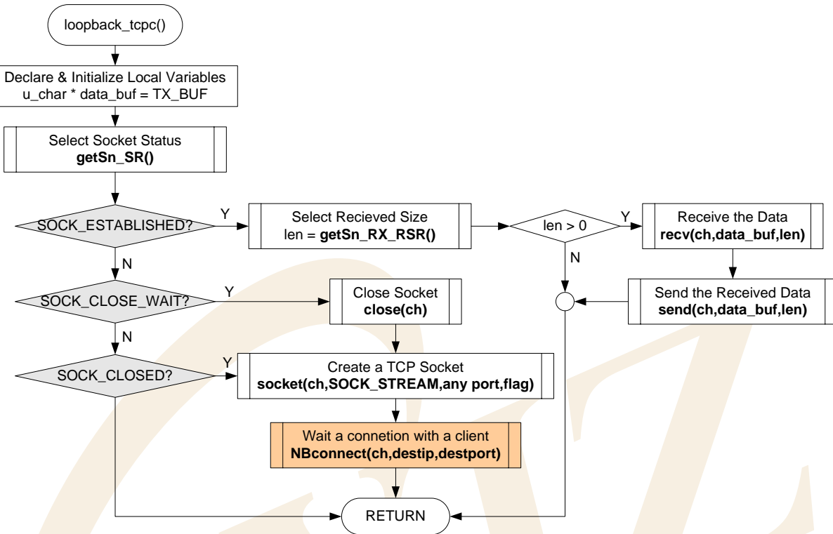
<Fig 3.15: loopback_tcpclient()>
