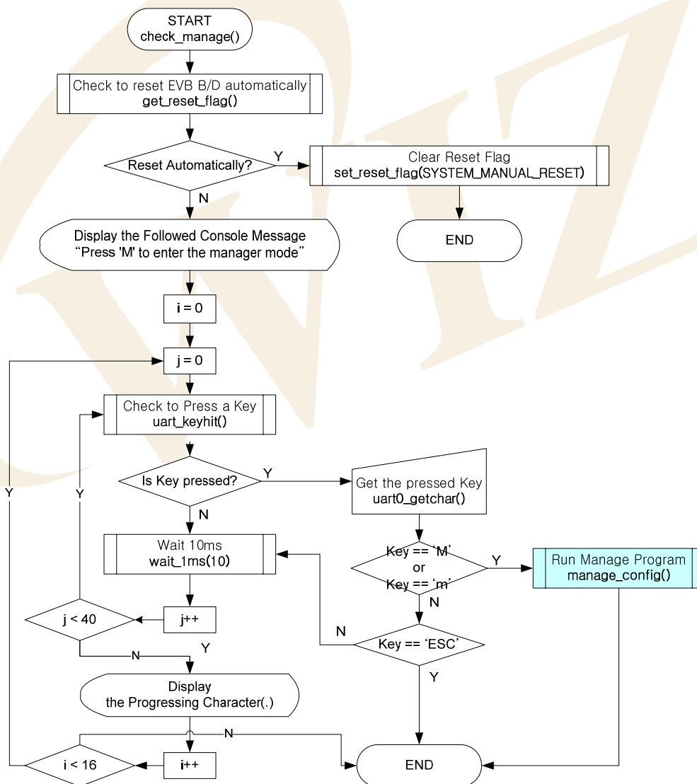
<Fig 3.4: check_manage()>
