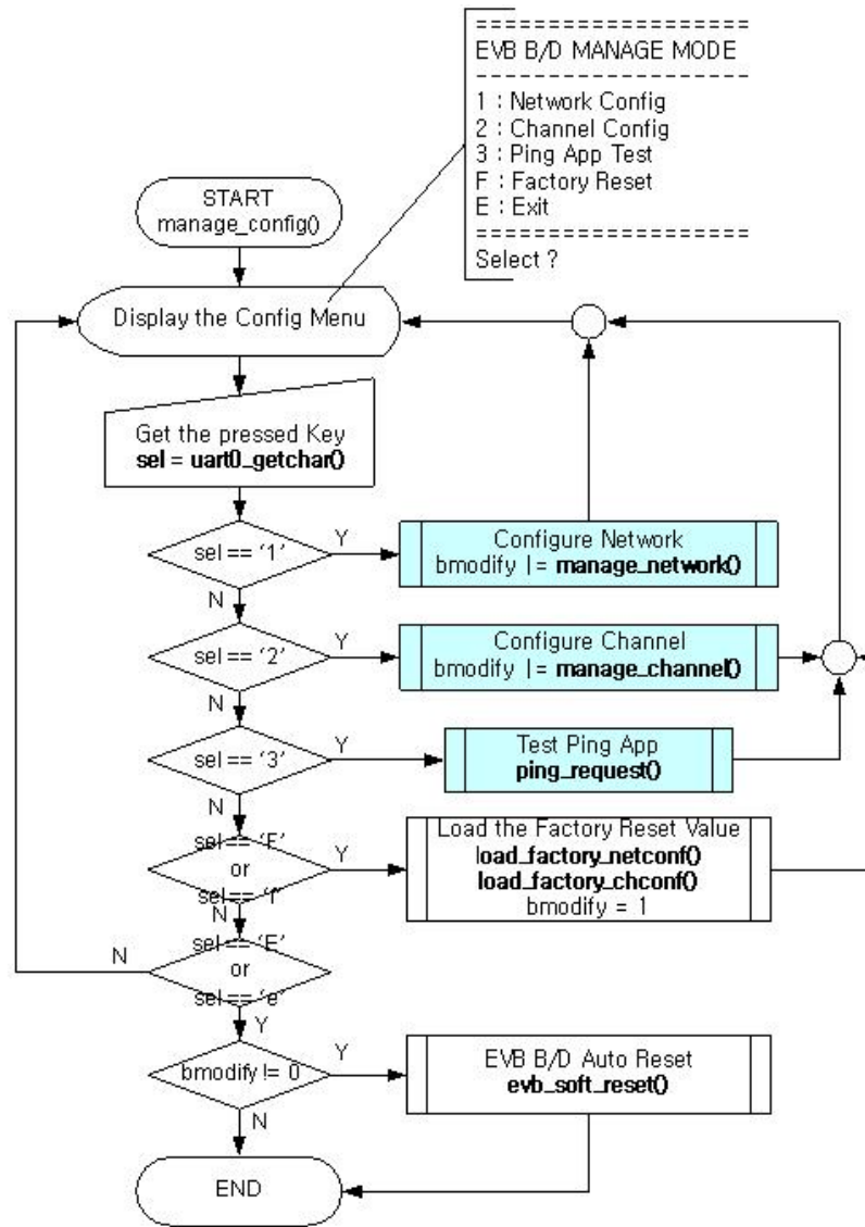
<Fig 3.5: manage_config(>
