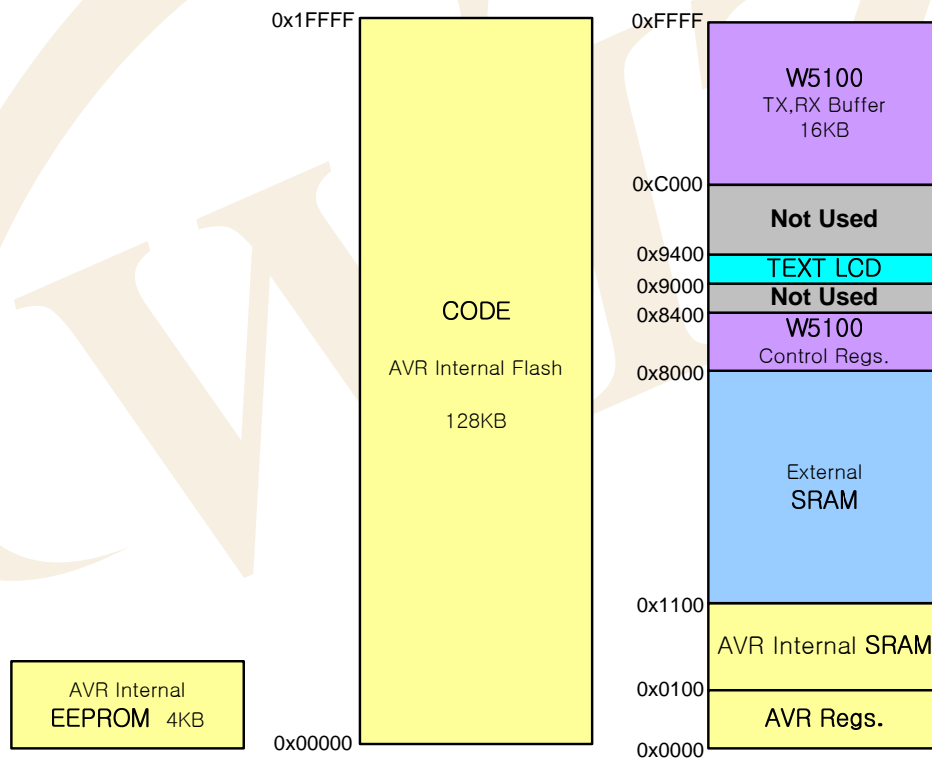
<Fig 3.1: EVB B/D Memory Map>
