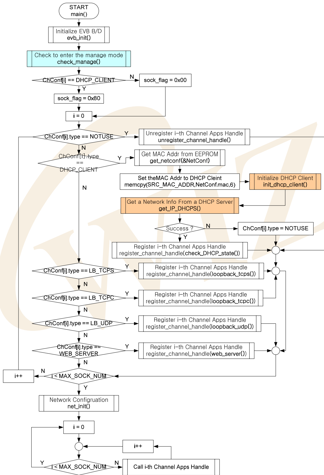
<Fig 3.3: EVB B/D's main()>
