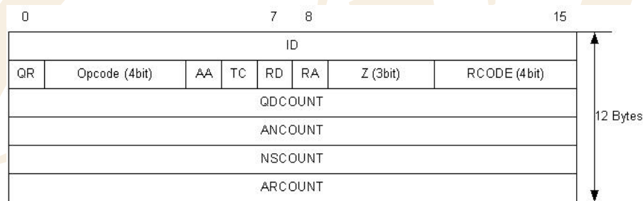
<Fig 3.35: Header Section Format>
