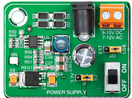
Figure 3-1: Dual power supply unit of EasyAVR™ v7
