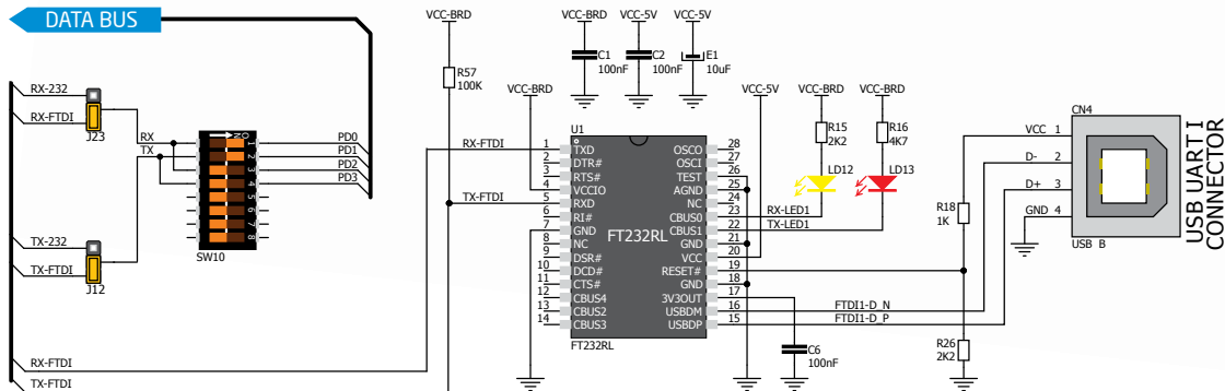
Figure 7-1: USB-UART connection schematic
