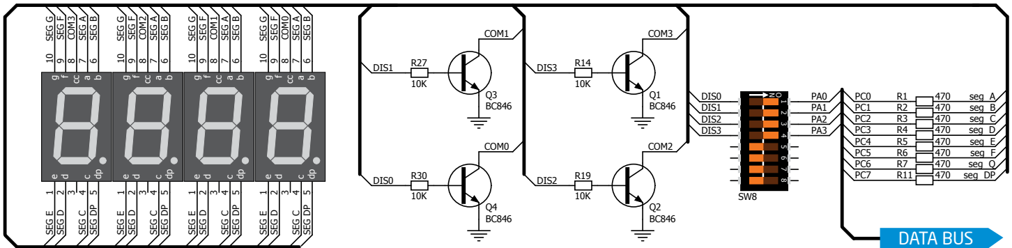
Figure 13-2: 4-digit 7-segment display schematic
