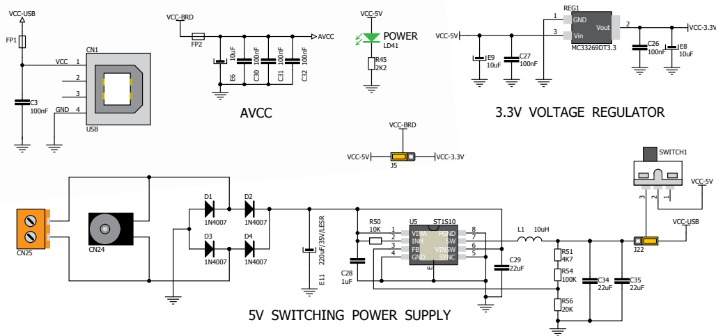
Figure 3-2: Dual power supply unit schematic
