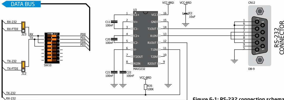
Figure 6-1: RS-232 connection schematic
