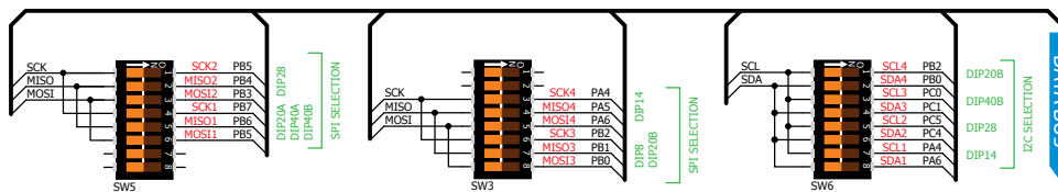
Figure 8-1: mikroBUS™ socket with DIP switches schematic
