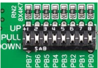
Figure 9-2: Tri-state DIP switch on PORTB
