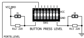
Figure 9-2: Tri-state DIP switch on PORTB
