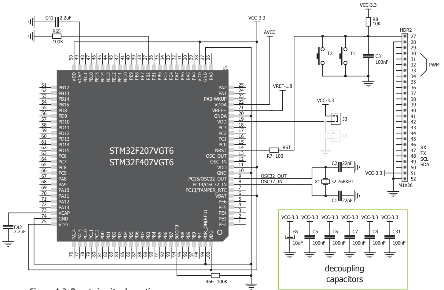
Figure 4-3: Reset circuit schematics
